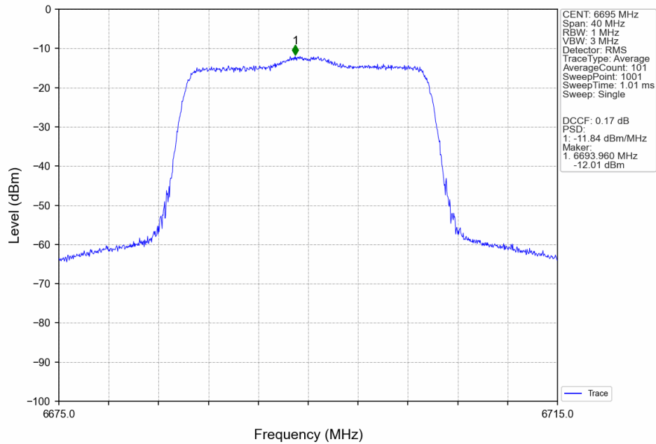
802.11ax(HEW20)_MCH_6695MHz_SU_/_MIMO_NTNV
