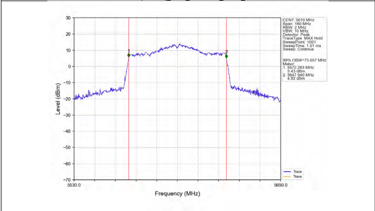
802.11ac(VHT80)_HCH_5610MHz_ANT3_NTNV
