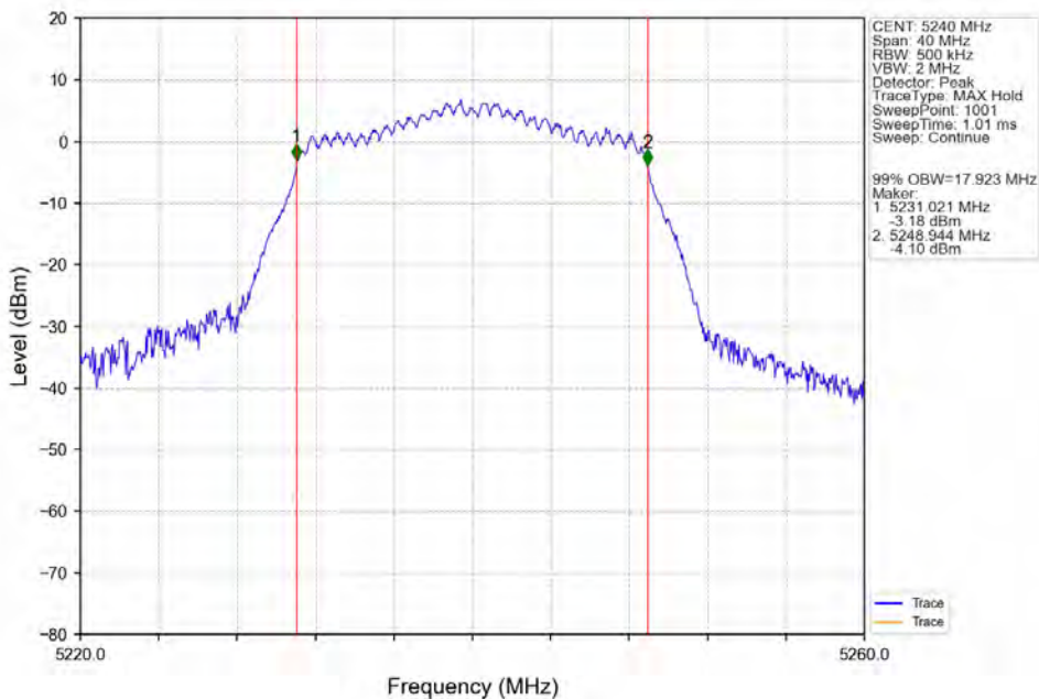
802.11n(HT20)_HCH_5240MHz_ANT3_NTNV
