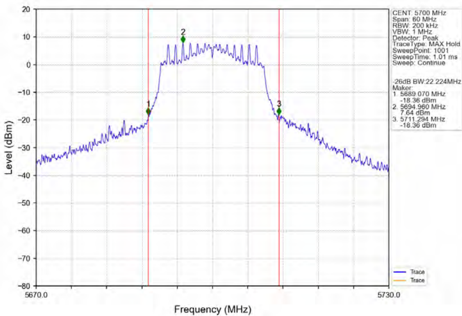
802.11n(HT20)_HCH_5700MHz_ANT3_NTNV
