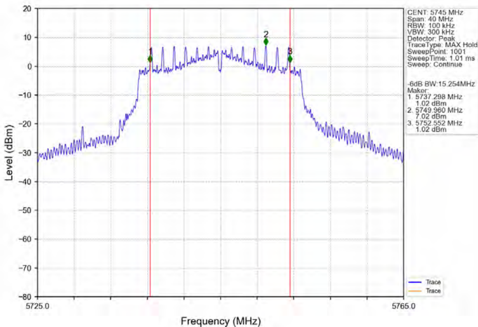
802.11n(HT20)_LCH_5745MHz_ANT3_NTNV
