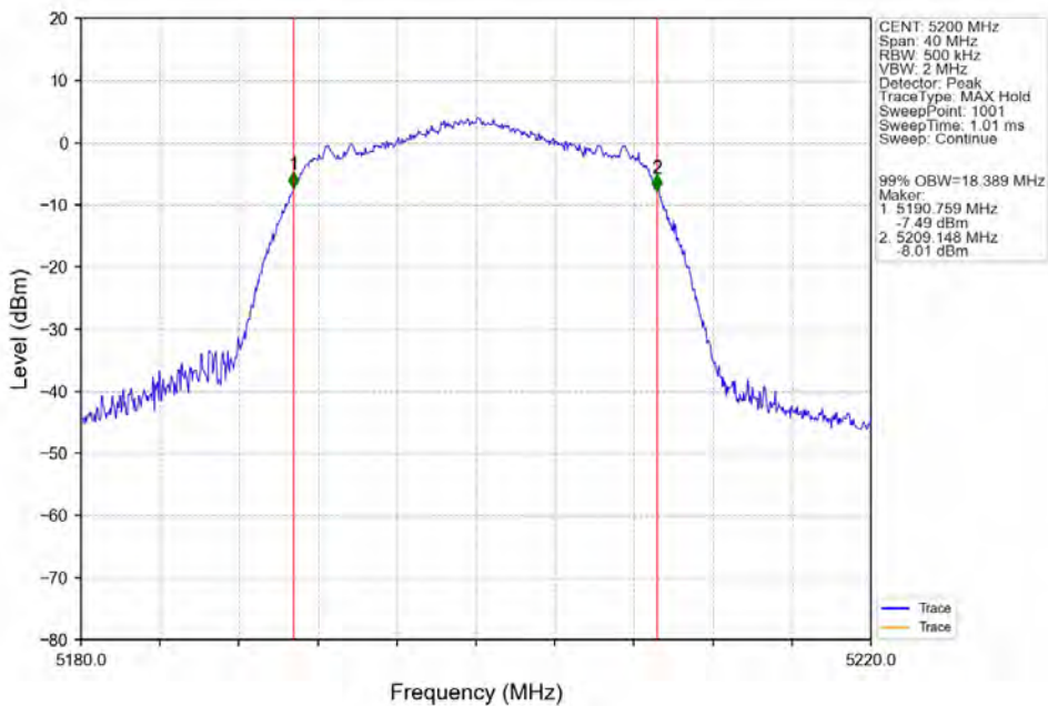
802.11ax(HEW20)_MCH_5200MHz_SU_/_ANT3_NTNV
