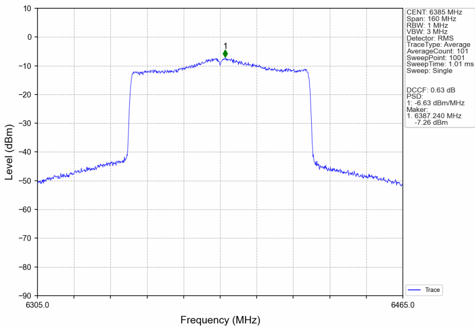
802.11ax(HEW80)_HCH_6385MHz_SU_/_ANT3_NTNV
