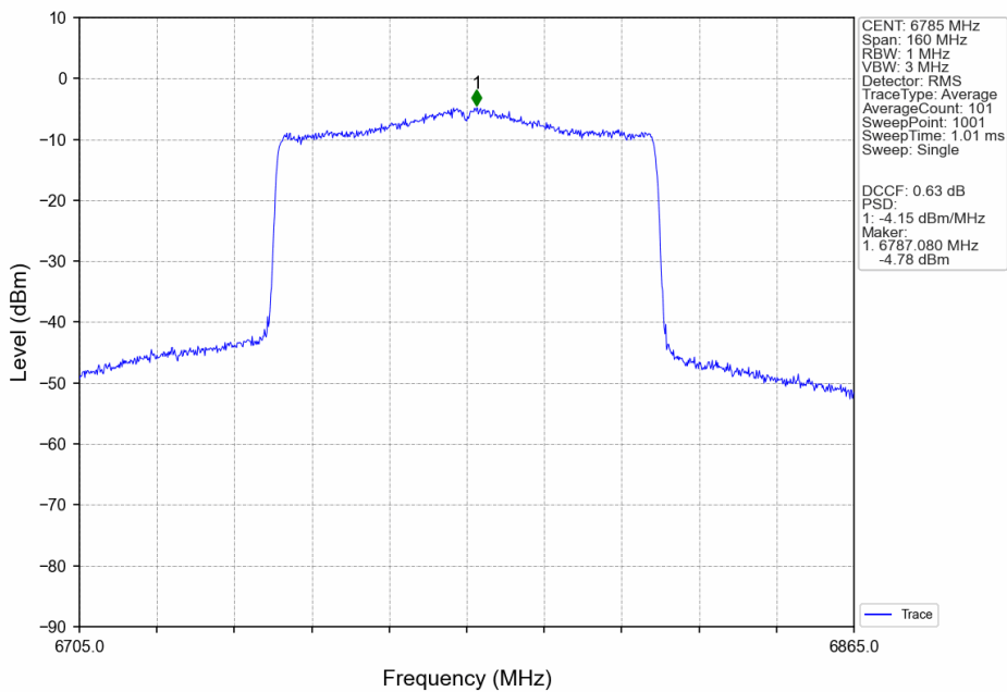
802.11ax(HEW80)_HCH_6785MHz_SU_/_ANT3_NTNV
