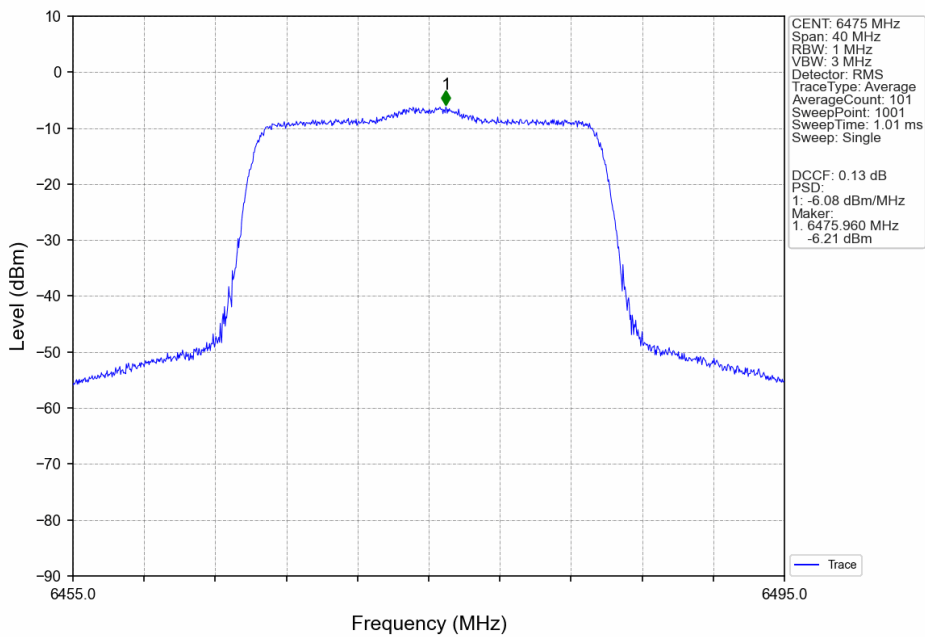
802.11ax(HEW20)_MCH_6475MHz_SU / _ANT2_NTNV
