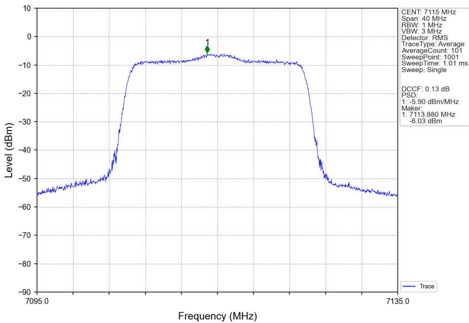
802.11ax(HEW20)_HCH_7115MHz_SU_/_ANT3_NTNV
