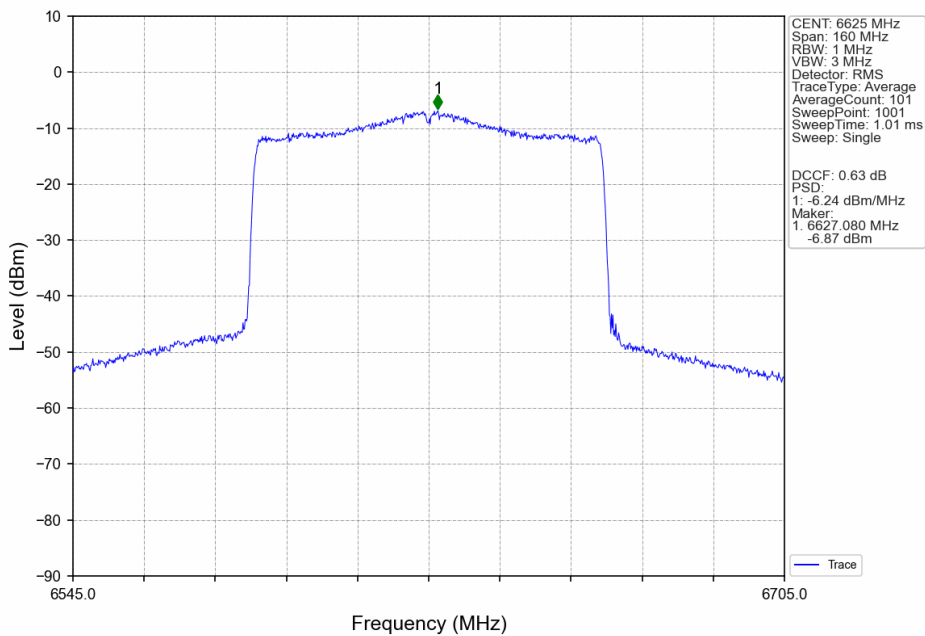
802.11ax(HEW80)_LCH_6625MHz_SU_/_ANT3_NTNV
