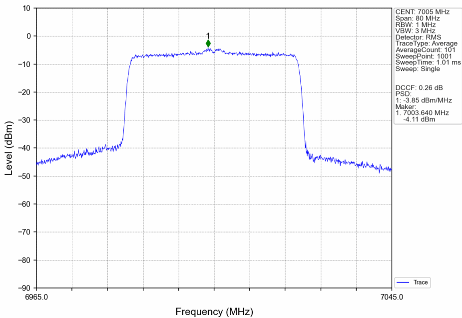
802.11ax(HEW40)_MCH_7005MHz_SU_/_ANT3_NTNV
