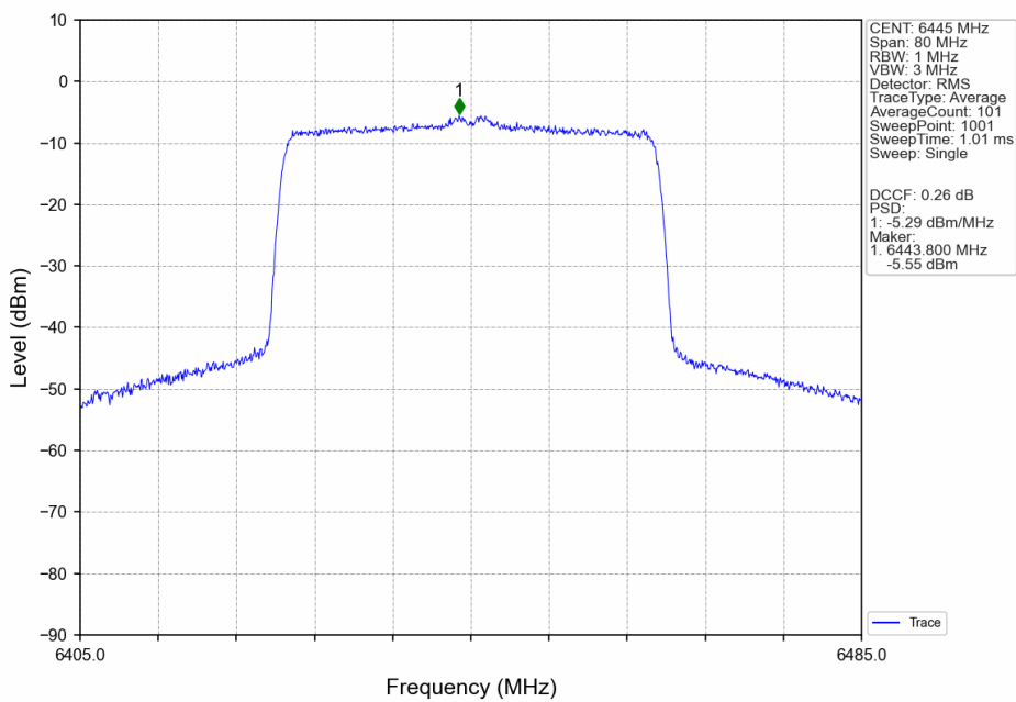
802.11ax(HEW40)_LCH_6445MHz_SU_/_ANT2_NTNV
