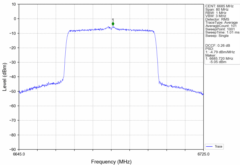
802.11ax(HEW40)_MCH_6685MHz_SU_/_ANT3_NTNV
