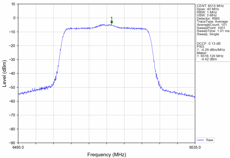
802.11ax(HEW20)_HCH_6515MHz_SU_/_ANT3_NTNV
