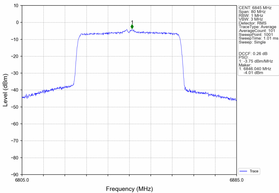
802.11ax(HEW40)_HCH_6845MHz_SU_/_ANT2_NTNV
