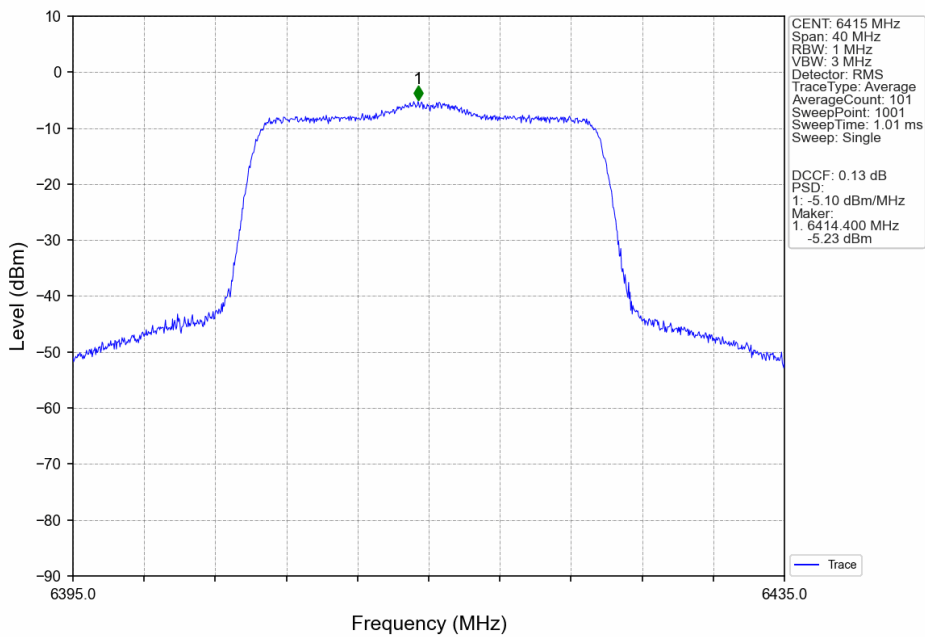
802.11ax(HEW20)_HCH_6415MHz_SU_/_ANT3_NTNV
