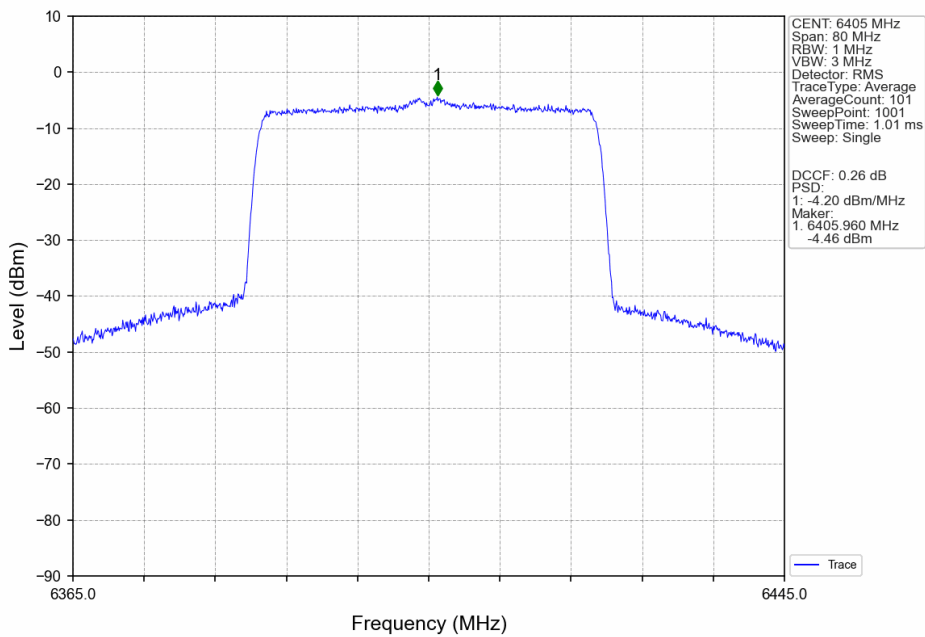
802.11ax(HEW40)_HCH_6405MHz_SU_/_ANT2_NTNV
