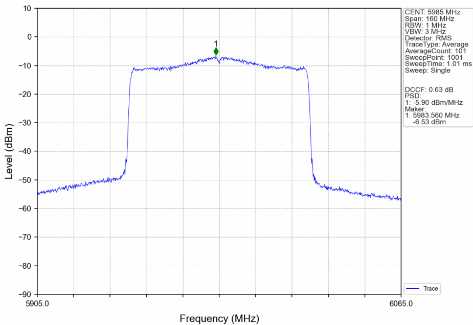
802.11ax(HEW80)_LCH_5985MHz_SU_/_ANT3_NTNV
