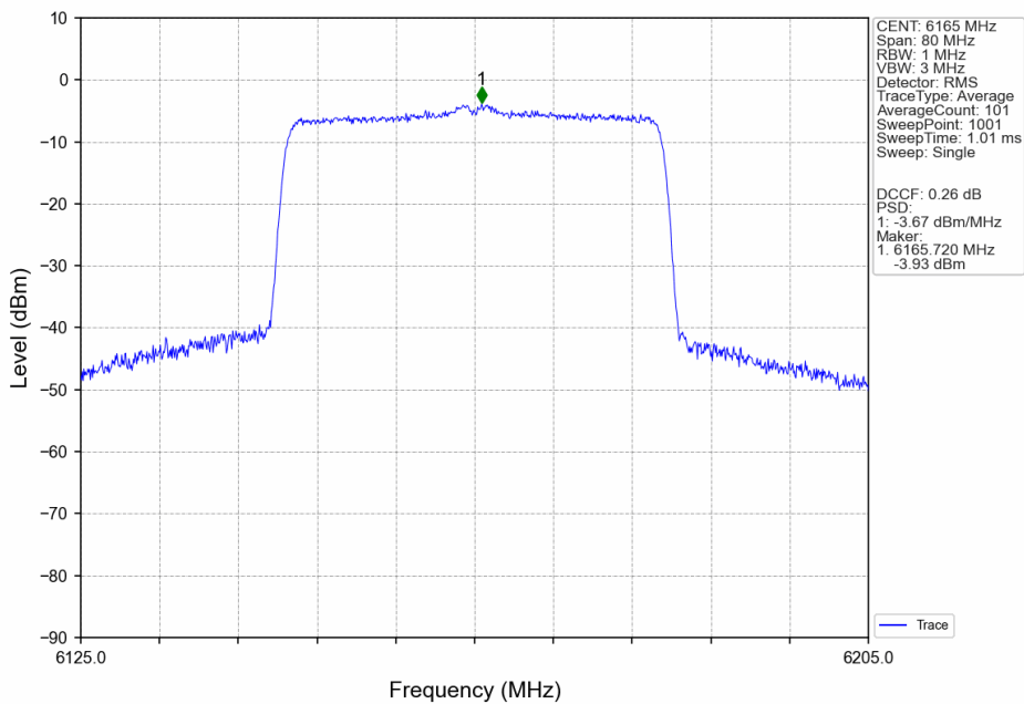
802.11ax(HEW40)_MCH_6165MHz_SU_/_ANT3_NTNV
