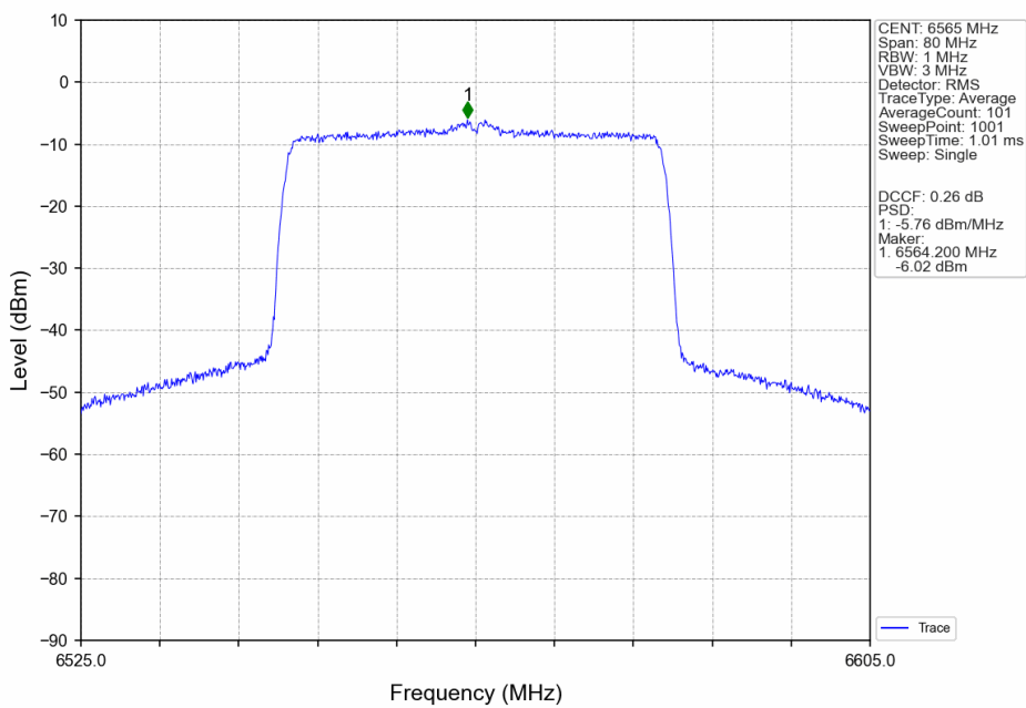
802.11ax(HEW40)_LCH_6565MHz_SU_/_ANT2_NTNV
