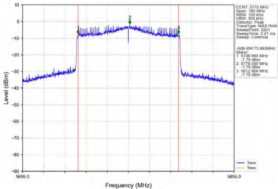
802.11ax(HEW80)_MCH_5775MHz_SU_/_ANT3_NTNV
