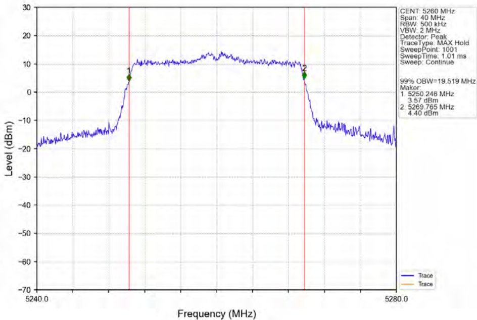
802.11ax(HEW20) LCH 5260MHz_SU / _ANT3_NTNV
