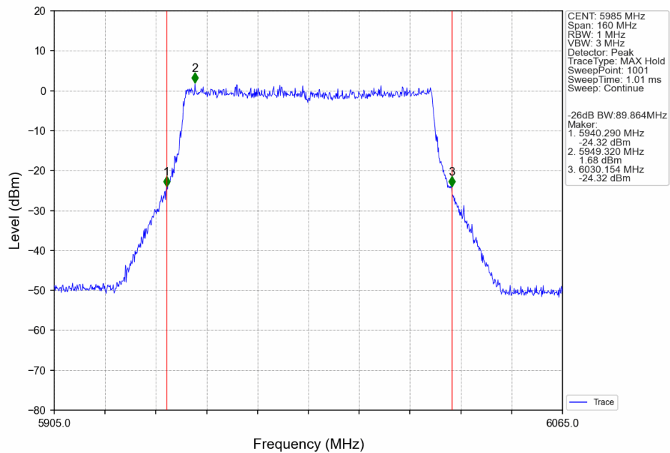
802.11ax(HEW80)_LCH_5985MHz_SU_/_ANT3_NTNV
