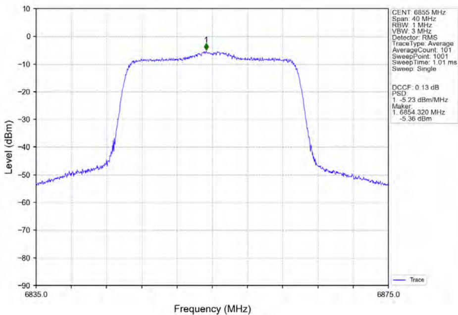
802.11ax(HEW20)_HCH_6855MHz_SU_/_ANT3_NTNV
