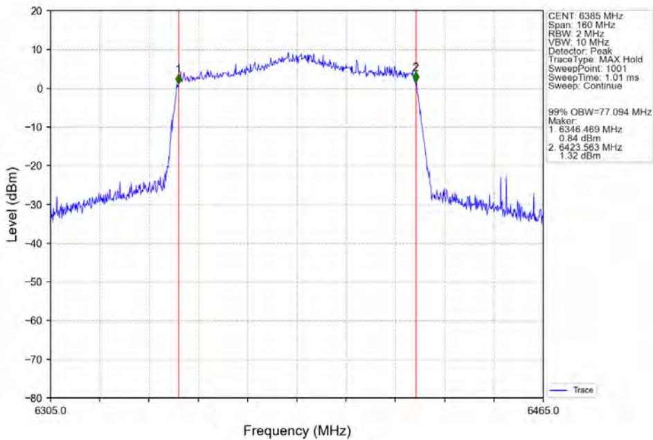
802.11ax(HEW80) HCH 6385MHz_SU / ANT3_NTNV
