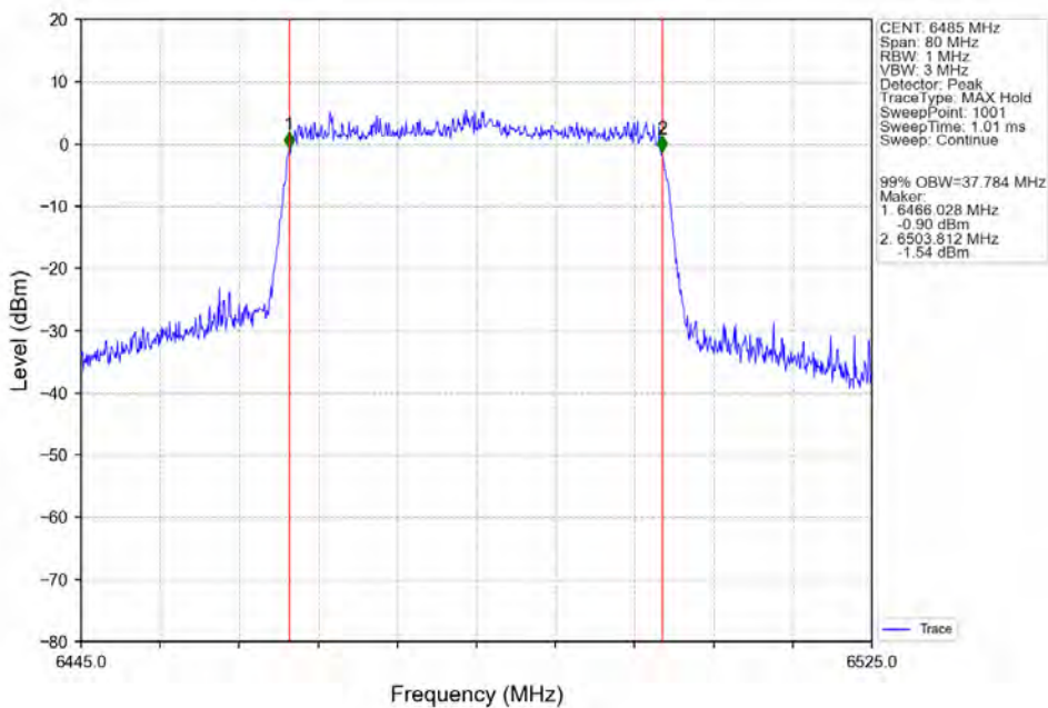
802.11ax(HEW40) MCH_6485MHz_SU / ANT3_NTNV
