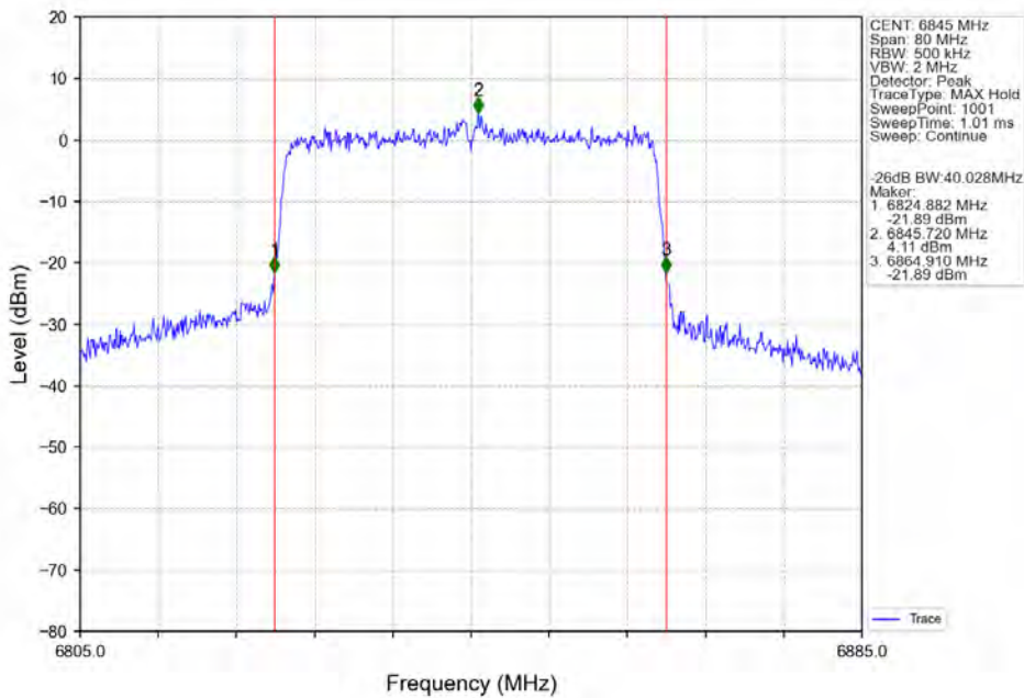
802.11ax(HEW40) HCH_6845MHz_SU / ANT3_NTNV
