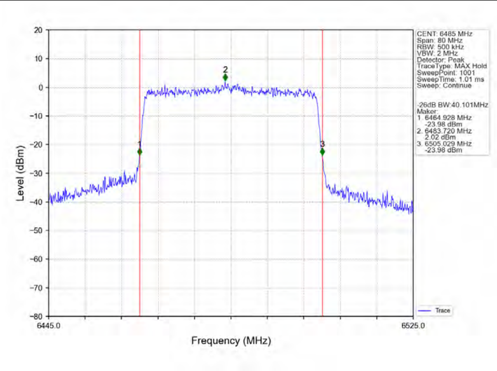
802.11ax(HEW40) MCH_6485MHz_SU / ANT3_NTNV
