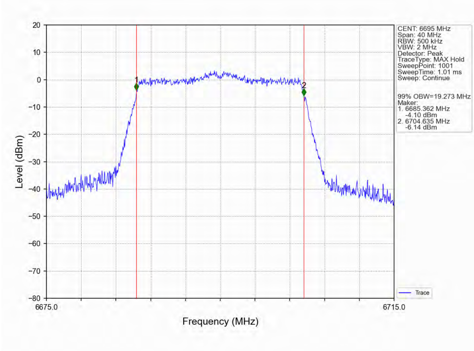
802.11ax(HEW20) MCH_6695MHz_SU / ANT3_NTNV
