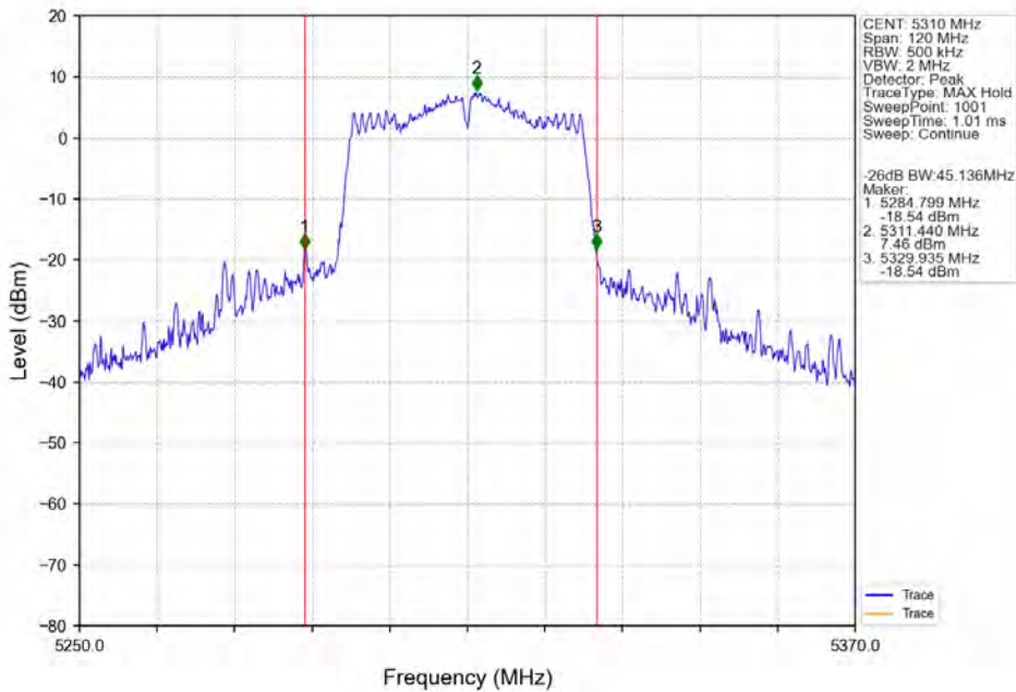
802.11ax(HEW40) HCH_5310MHz_SU_ / _ANT3_NTNV
