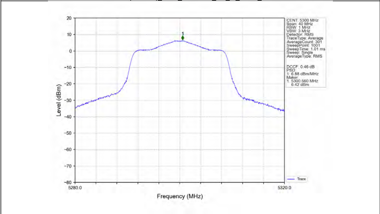
802.11ax(HEW20) MCH_5300MHz_SU_/_ANT3_NTNV
