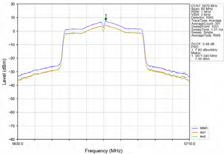
802.11n(HT40)_HCH_5670MHz_MIMO_NTNV
