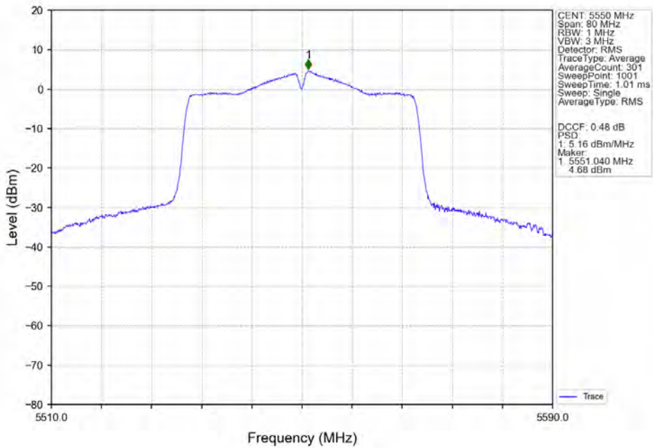
802.11n(HT40)_MCH_5550MHz_ANT3_NTNV
