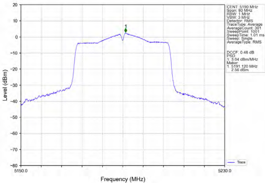
802.11ax(HEW40)_LCH_5190MHz_SU_/_ANT2_NTNV
