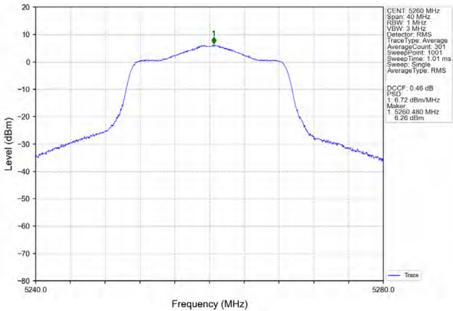
802.11ax(HEW20)_LCH_5260MHz_SU_/_MIMO_NTNV
