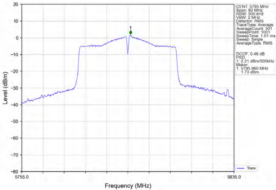
802.11n(HT40) HCH 5795MHz ANT3_NTNV
