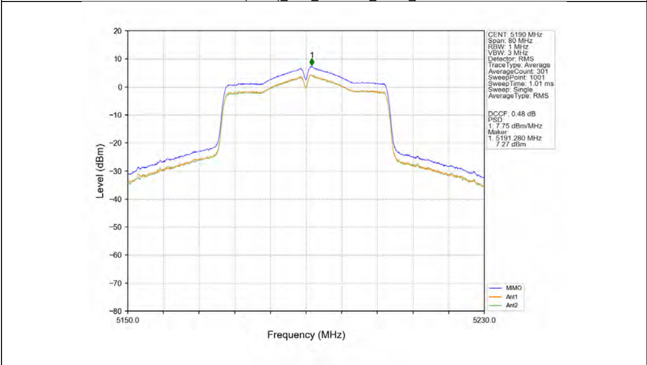
802.11n(HT40)_LCH_5190MHz_MIMO_NTNV
