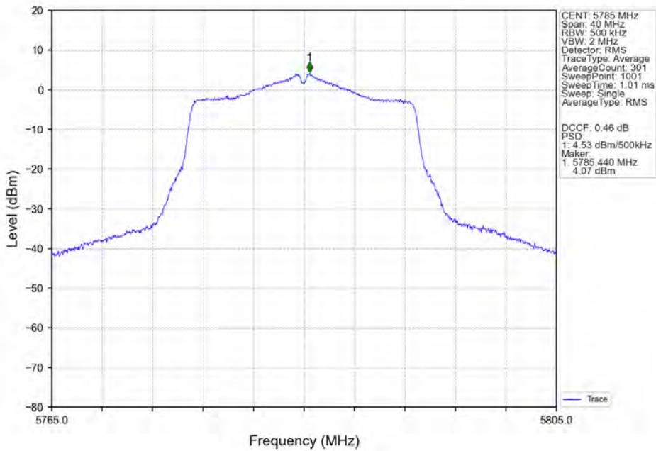
802.11ax(HEW20) MCH_5785MHz_SU_ / _MIMO_NTNV
