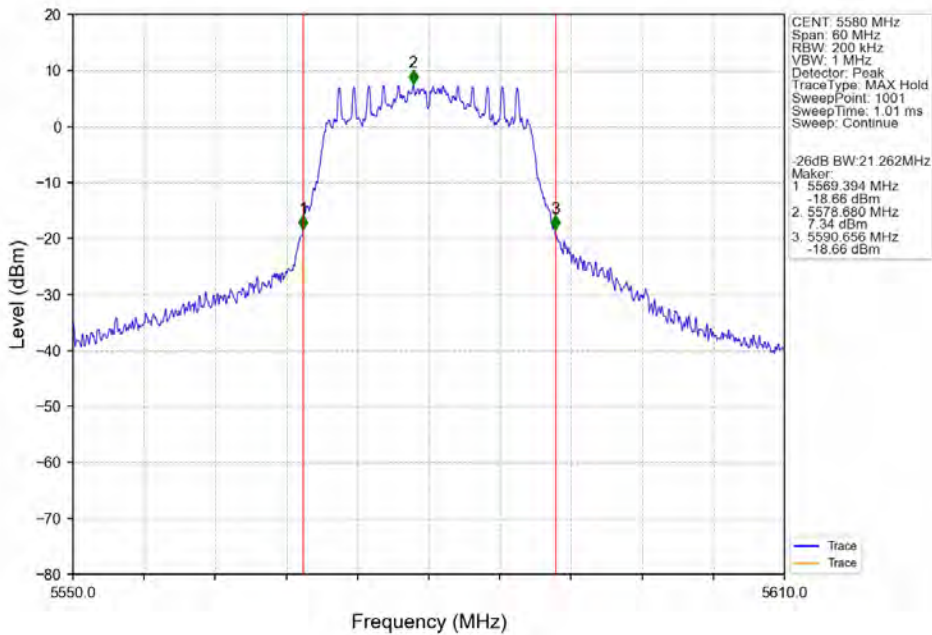
802.11ax(HEW20)_MCH_5580MHz_SU_/_ANT3_NTNV
