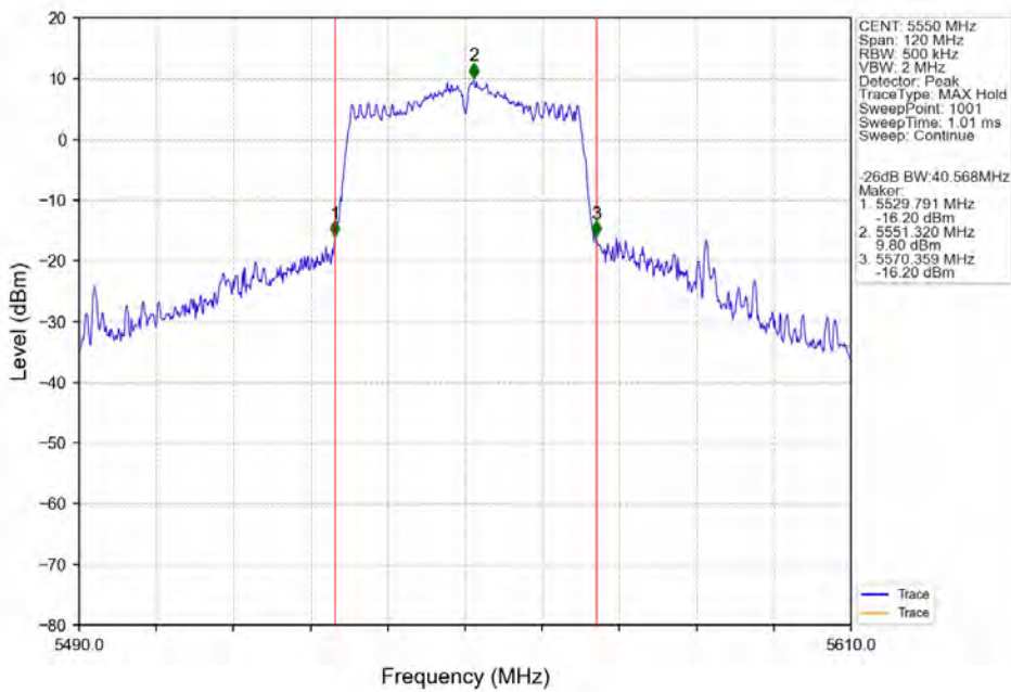
802.11n(HT40)_MCH_5550MHz_ANT3_NTNV
