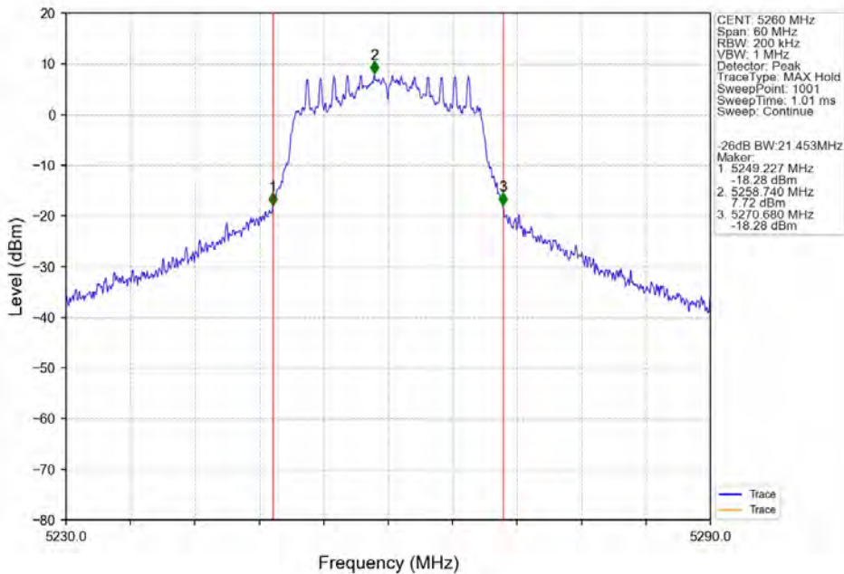
802.11ax(HEW20)_LCH_5260MHz_SU_/_ANT3_NTNV
