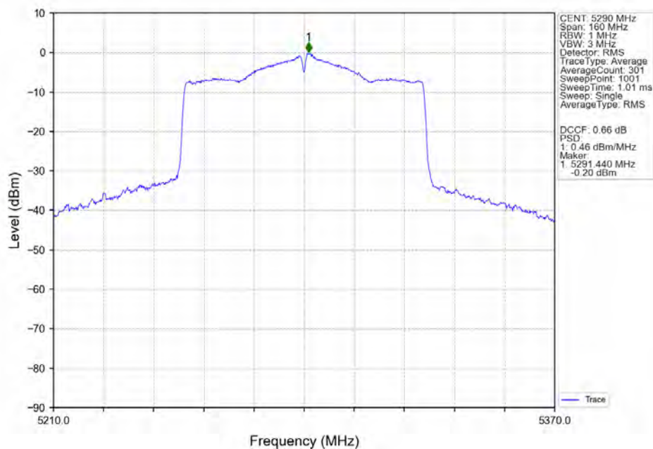
802.11ax(HEW80)_MCH_5290MHz_SU_/_ANT2_NTNV
