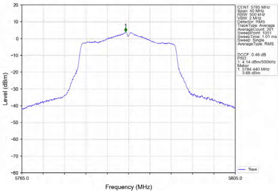
802.11ax(HEW20)_MCH_5785MHz_SU_/_ANT2_NTNV
