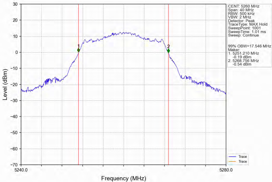
802.11a_LCH_5260MHz_ANT3_NTNV
