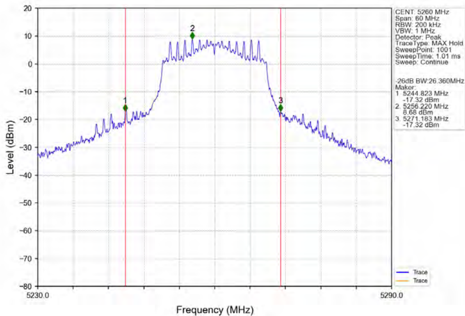
802.11n(HT20)_LCH_5260MHz_ANT3_NTNV
