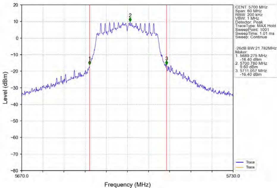
802.11n(HT20)_HCH_5700MHz_ANT3_NTNV
