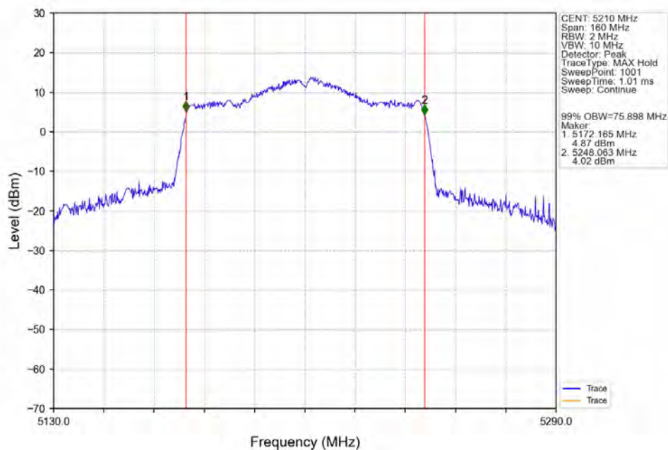
802.11ax(HEW80)_MCH_5210MHz_SU_/_ANT3_NTNV
