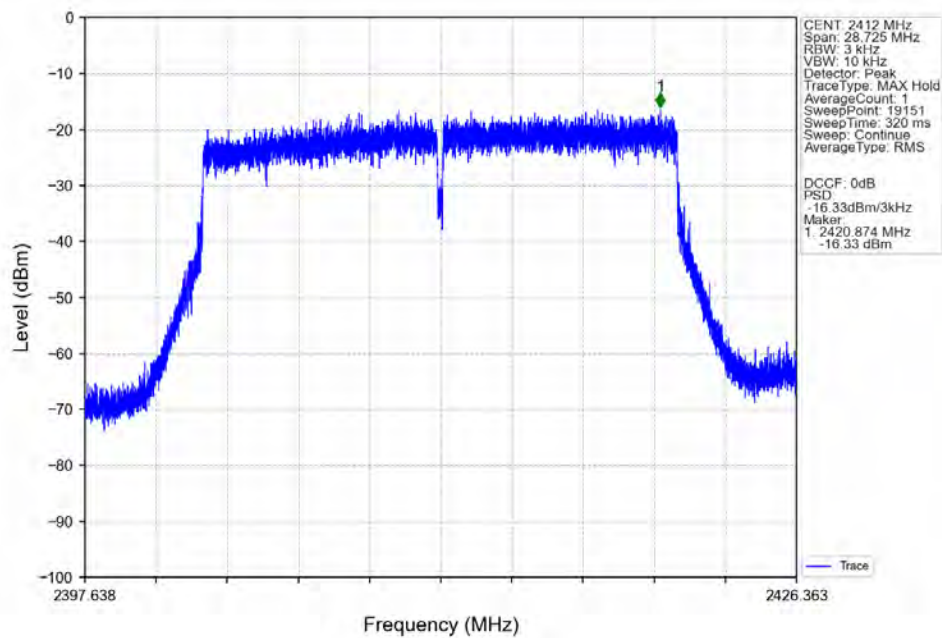
802.11ax(HEW20) LCH 2412MHz_SU / MIMO NTN
