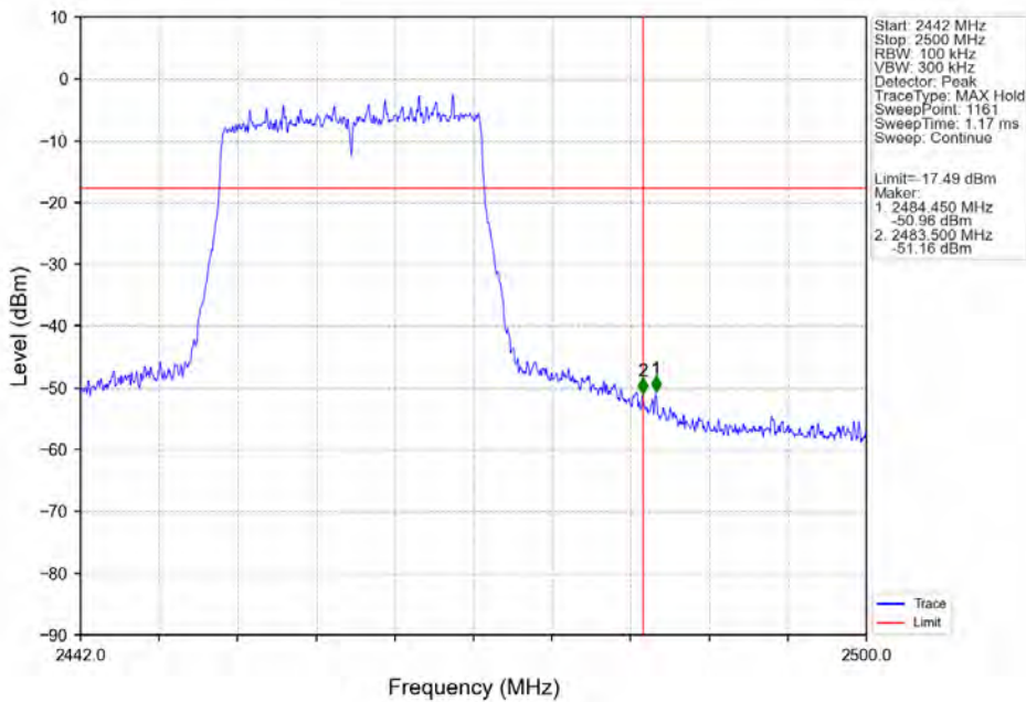
802.11ax(HEW20) HCH_2462MHz_SU / Ant3 (MIMO) NTVN
