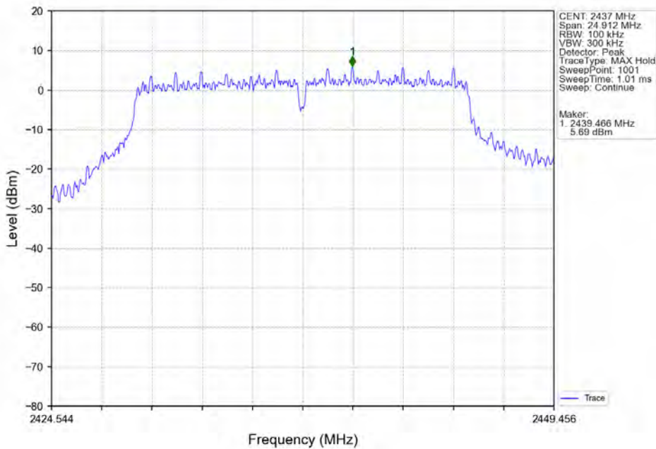
802.11g_MCH_2437MHz_Ant3 (SISO) NTN
