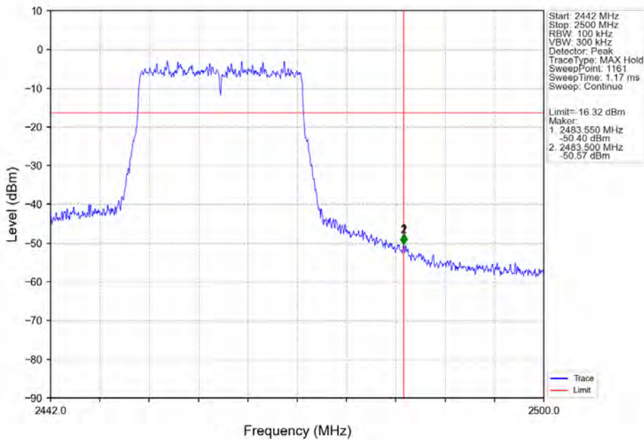
802.11ax(HEW20) HCH_2462MHz_SU / Ant2 (MIMO) NTN
