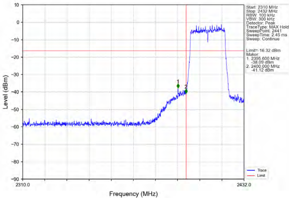
802.11ax(HEW20) LCH_2412MHz_SU / Ant2 (MIMO) NTN
