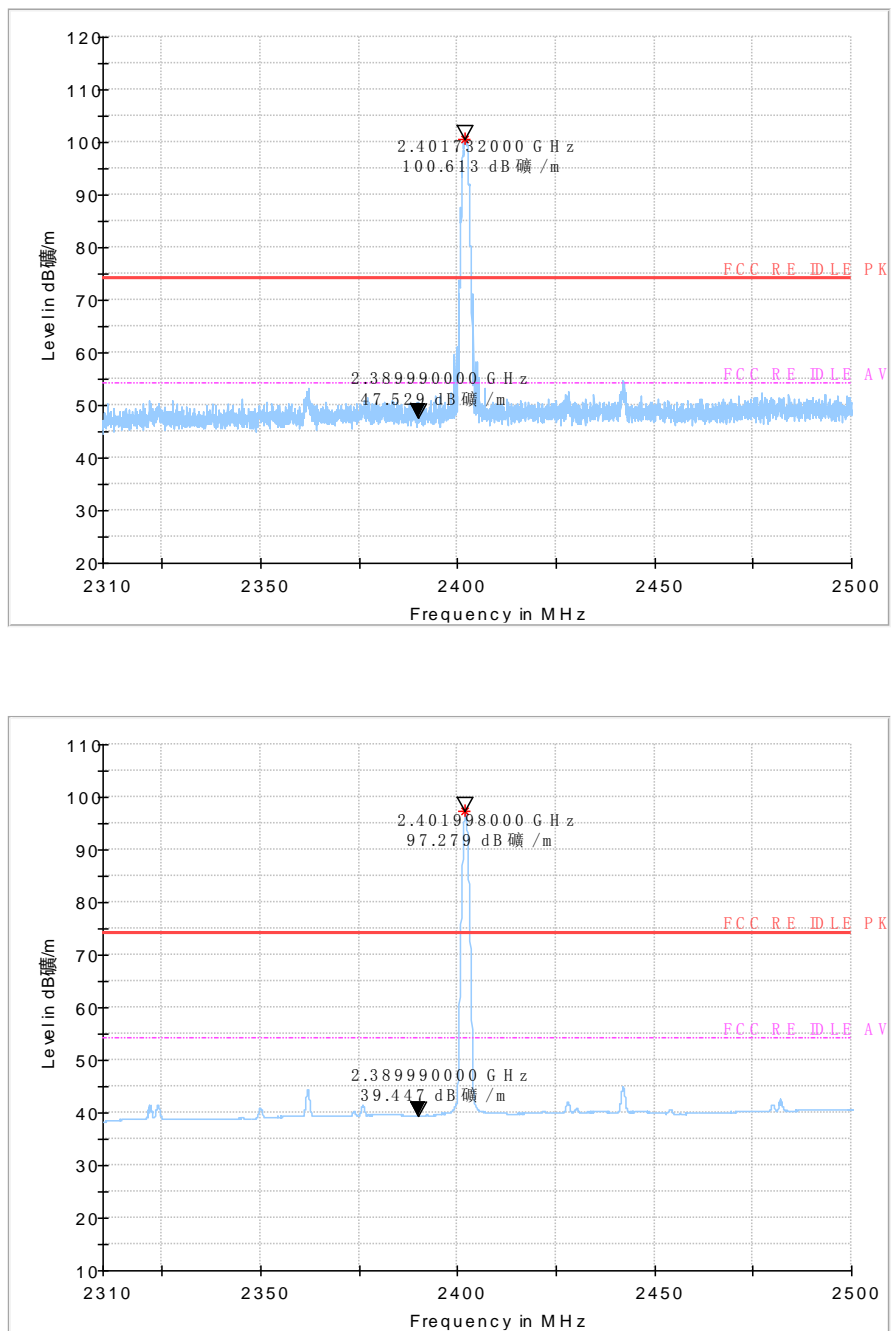
Fig.21 Bandedge:ch0
