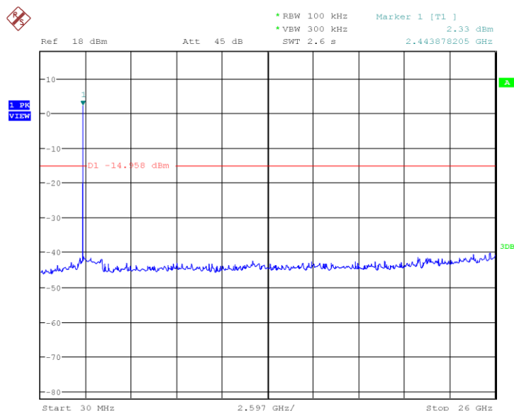
Fig.23 Conducted spurious emission: GFSK, Ch39, 30MHz~26GHz
