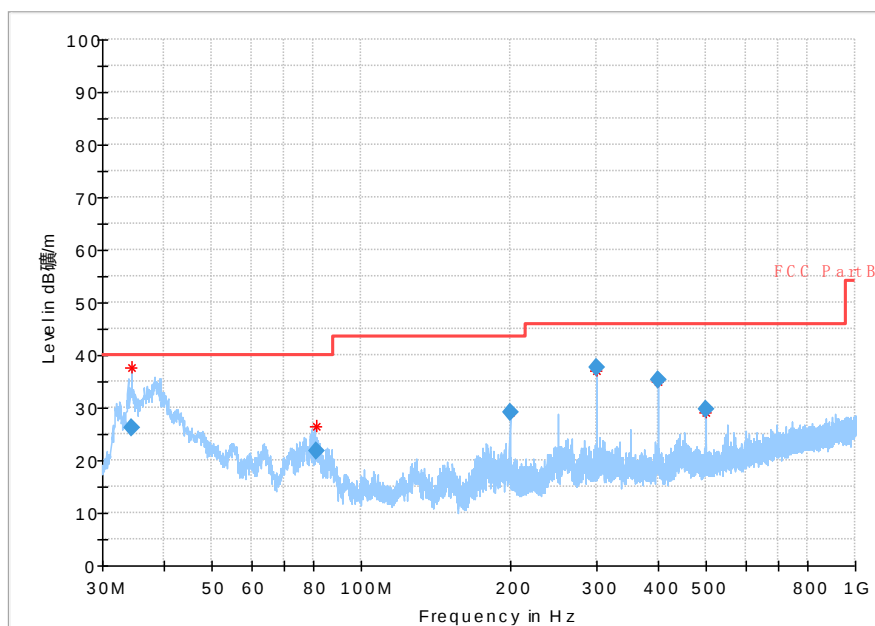
Fig.36 Radiated emission: \pi/4 DQPSK, Ch0, 30MHz~1GHz
