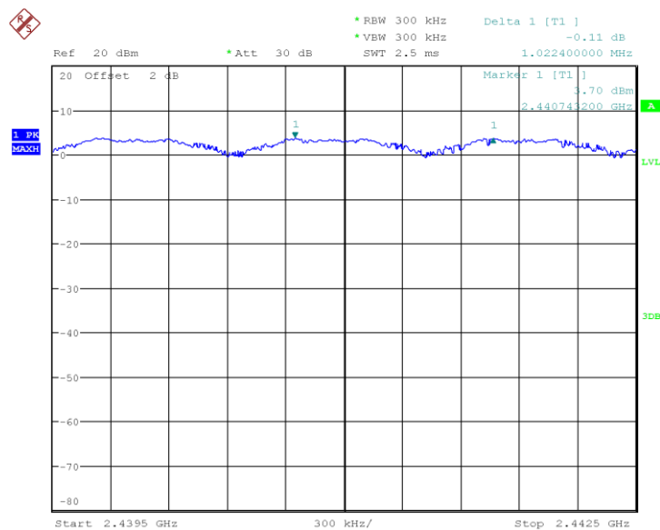
Fig.74 Carrier separation measurement: \pi/4 DQPSK, Ch39
