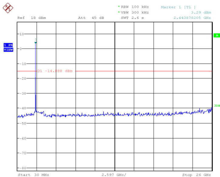
Fig.29 Conducted spurious emission: 8DPSK, Ch39, 30MHz~26GHz
