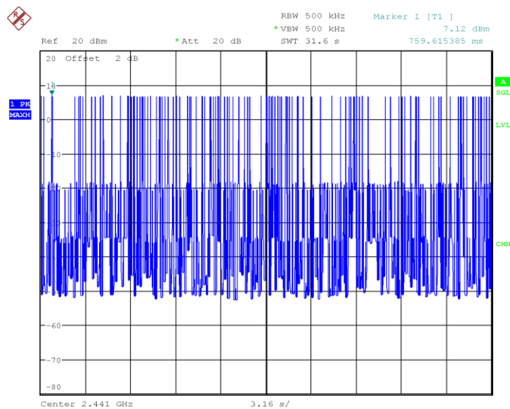
Fig.50 Time of occupancy (Dwell Time): Ch39,Packet DH5
