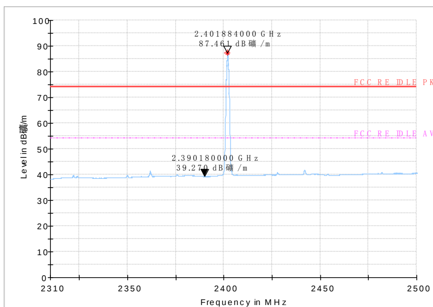
Fig.39 Bandedge (Low): \pi/4 DQPSK, low channel
