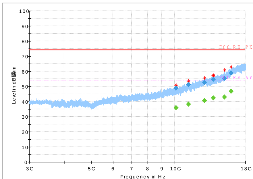
Fig.38 Radiated emission: \pi/4 DQPSK, Ch0, 3GHz~18GHz
