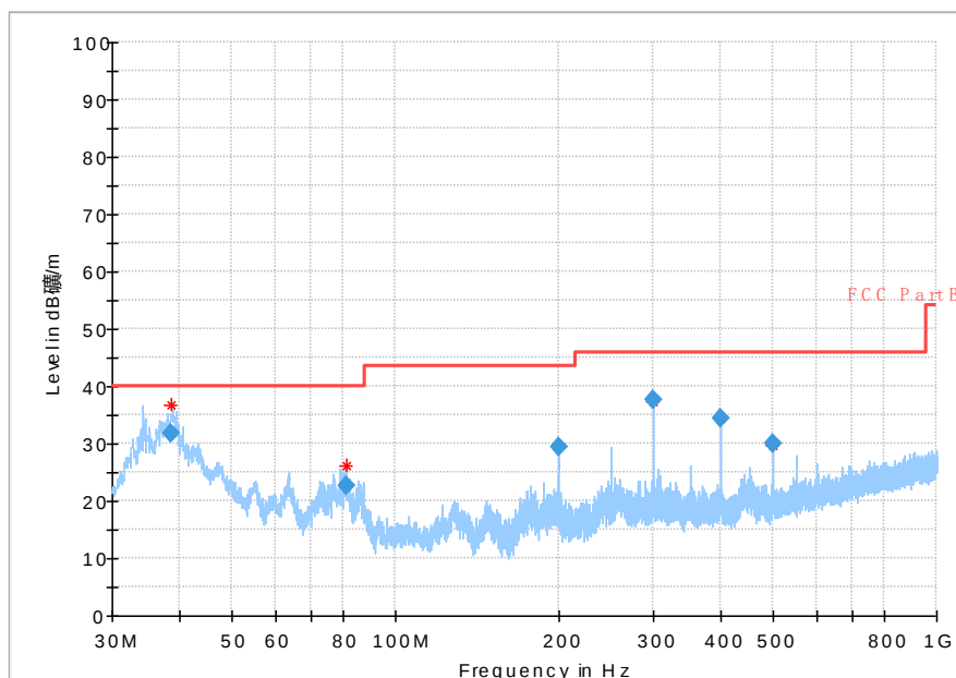
Fig.31 Radiated emission: GFSK, Ch0, 30MHz~1GHz
