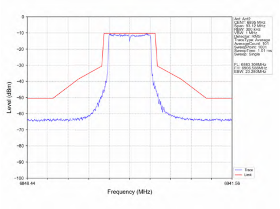
802.11ax(HEW20)_LCH_6895MHz_SU / Ant2_NTNV
