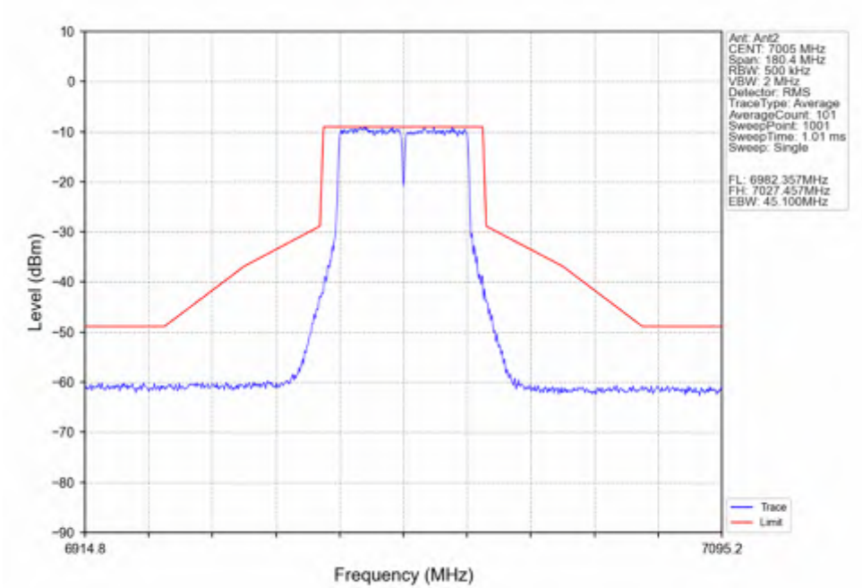
802.11ac(VHT40)_MCH_7005MHz_Ant2_NTNV
