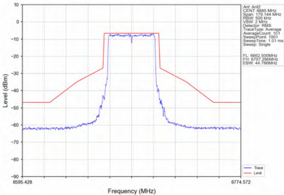
802.11ax(HEW40) MCH_6685MHz_SU / Ant2_NTNV
