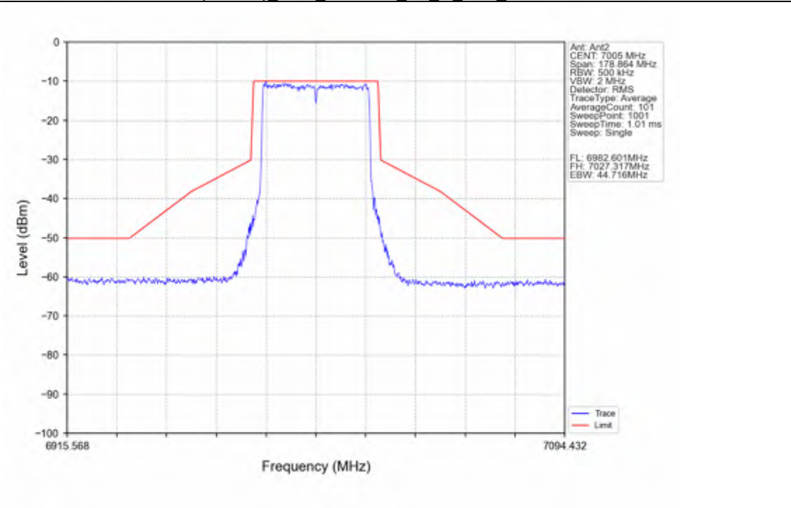
802.11ax(HEW40) MCH_7005MHz_SU / Ant2_NTNV
