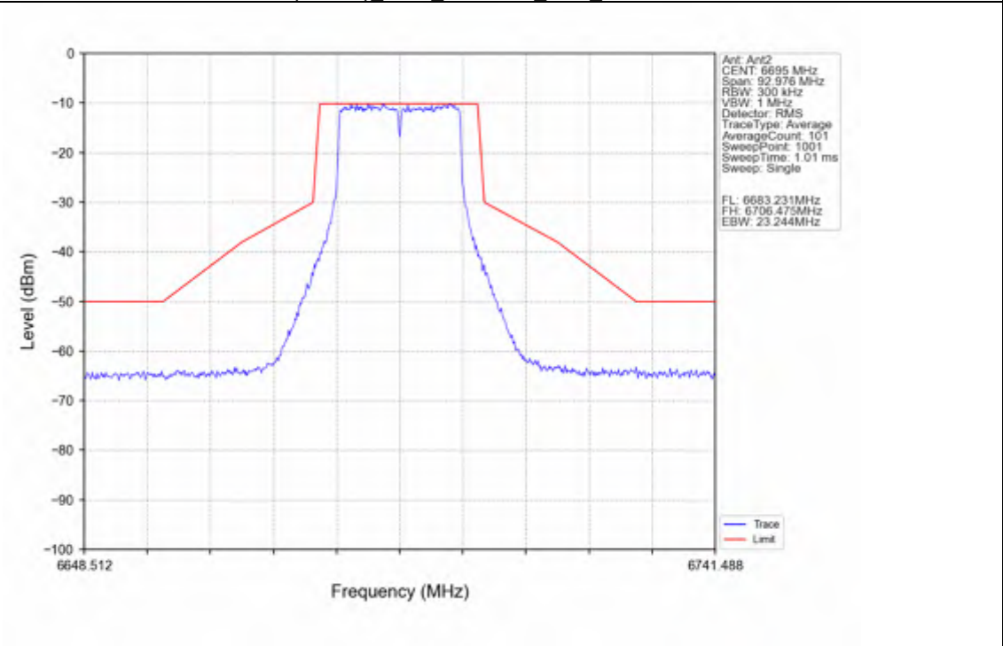
802.11ac(VHT20)_MCH_6695MHz_Ant2_NTNV
