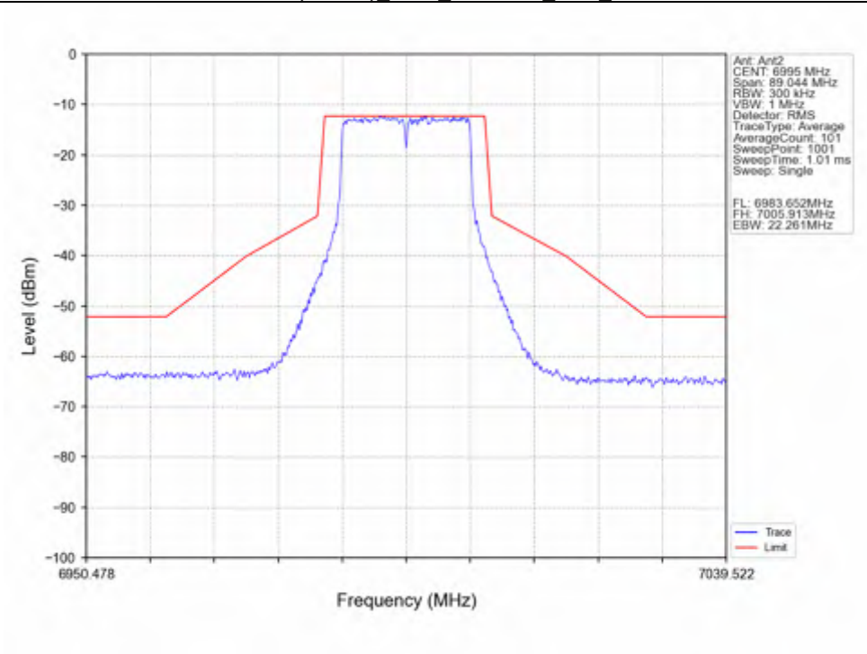
802.11ac(VHT20)_MCH_6995MHz_Ant2_NTNV
