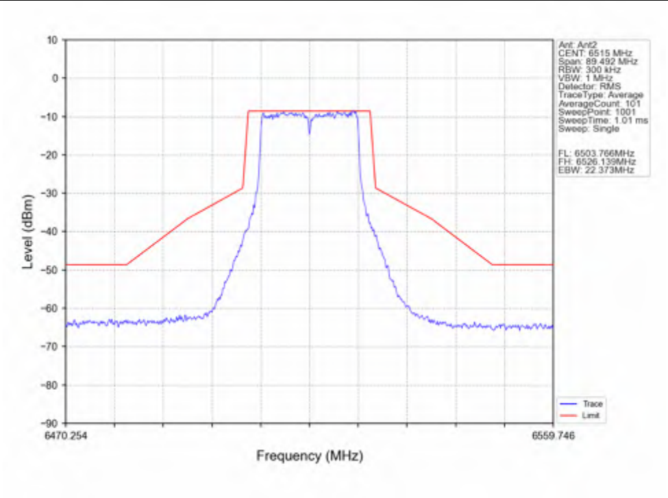
802.11n(HT20)_HCH_6515MHz_Ant2_NTNV
