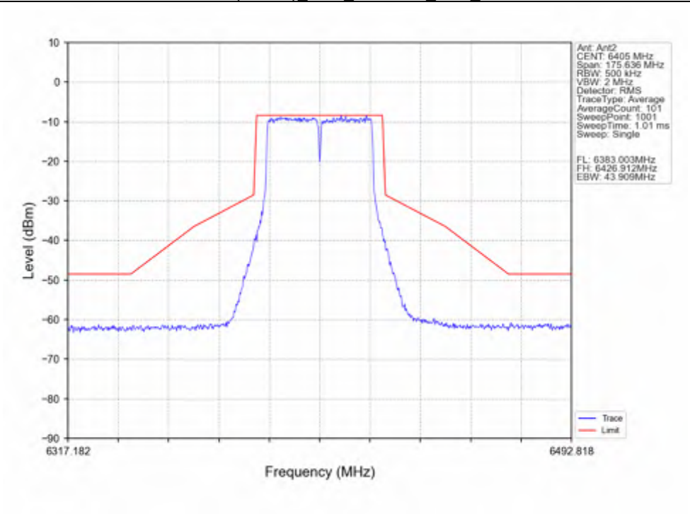
802.11ac(VHT40)_HCH_6405MHz_Ant2_NTNV
