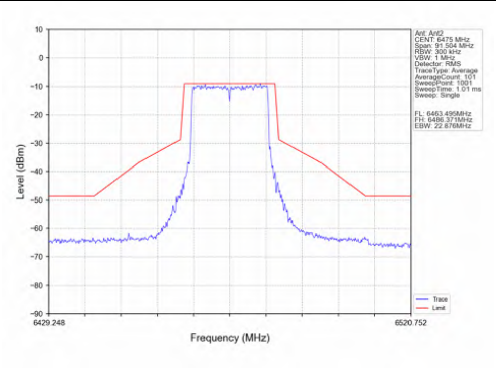
802.11ax(HEW20)_MCH_6475MHz_SU / Ant2_NTNV
