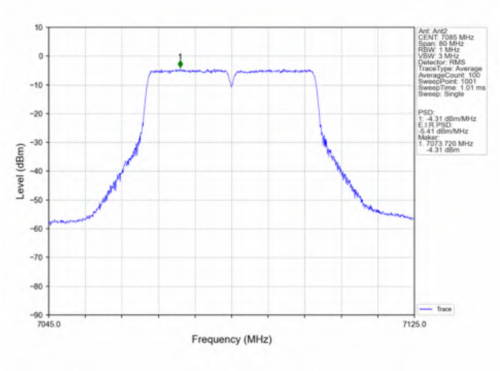
802.11ac(VHT40)_HCH_7085MHz_Ant2_NTNV
