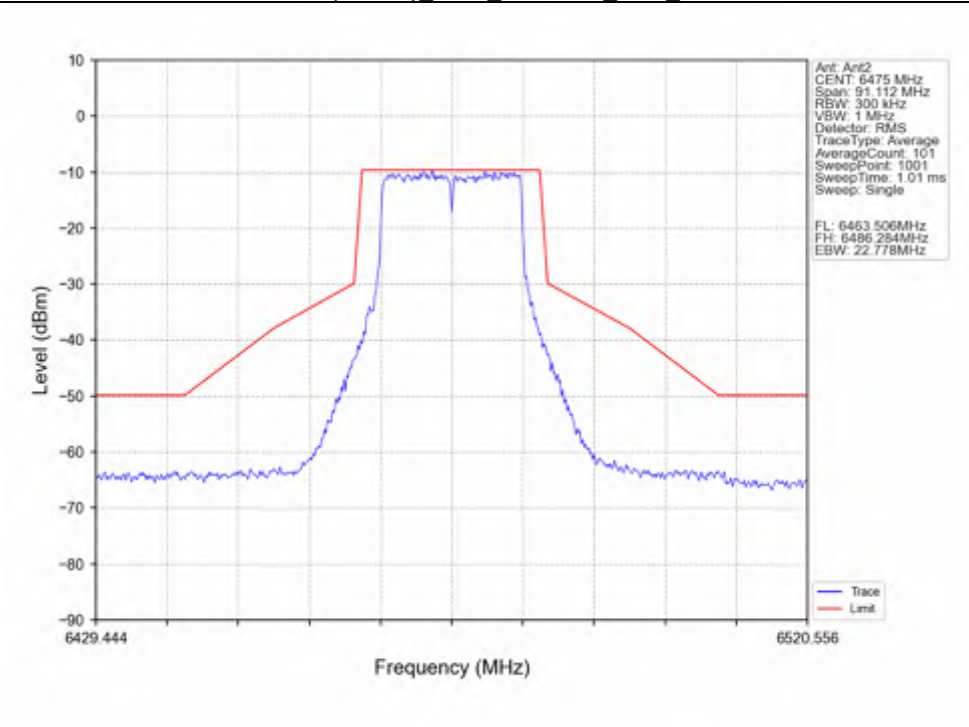
802.11ac(VHT20)_MCH_6475MHz_Ant2_NTNV
