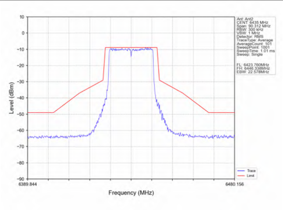
802.11ax(HEW20)_LCH_6435MHz_SU_ / Ant2_NTNV
