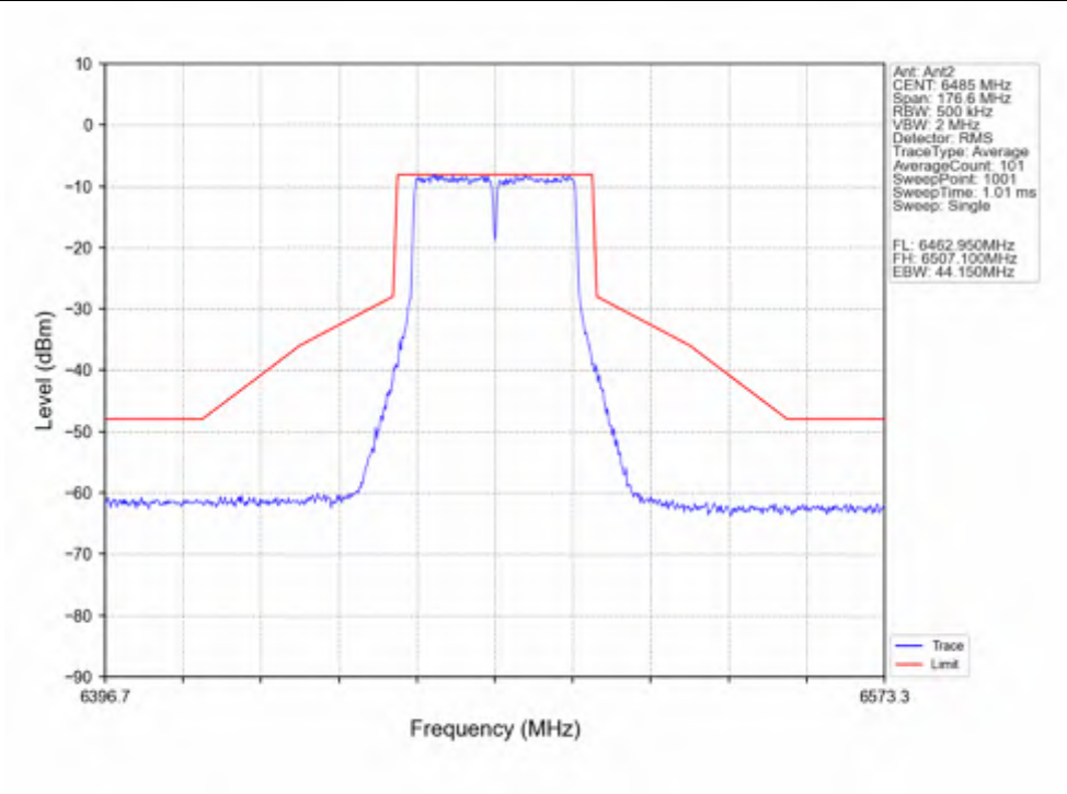
802.11n(HT40)_MCH_6485MHz_Ant2_NTNV
