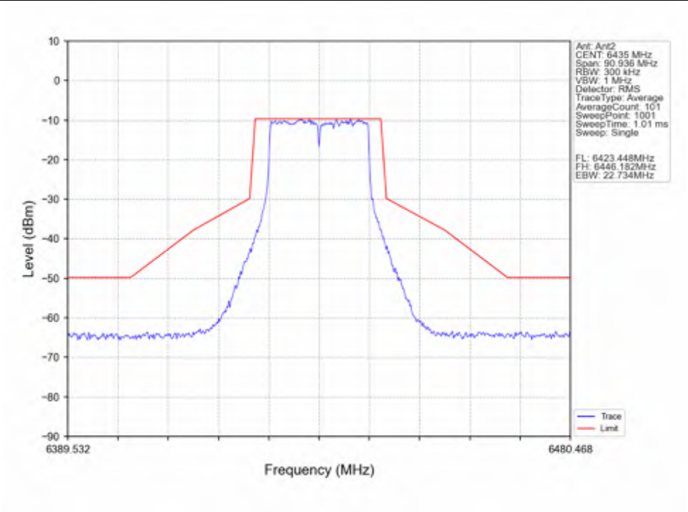
802.11ac(VHT20)_LCH_6435MHz_Ant2_NTNV
