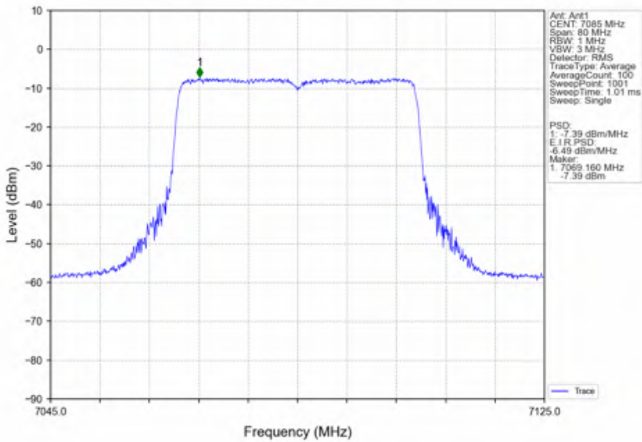
802.11ax(HEW40)_HCH_7085MHz_SU / Ant1_NTNV
