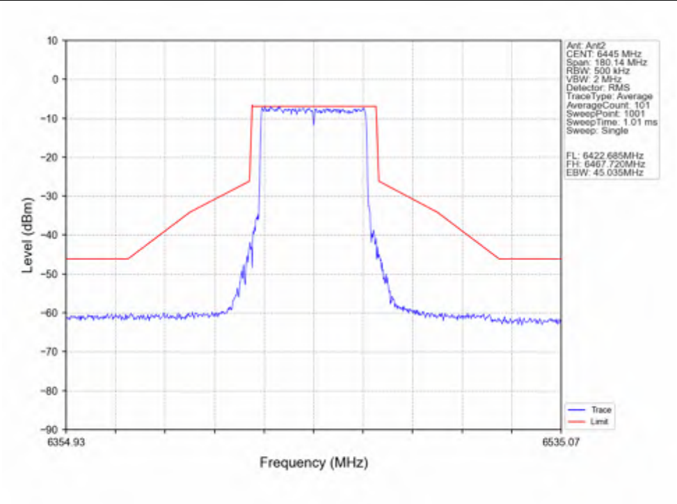
802.11ax(HEW40)_LCH_6445MHz_SU_ / Ant2_NTNV
