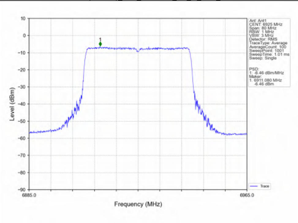
802.11ax(HEW40)_LCH_6925MHz_SU / Ant1_NTNV
