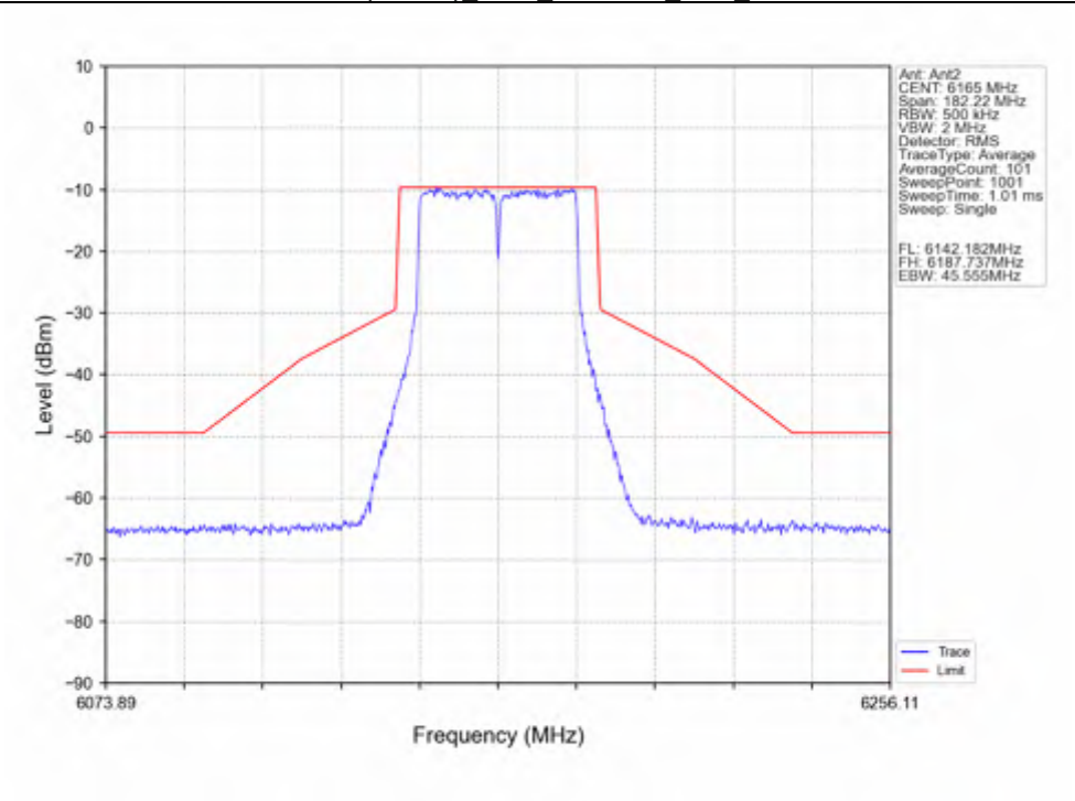
802.11ac(VHT40)_MCH_6165MHz_Ant2_NTNV
