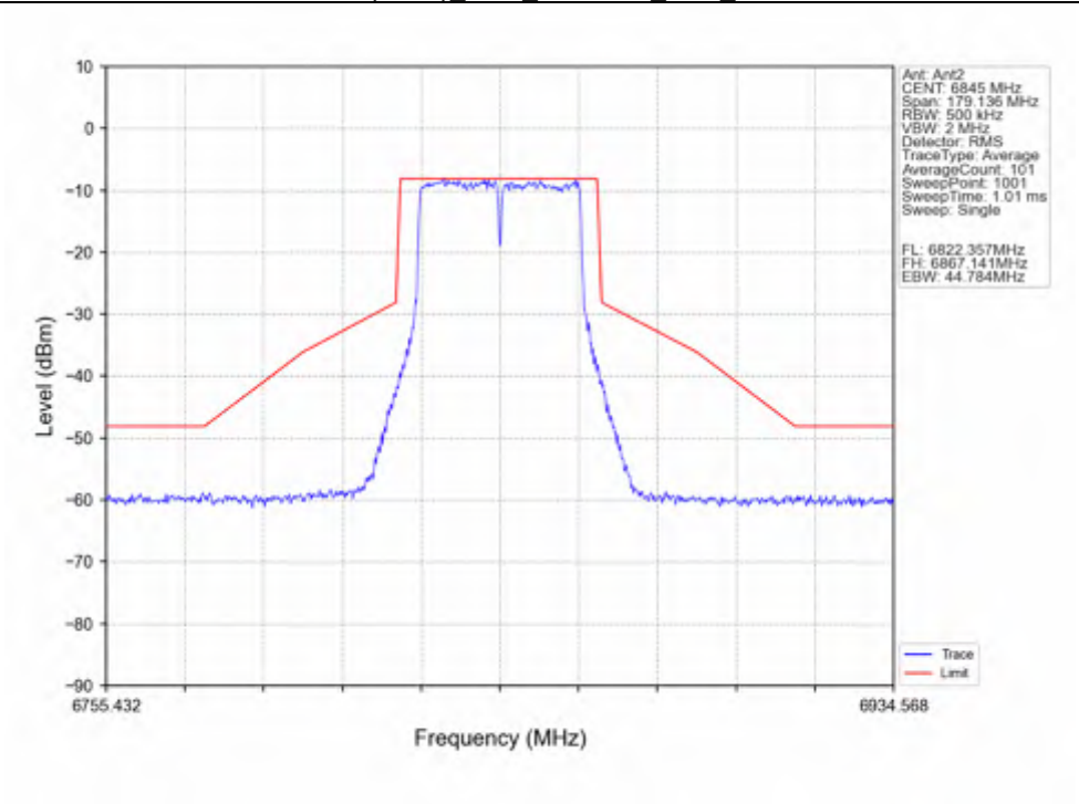
802.11n(HT40)_HCH_6845MHz_Ant2_NTNV
