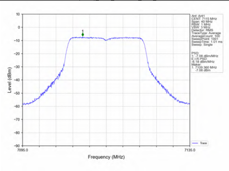
802.11n(HT20)_HCH_7115MHz_Ant1_NTNV
