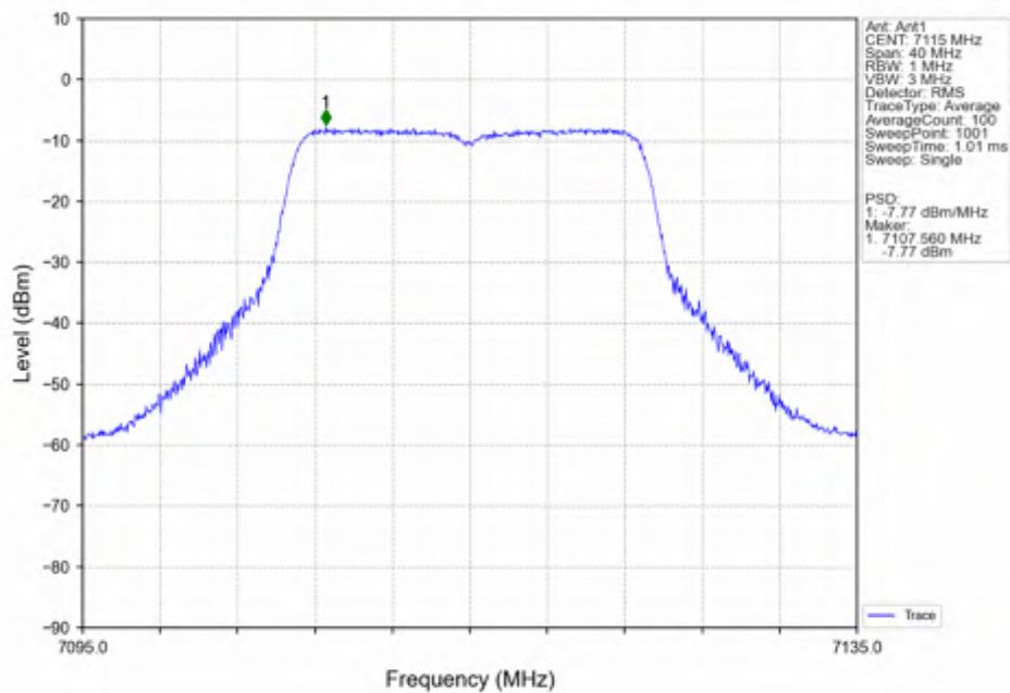
802.11ac(VHT20)_HCH_7115MHz_Ant1_NTNV
