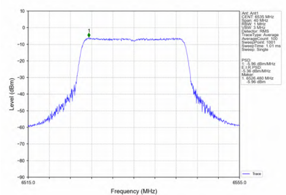
802.11ax(HEW20)_LCH_6535MHz_SU / Ant1_NTNV
