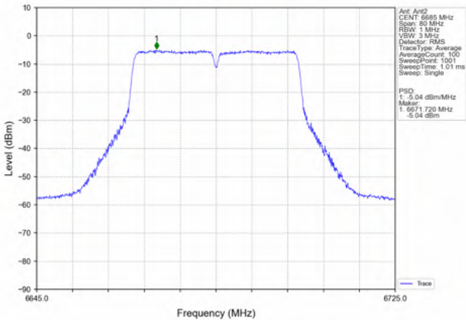
802.11n(HT40)_MCH_6685MHz_MIMO_NTNV
