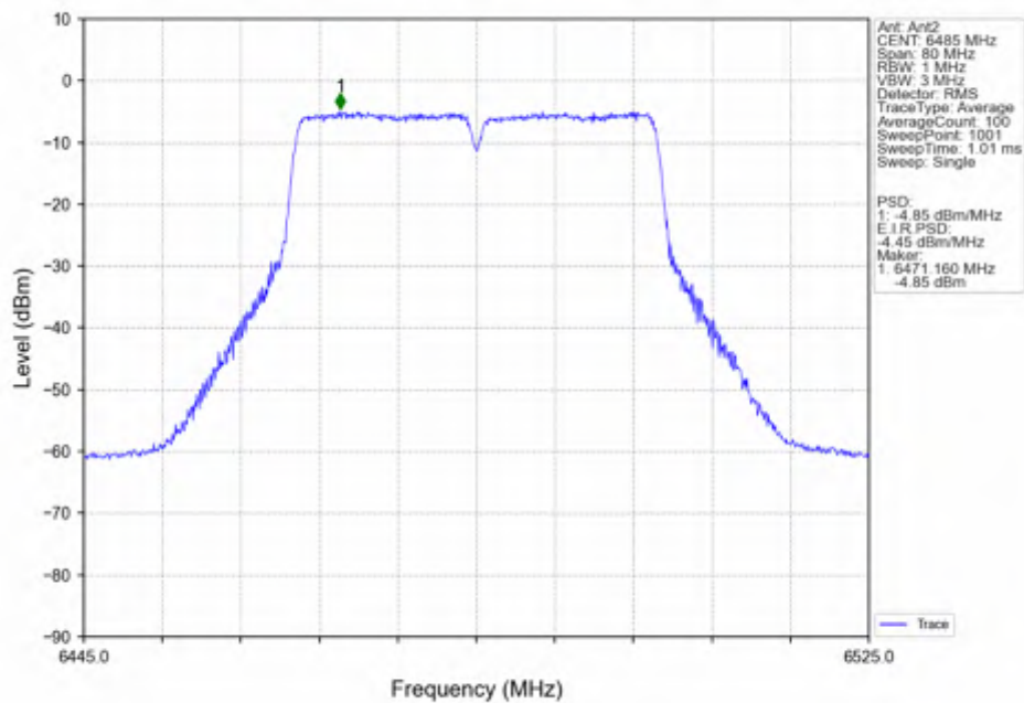
802.11ac(VHT40)_MCH_6485MHz_Ant2_NTNV
