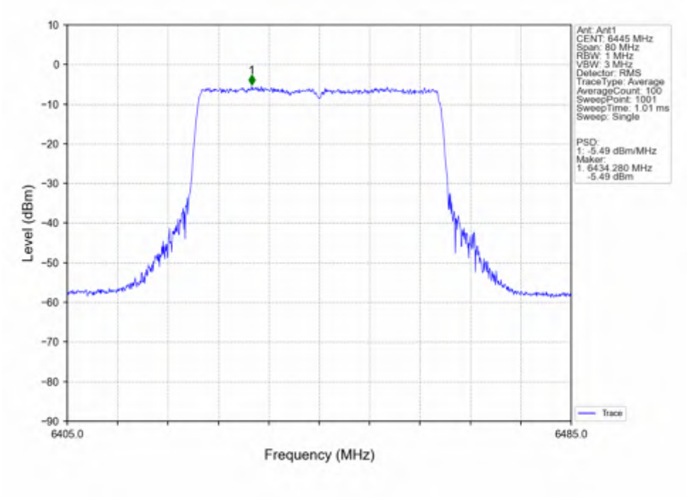
802.11ax(HEW40)_LCH_6445MHz_SU / Ant1_NTNV
