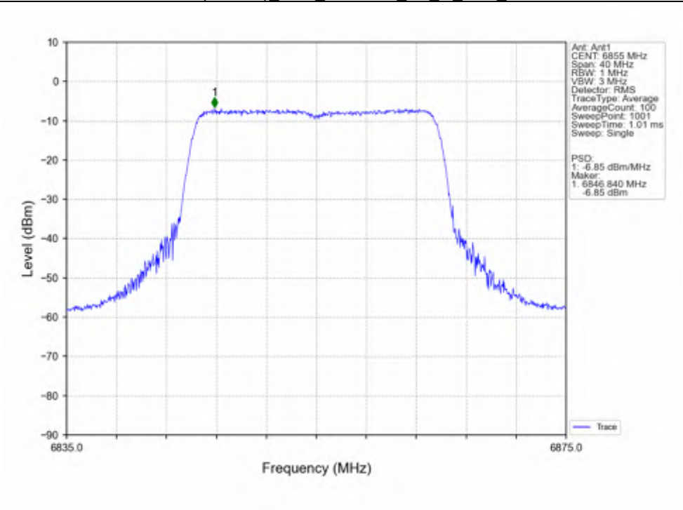
802.11ax(HEW20)_HCH_6855MHz_SU / Ant1_NTNV
