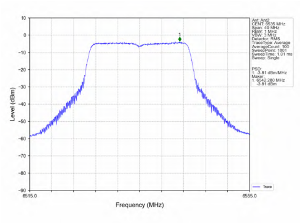
802.11n(HT20)_LCH_6535MHz_MIMO_NTNV
