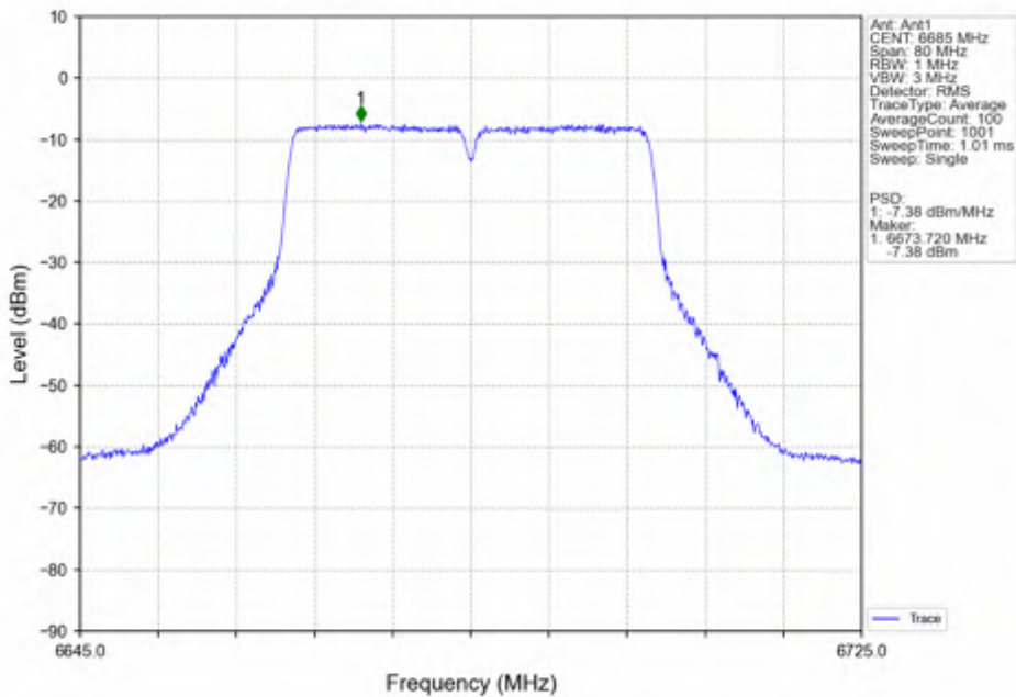
802.11ac(VHT40)_MCH_6685MHz_Ant1_NTNV
