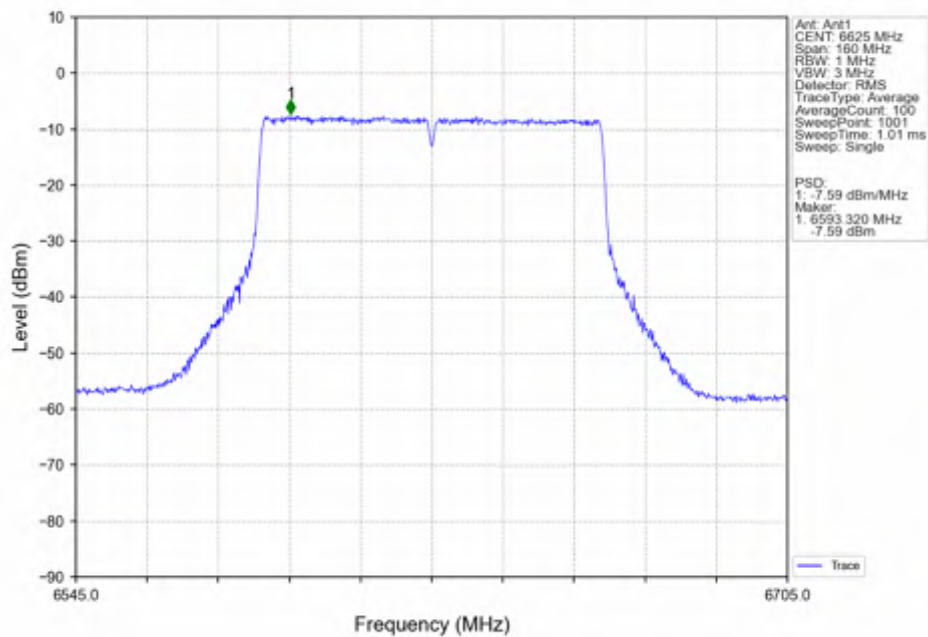
802.11ac(VHT80)_LCH_6625MHz_Ant1_NTNV
