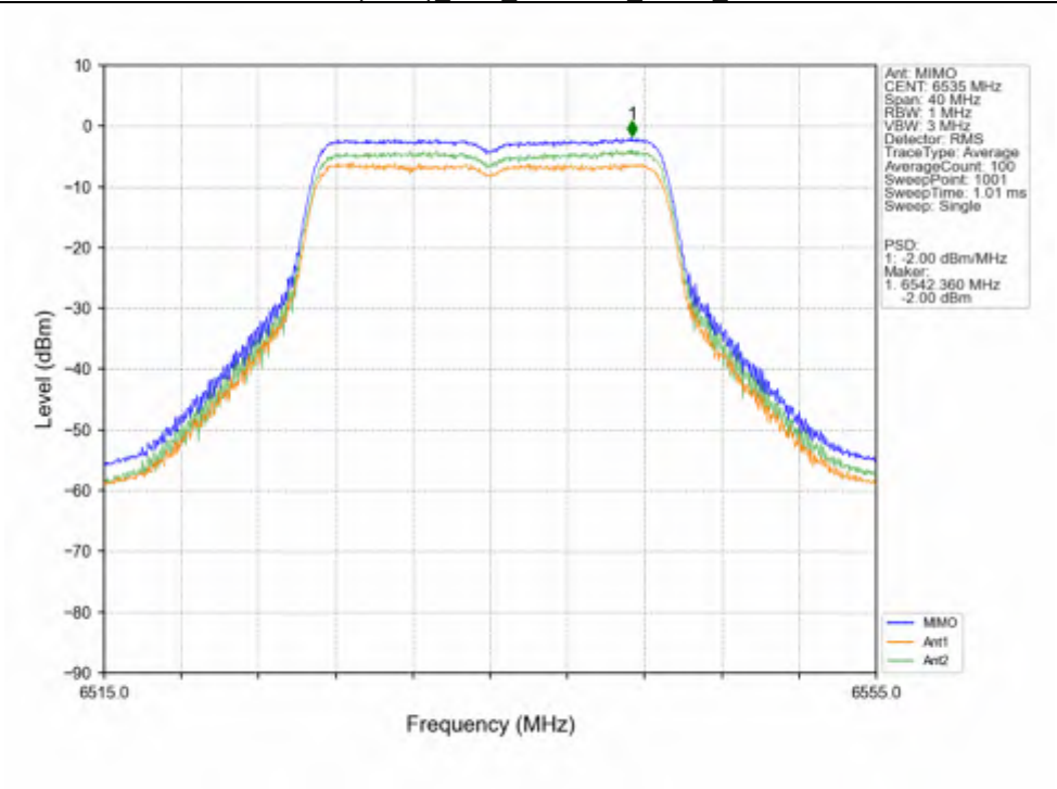
802.11n(HT20)_LCH_6535MHz_MIMO_NTNV
