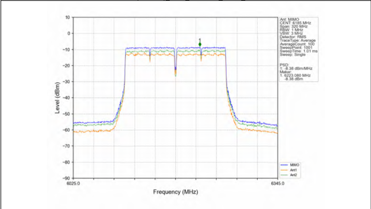
802.11ac(VHT160)_MCH_6185MHz_MIMO_NTNV
