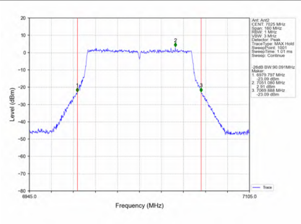
802.11ac(VHT80)_HCH_7025MHz_Ant2_NTNV
