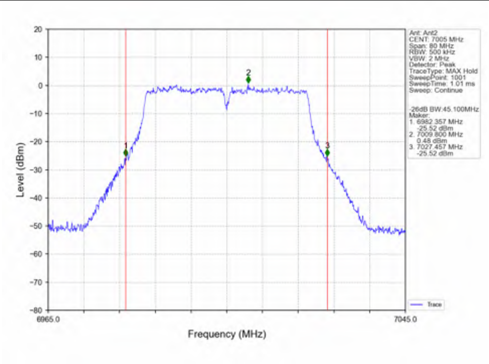
802.11ac(VHT40)_MCH_7005MHz_Ant2_NTNV
