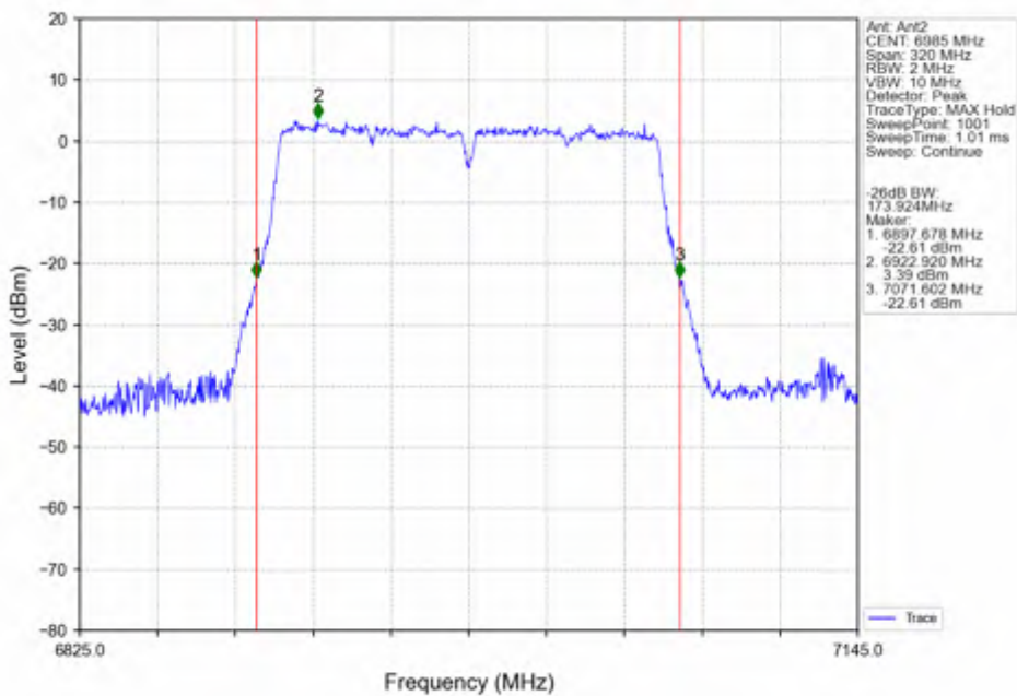
802.11ac(VHT160)_MCH_6985MHz_Ant2_NTNV
