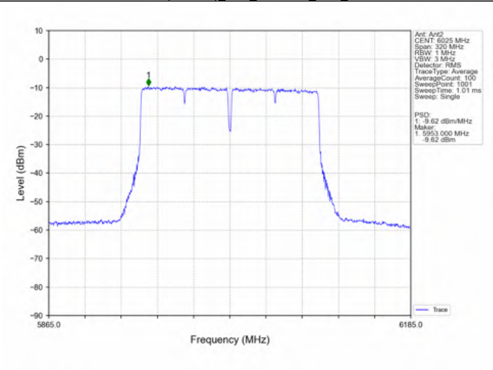
802.11ac(VHT160)_LCH_6025MHz_Ant2_NTNV
