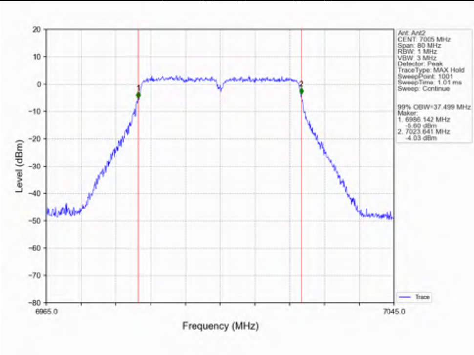
802.11ac(VHT40)_MCH_7005MHz_Ant2_NTNV
