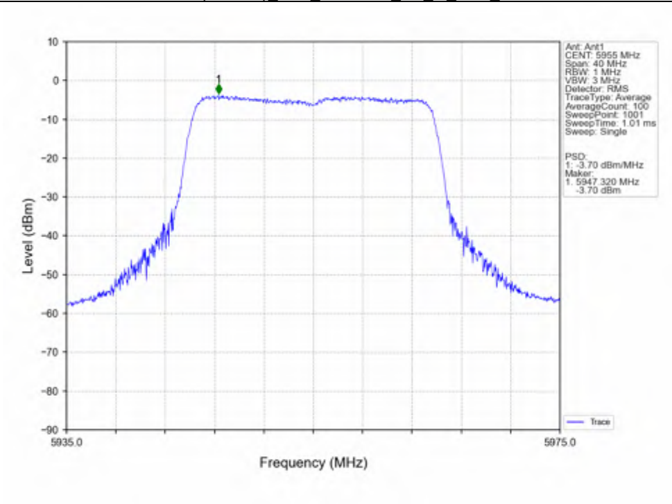
802.11ax(HEW20)_LCH_5955MHz_SU / Ant1_NTNV
