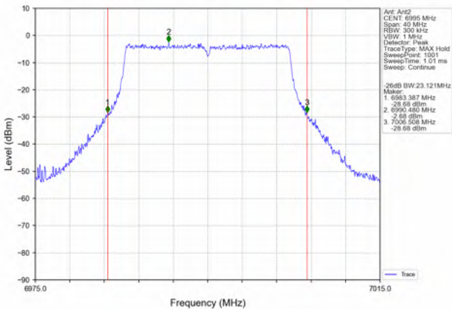
802.11ax(HEW20)_MCH_6995MHz_SU / Ant2_NTNV
