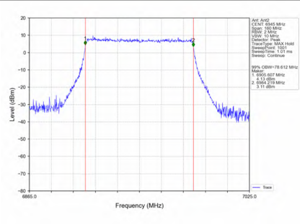
802.11ax(HEW80)_LCH_6945MHz_SU / Ant2_NTNV
