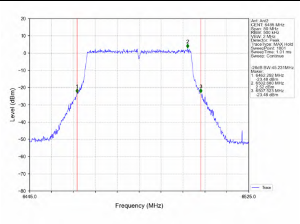
802.11ax(HEW40)_MCH_6485MHz_SU / Ant2_NTNV
