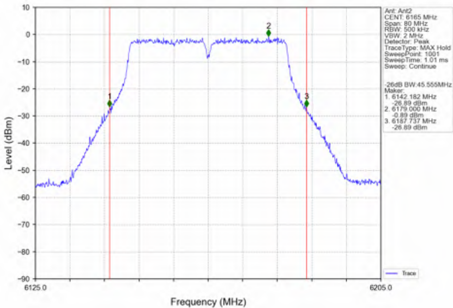
802.11ac(VHT40)_MCH_6165MHz_Ant2_NTNV
