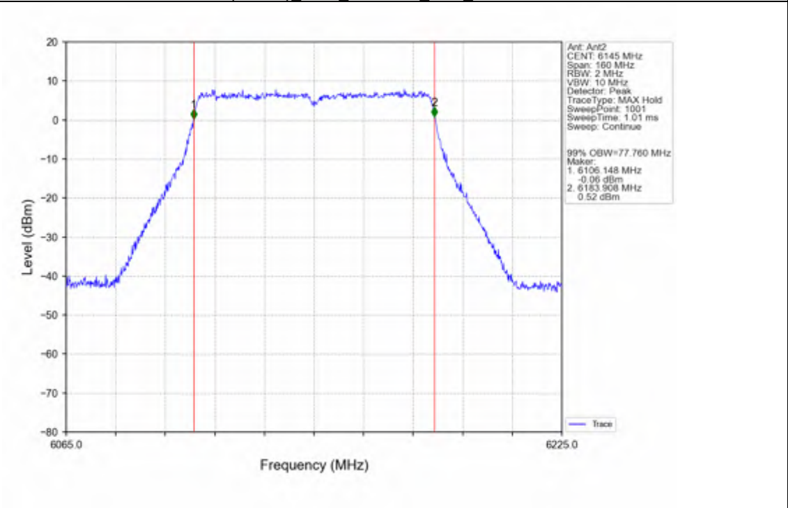
802.11ac(VHT80)_MCH_6145MHz_Ant2_NTNV
