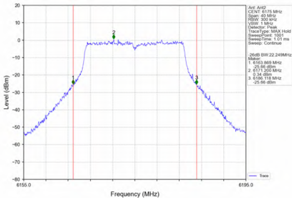
802.11n(HT20)_MCH_6175MHz_Ant2_NTNV
