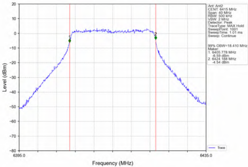
802.11ac(VHT20)_HCH_6415MHz_Ant2_NTNV
