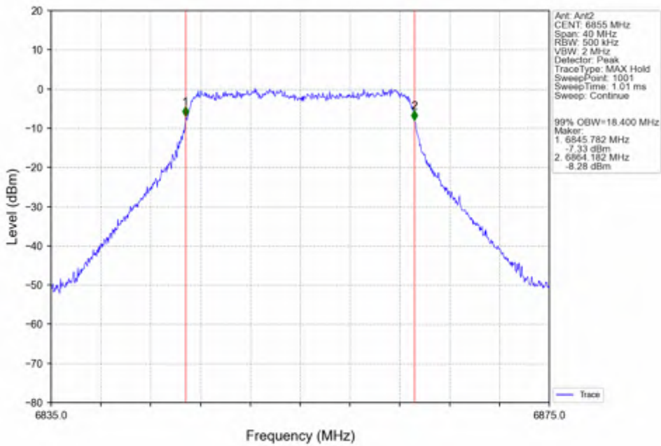
802.11ac(VHT20)_HCH_6855MHz_Ant2_NTNV
