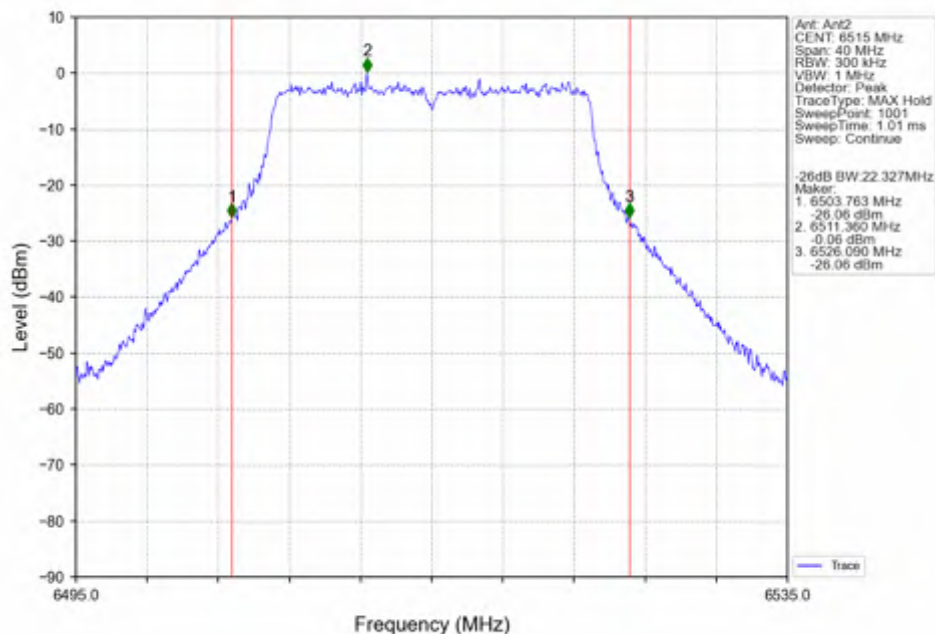
802.11ac(VHT20)_HCH_6515MHz_Ant2_NTNV
