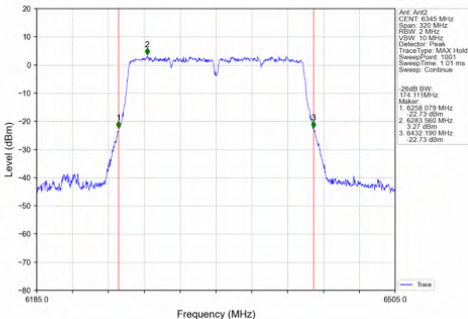
802.11ac(VHT160) HCH_6345MHz_Ant2_NTNV
