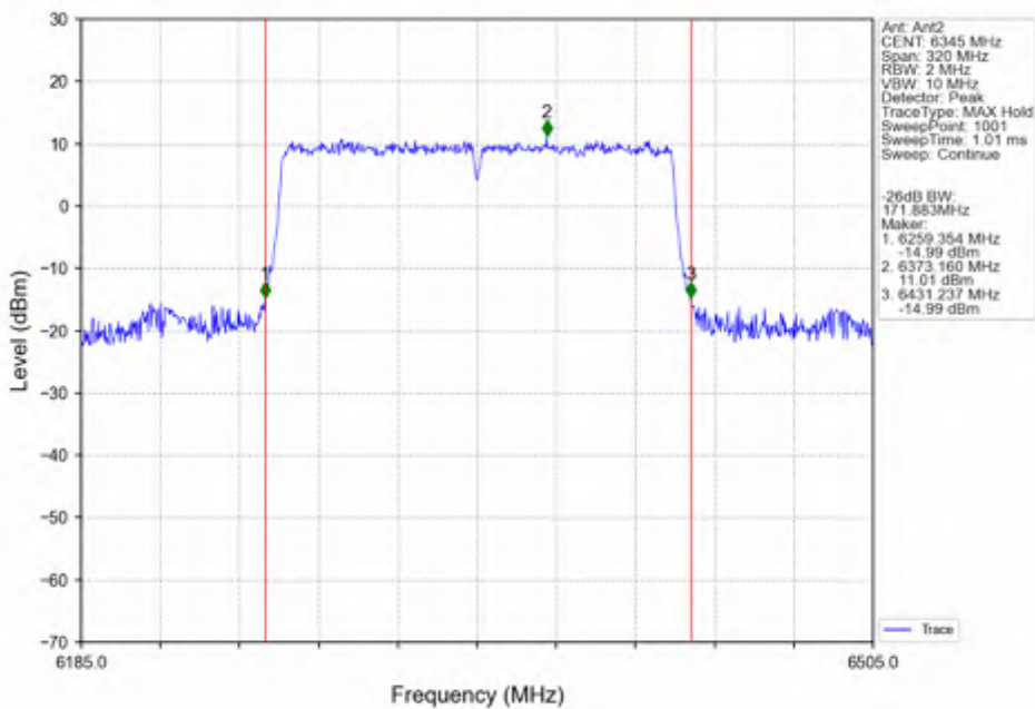
802.11ax(HEW160)_HCH_6345MHz_SU / Ant2_NTNV
