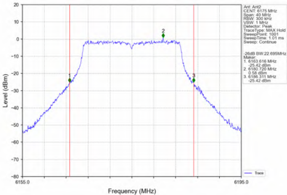
802.11ac(VHT20)_MCH_6175MHz_Ant2_NTNV
