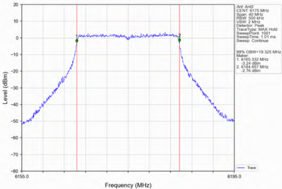
802.11ax(HEW20) MCH_6175MHz_SU / Ant2_NTNV
