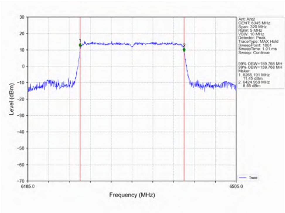
802.11ax(HEW160)_HCH_6345MHz_SU / Ant2_NTNV
