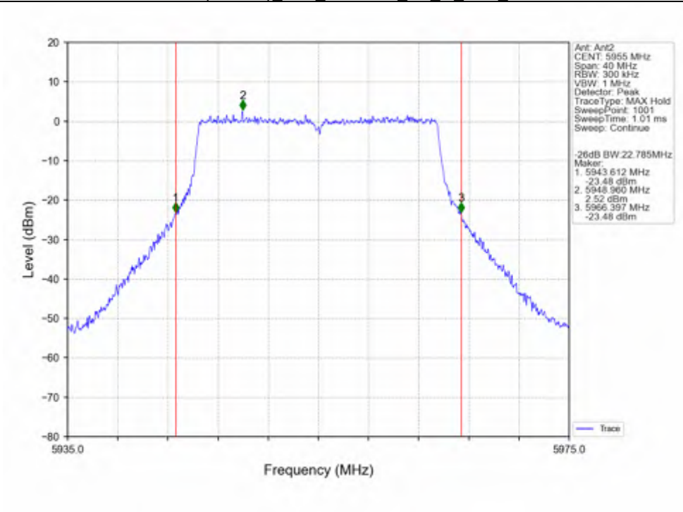
802.11ax(HEW20)_LCH_5955MHz_SU / Ant2_NTNV
