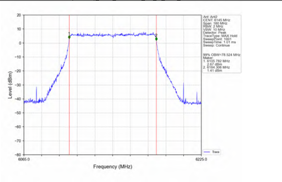
802.11ax(HEW80) MCH_6145MHz_SU / Ant2_NTNV
