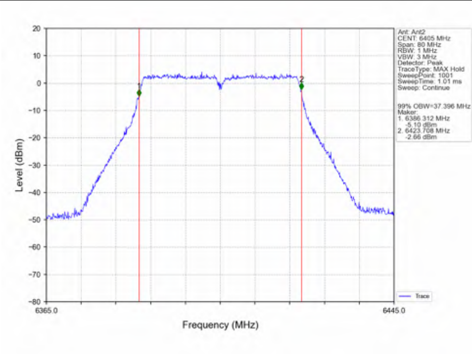
802.11ac(VHT40)_HCH_6405MHz_Ant2_NTNV
