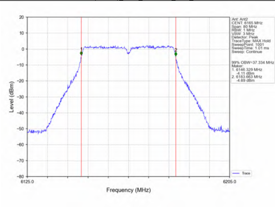
802.11ac(VHT40)_MCH_6165MHz_Ant2_NTNV
