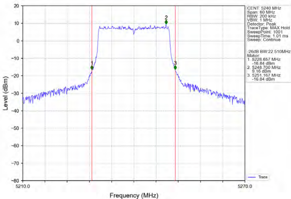
802.11ax(HEW20)_HCH_5240MHz_SU_/_Ant2_NTNV
