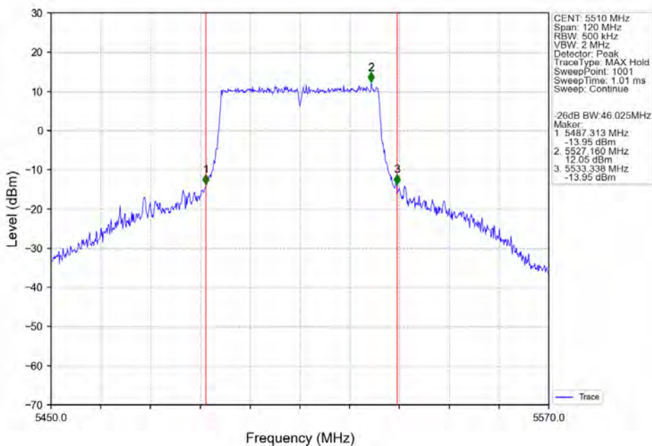
802.11ax(HEW40)_LCH_5510MHz_SU_/_Ant2_NTNV
