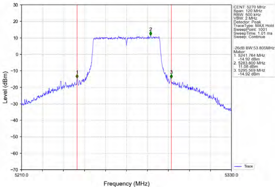
802.11ax(HEW40)_LCH_5270MHz_SU_/_Ant2_NTNV
