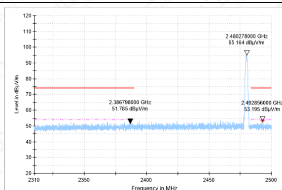
Bandedge-2DH5-CH78-PK
