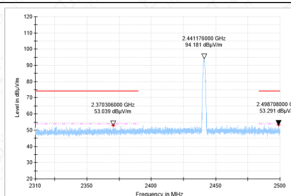
Bandedge-2DH5-CH39-PK
