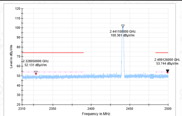
Bandedge-3DH5-CH39-PK
