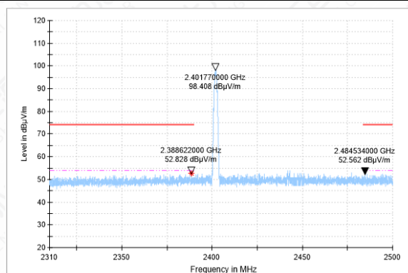
Bandedge-2DH5-CH0-PK
