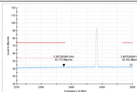
Bandedge-2DH5-CH39-AV
