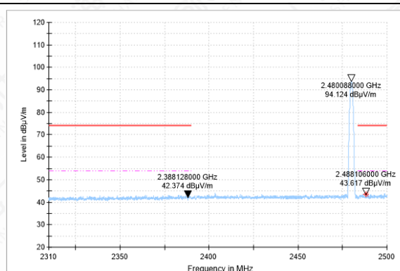
Bandedge-2DH5-CH78-AV
