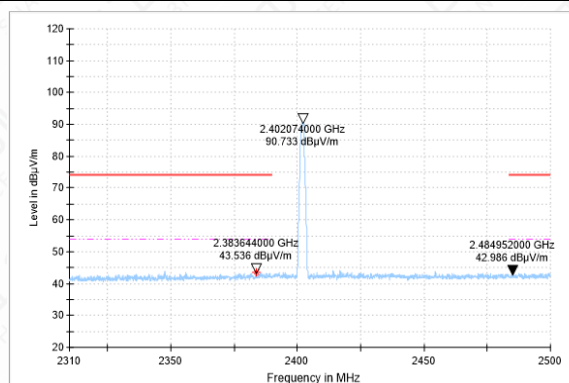
Bandedge-2DH5-CH0-AV
