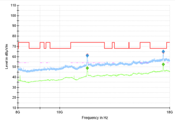
RSE-11N(40M)-CH159-8GHz-18GHz
