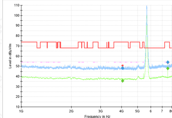
RSE-11N(40M)-CH134-1GHz-8GHz
