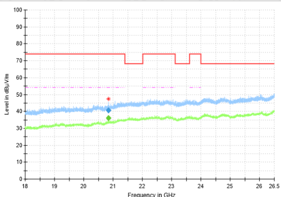
RSE-11AC(80M)-CH42-18GHz-26.5GHz
