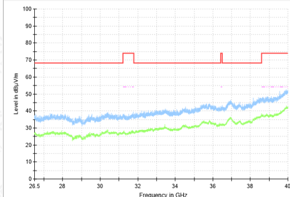
RSE-11N(40M)-CH62-26.5GHz-40GHz
