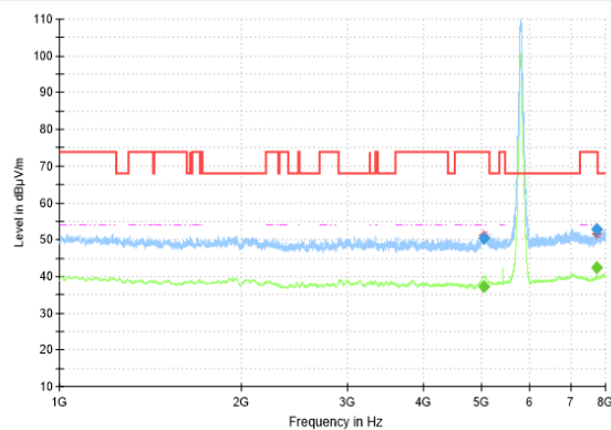
RSE-11N(40M)-CH159-1GHz-8GHz
