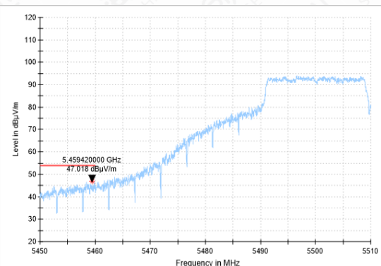
Bandedge-11N(20M)-CH100-AV
