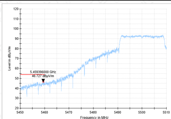
Bandedge-11AC(20M)-CH100-AV
