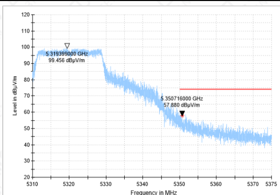
Bandedge-11AC(20M)-CH64-PK
