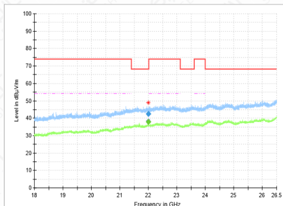
RSE-11A-CH100-18GHz-26.5GHz
