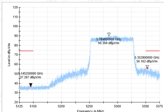
Bandedge-11AC(80M)-CH58-PK
