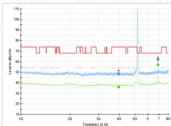
RSE-11N-CH36-1GHz-8GHz
