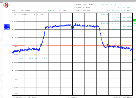
11AC40SISO-Ant1-5550
