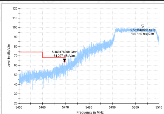
Bandedge-11AC(20M)-CH100-PK
