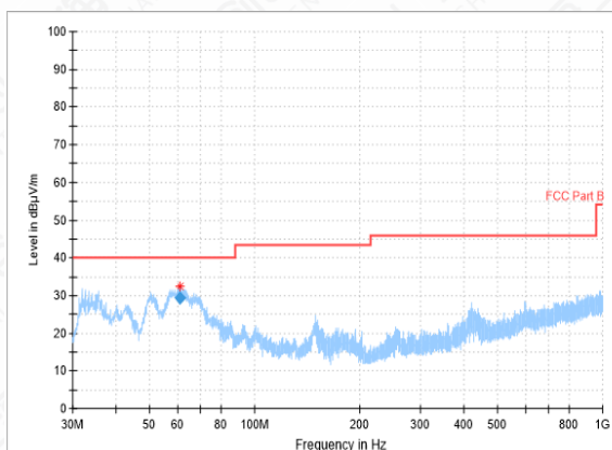
RSE-11N-CH36-30MHz-1GHz
