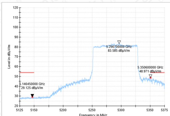
Bandedge-11AC(80M)-CH58-AV
