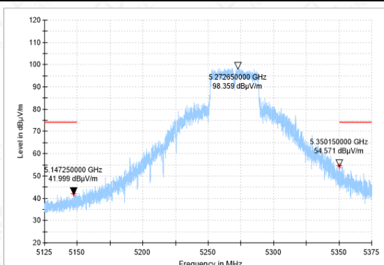
Bandedge-11N(40M)-CH54-PK
