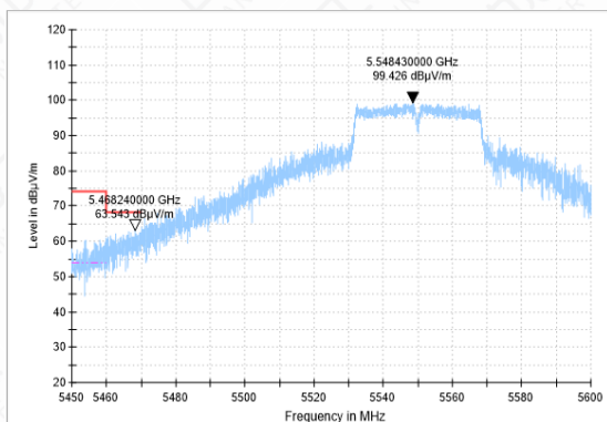
BANDEDGE-11AC(40M)-CH110-PK
