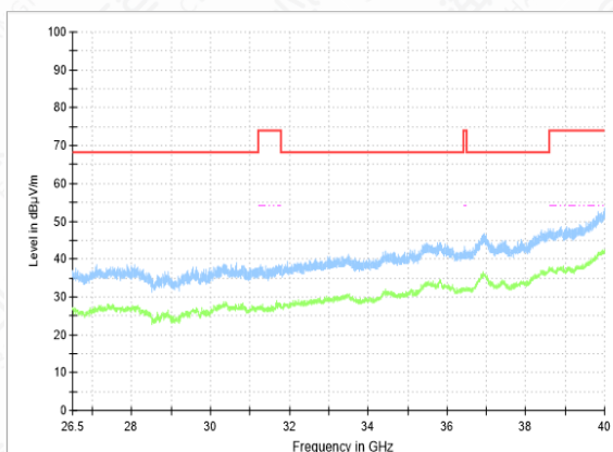
RSE-11N-CH36-26.5GHz-40GHz
