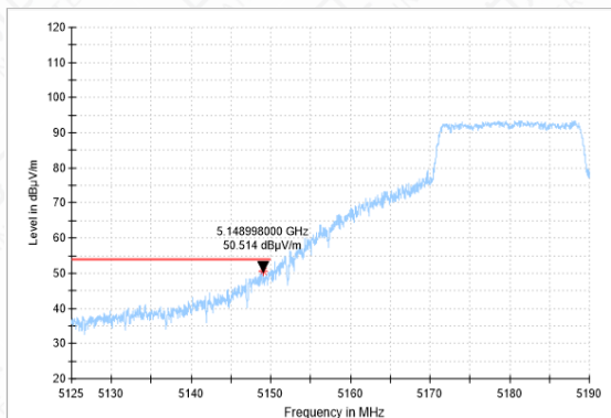
Bandedge-11N(20M)-CH36-AV
