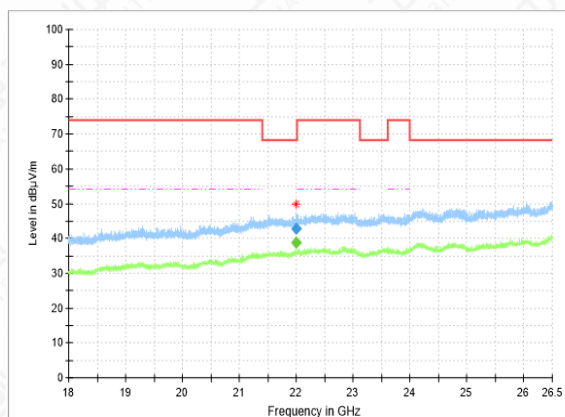
RSE-11N-CH100-18GHz-26.5GHz
