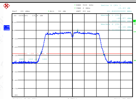
11AC40SISO-Ant1-5310
