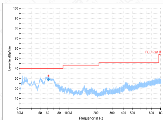
RSE-11N-CH64-30MHz-1GHz
