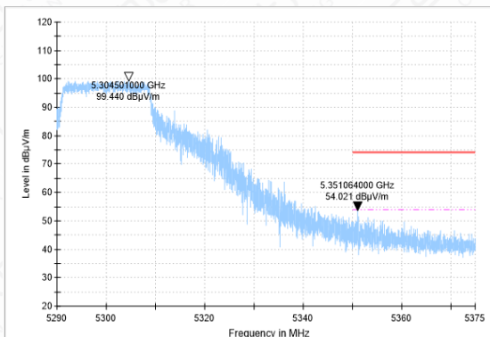
Bandedge-11AC(20M)-CH64-PK
