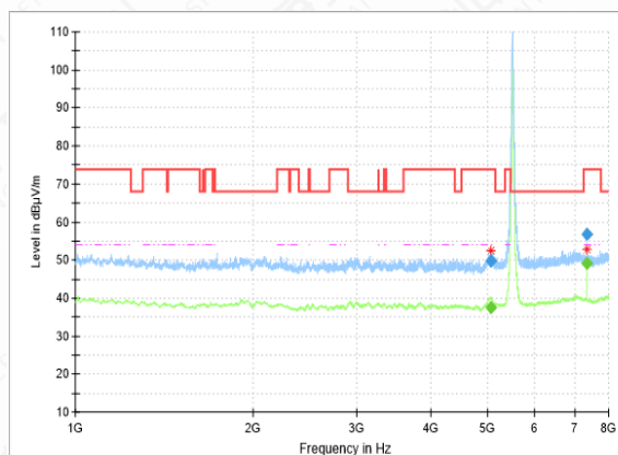
RSE-11N-CH100-1GHz-8GHz
