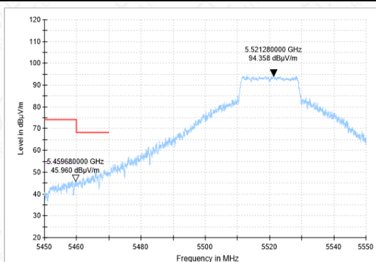
Bandedge-11AC(20M)-CH104-AV
