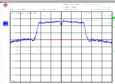
11AC40SISO-Ant1-5230
