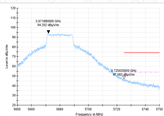
Bandedge-11N(20M)-CH136-AV
