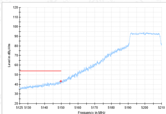
Bandedge-11N(20M)-CH40-AV
