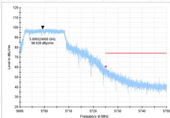
Bandedge-11A-CH140-PK
