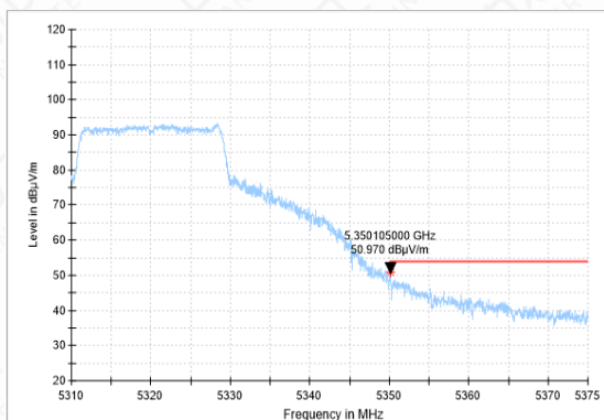
Bandedge-11N(20M)-CH64-AV
