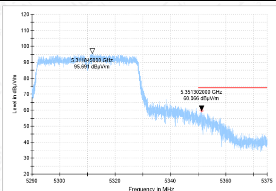
Bandedge-11N(40M)-CH62-PK
