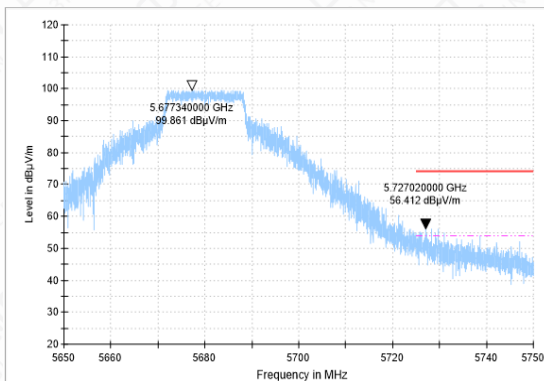
Bandedge-11A-CH136-PK
