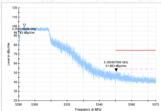
Bandedge-11N(20M)-CH60-PK
