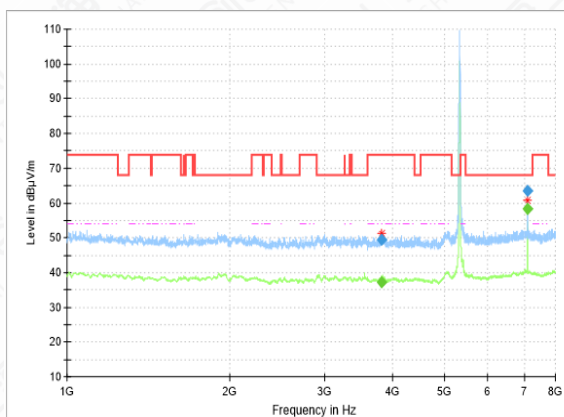
RSE-11N-CH64-1GHz-8GHz
