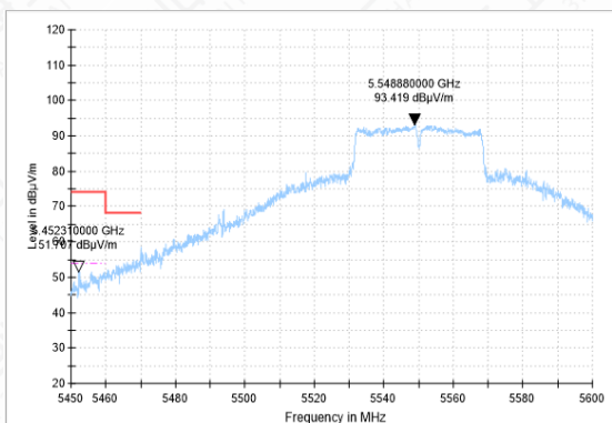
BANDEDGE-11AC(40M)-CH110-AV
