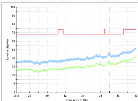
RSE-11A-CH100-26.5GHz-40GHz
