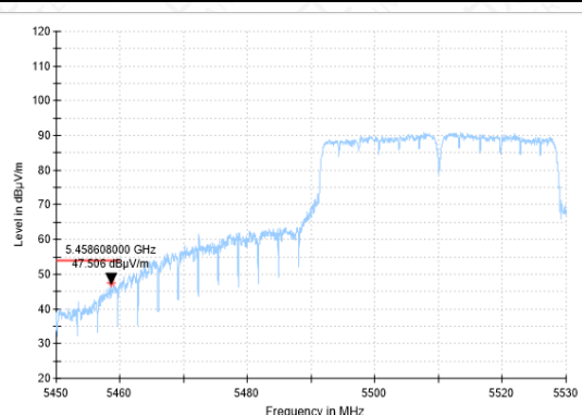
Bandedge-11N(40M)-CH102-AV
