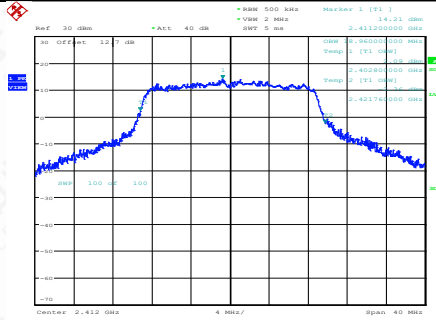
11N20SISO-Ant1-2412
