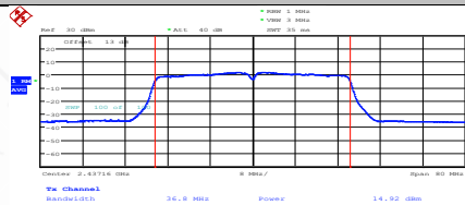
11N40SISO-Ant1-2437-PASS
