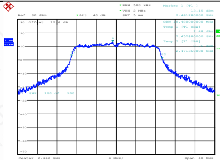
11N20SISO-Ant1-2462
