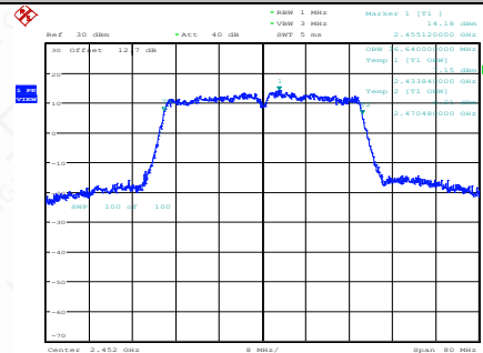
11N40SISO-Ant1-2452
