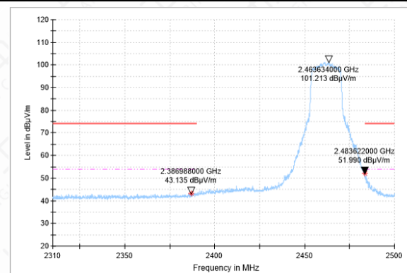
BANDEDGE-11G-CH11-AV
