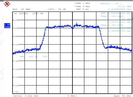
11N40SISO-Ant1-2422
