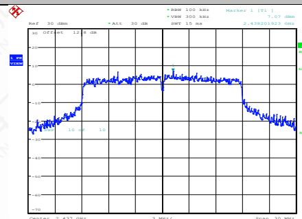
11N20SISO-Ant1-2437-0~Reference-PASS
