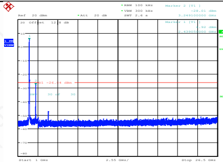
11N40SISO-Ant1-2437-1000~26500-PASS
