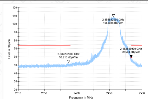
BANDEGE-11N(20M)-CH10-PK
