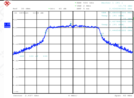
11N20SISO-Ant1-2437
