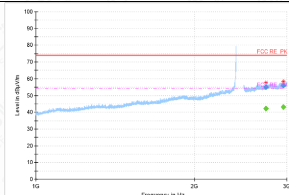
RSE-11B-CH1-1GHz-3GHz
