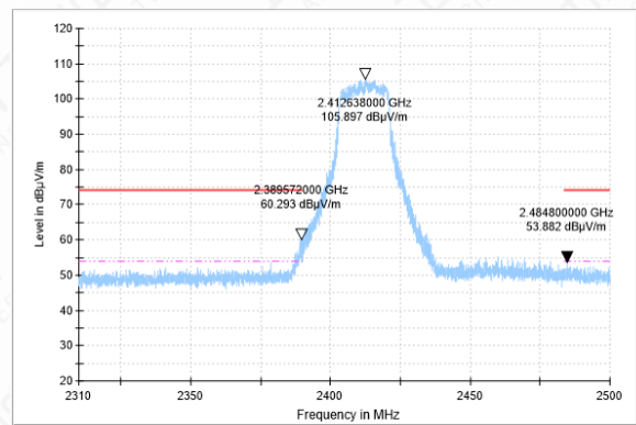
BANDEGE-11N(20M)-CH1-PK
