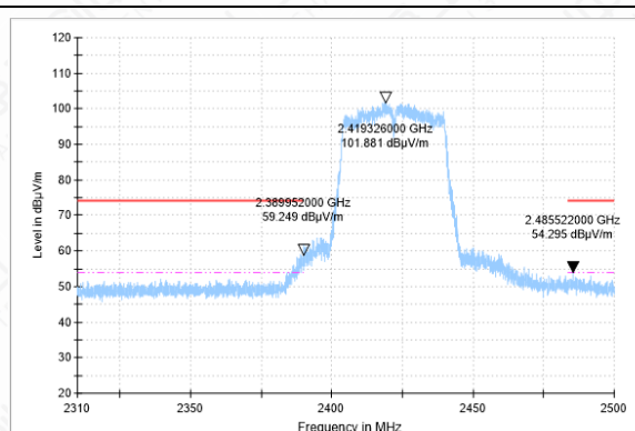
BANEDGE-11N(40M)-CH3-PK
