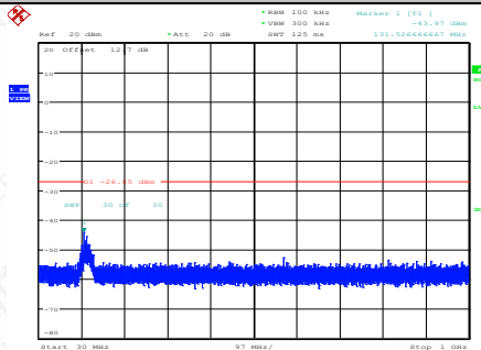
11N40SISO-Ant1-2452-30~1000-PASS
