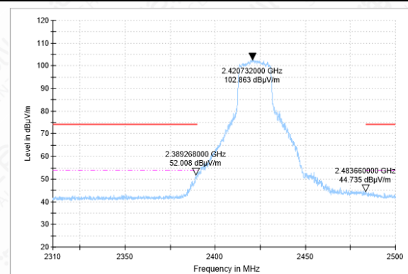
BANDEDGE-11G-CH3-AV
