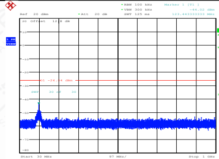
11N40SISO-Ant1-2437-30~1000-PASS
