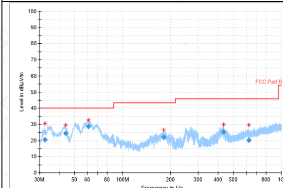
RSE-11B-CH1-30MHz-1GHz
