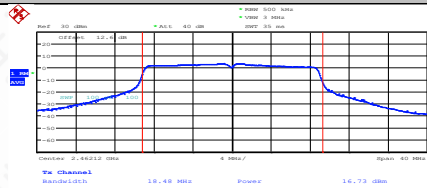
11N20SISO-Ant1-2462-PASS
