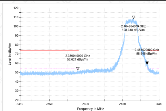
BANDEDGE-11G-CH11-PK
