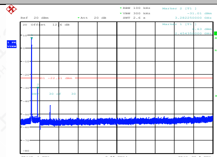
11G-Ant1-2462-1000~26500-PASS
