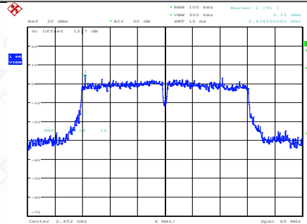
11N40SISO-Ant1-2452-0~Reference-PASS
