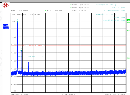
11G-Ant1-2437-1000~26500-PASS
