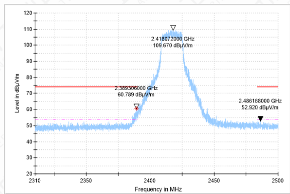
BANDEDGE-11G-CH2-PK
