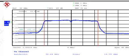
11N40SISO-Ant1-2452-PASS
