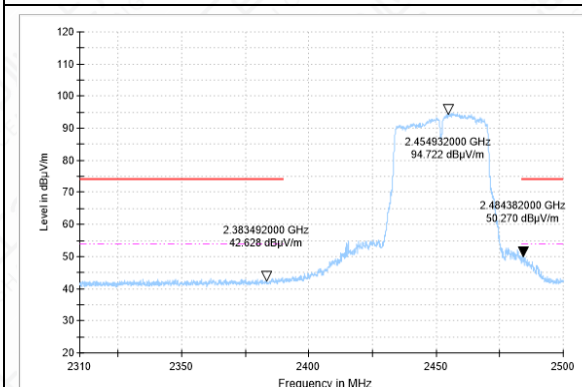
BANEDGE-11N(40M)-CH9-AV
