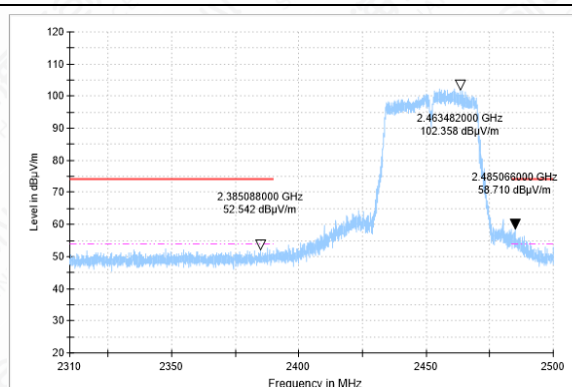
BANEDGE-11N(40M)-CH9-PK
