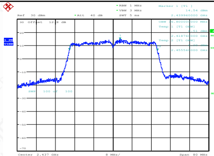
11N40SISO-Ant1-2437
