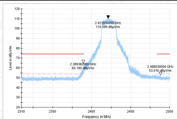
BANDEDGE-11G-CH3-PK
