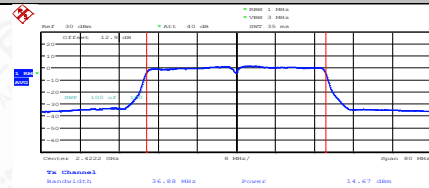
11N40SISO-Ant1-2422-PASS
