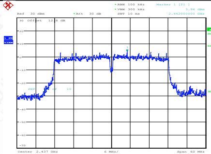
11N40SISO-Ant1-2437-0~Reference-PASS
