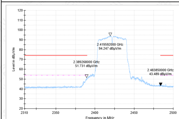
BANEDGE-11N(40M)-CH3-AV
