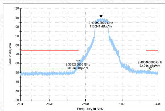
BANDEGE-11N(20M)-CH3-PK
