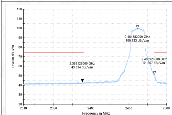
BANEDGE-11N(20M)-CH11-AV
