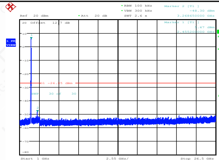
11N40SISO-Ant1-2452-1000~26500-PASS
