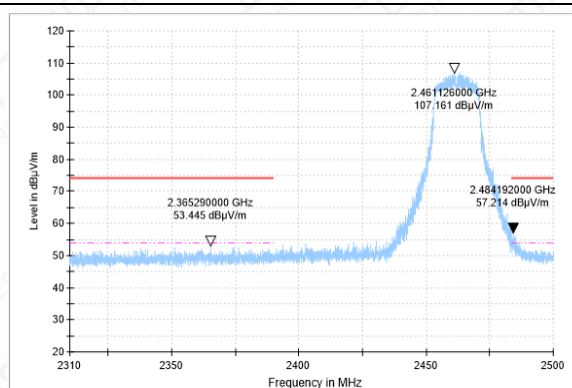
BANEDGE-11N(20M)-CH11-PK
