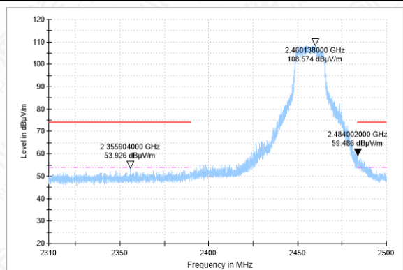
BANDEDGE-11G-CH10-PK
