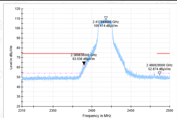
BANDEGE-11N(20M)-CH2-PK
