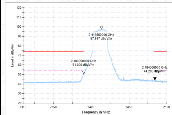
BANDEGE-11N(20M)-CH1-AV
