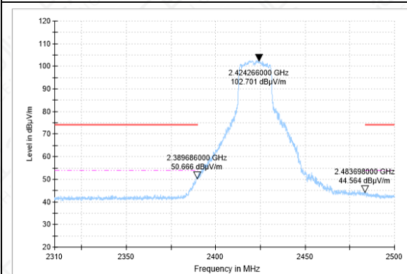
BANDEGE-11N(20M)-CH3-AV
