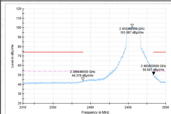
BANDEGE-11N(20M)-CH10-AV
