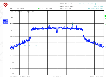
11G-Ant1-2462-0~Reference-PASS
