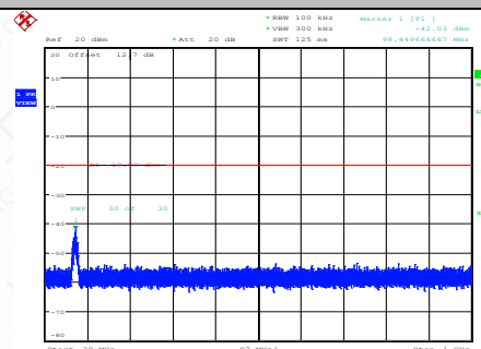
11N20SISO-Ant1-2412-30~1000-PASS
