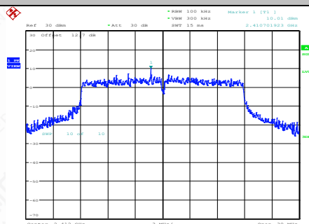
11N20SISO-Ant1-2412-0~Reference-PASS
