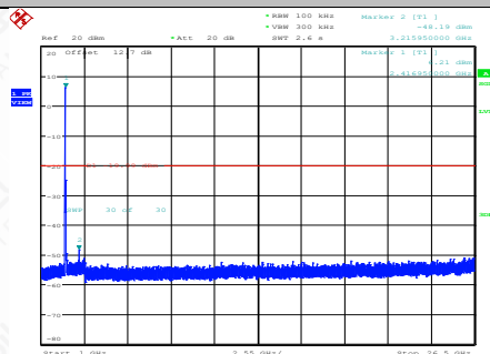
11N20SISO-Ant1-2412-1000~26500-PASS
