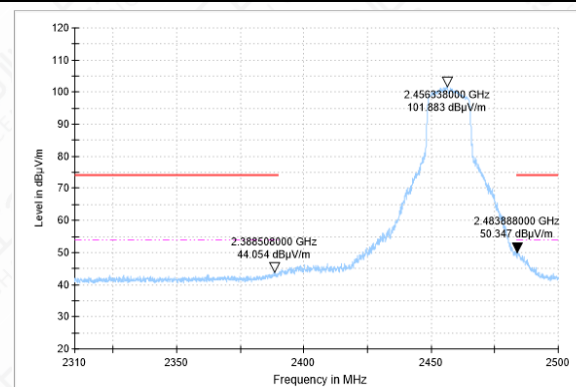
BANDEDGE-11G-CH10-AV
