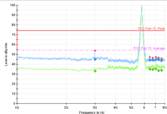
Radiated Spurious Emission (802.11ac-VHT80, ch155, 1GHz-8GHz)
