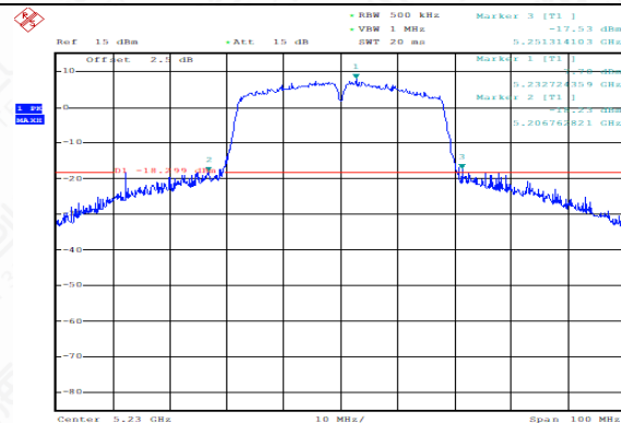
Occupied 26dB Bandwidth (MHz) (802.11ac-VHT40, 5230MHz)
