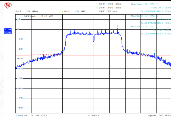
Occupied 26dB Bandwidth (MHz) (802.11ac-VHT20, 5240MHz)
