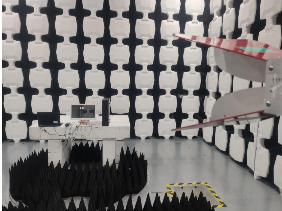
Description: Back view of Radiated Emission Test Setup (Above 1G)
