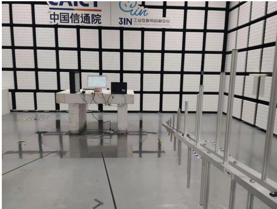
Description: Back view of Radiated Emission Test Setup (Below 1G)
