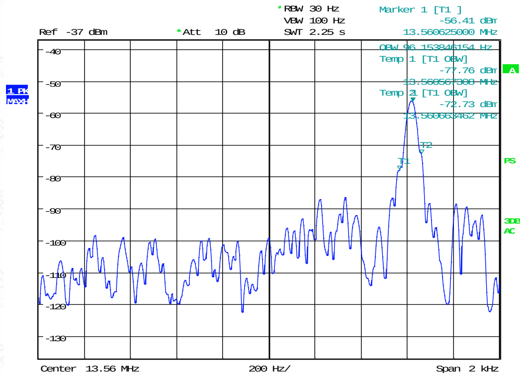
Figure A.4-1 Mode 1 Occupied bandwidth
