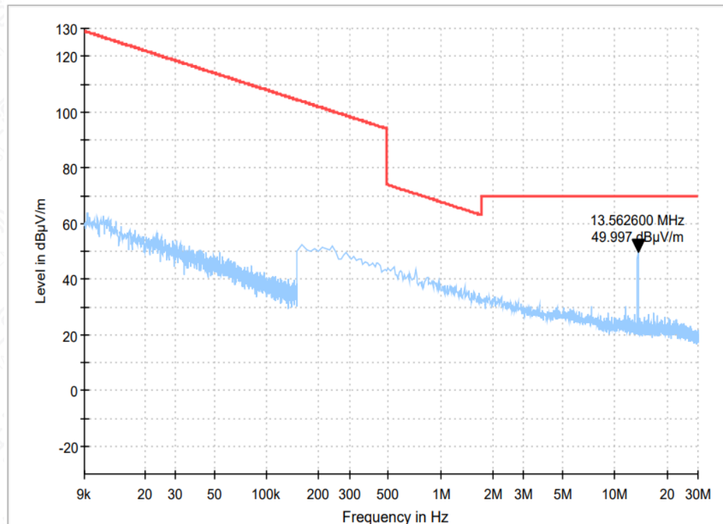
Figure A.3.2-1 Mode 1 Electric Field Radiated Emissions (Below 30MHz)
