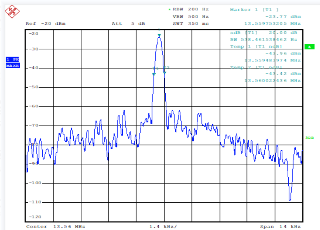
Figure A.1-1 Mode 1 20dB Bandwidth
