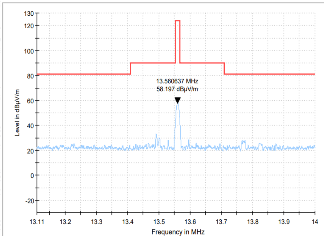
Figure A.3.1-1 Mode 1 Electric Field Strength of Fundamental Emissions
