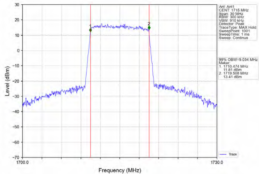
Band66_10MHz_16QAM_LCH_1715MHz_RB_50_0_NTNV
