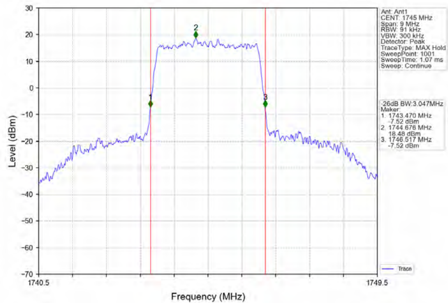
Band66_3MHz_QPSK_MCH_1745MHz_RB_15_0_NTNV
