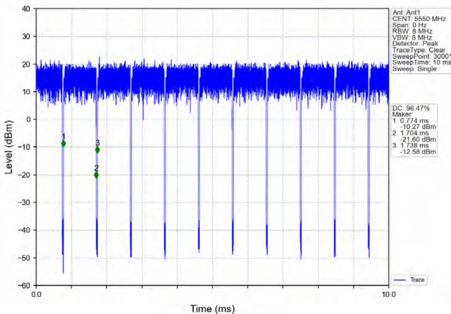
802.11n(HT40)_MCH_5550MHz_Ant1_NTNV
