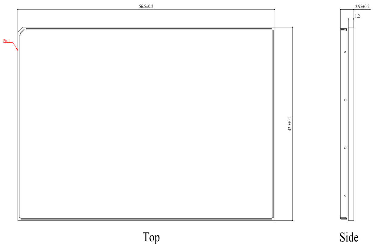
Figure 37: Module Top and Side Dimensions
