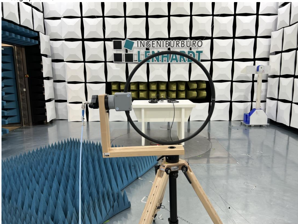
Photograph 4: : EUT A + AE 1 + AE 2 + AE 3+ AE 6. Close view.
