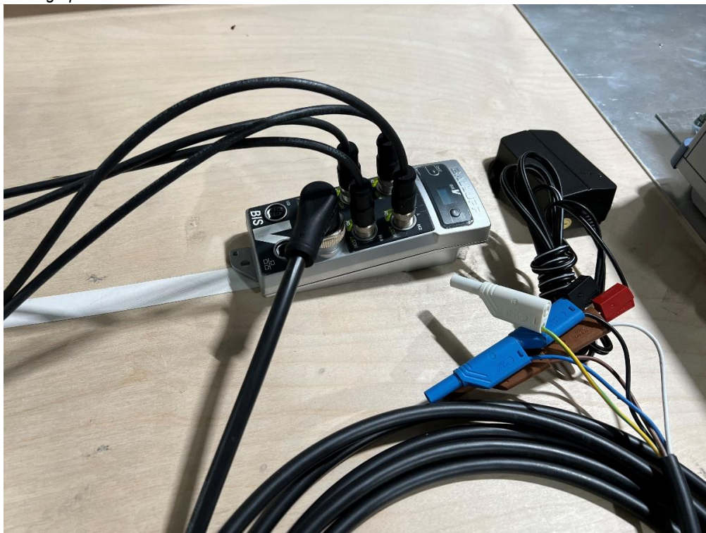
Photograph 10: EUT A + AE 1 + AE 2 + AE 3+ AE 6. Close view.
