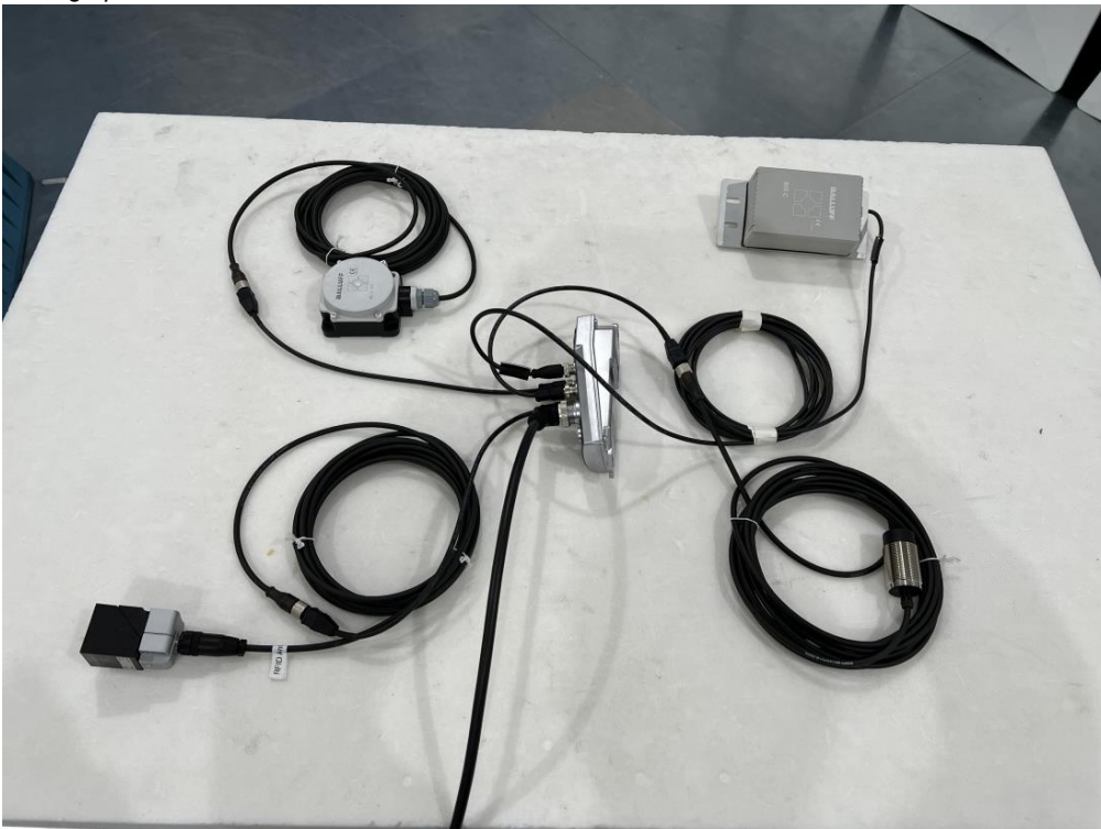
Photograph 2: EUT A + AE 4 + AE 5 + AE 7 + AE 8. Close view.
