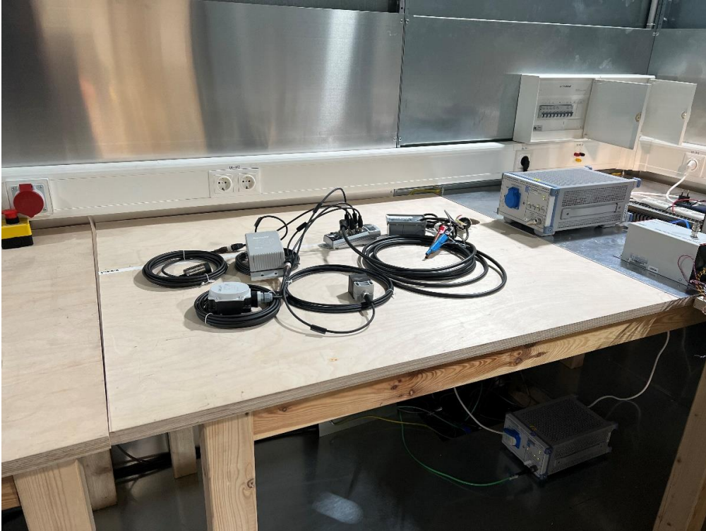
Photograph 7: EUT A + AE 4 + AE 5 + AE 7 + AE 8. Overall view.
