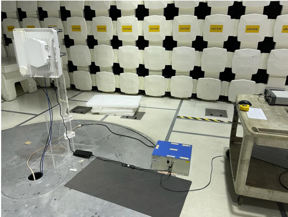
AC Mains Line Conducted Emissions
