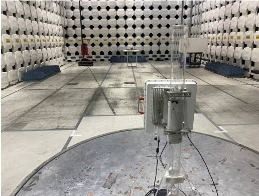
9 kHz-30 MHz Test Setup
