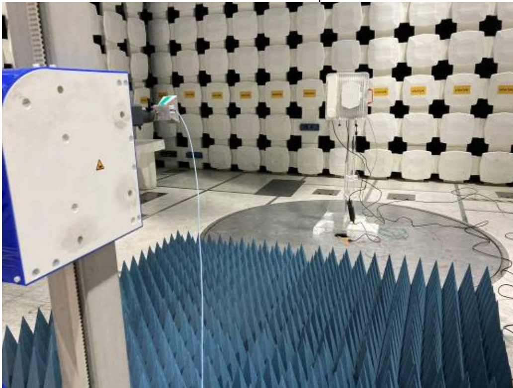
18-40 GHz Test Setup
