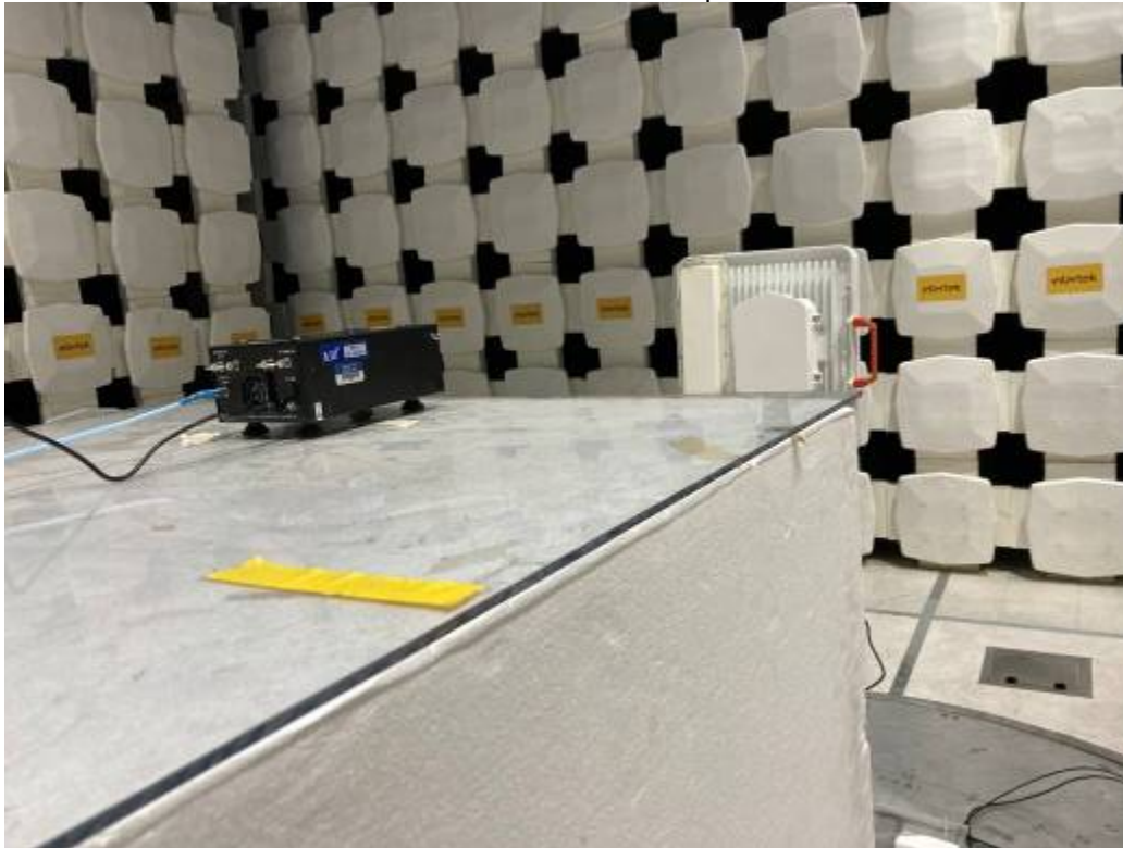
40-100 GHz Test Setup
