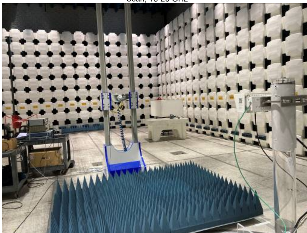
Scan, 18-26 GHz
