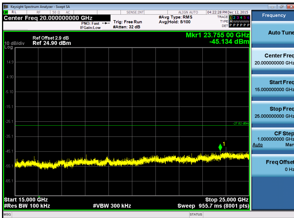
(Plot 4.6.1 C6: Channel 39: 2480MHz @ GFSK)
