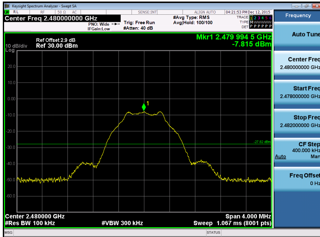
(Plot 4.6.1 C1: Channel 39: 2480MHz @ GFSK)
