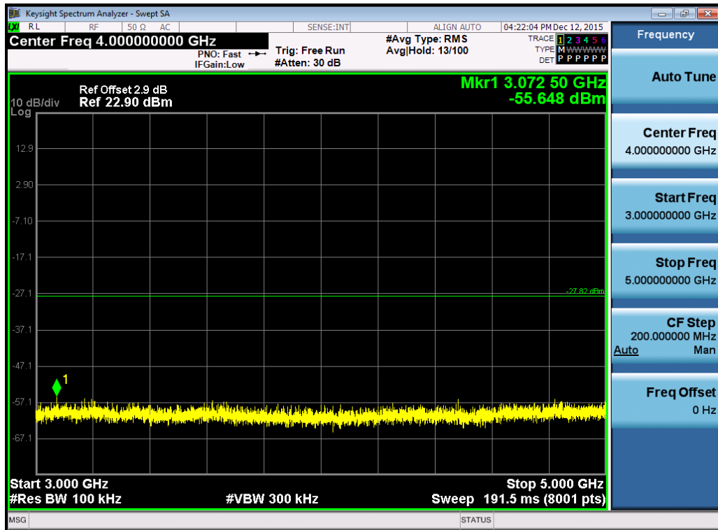
(Plot 4.6.1 C3: Channel 39: 2480MHz @ GFSK)
