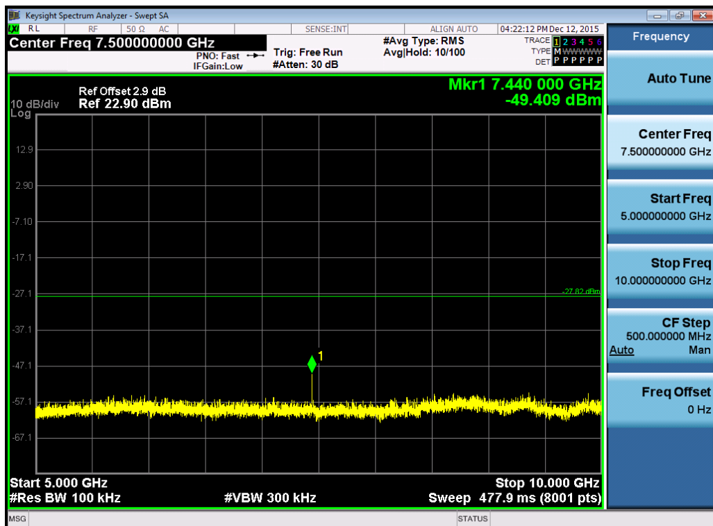
(Plot 4.6.1 C4: Channel 39: 2480MHz @ GFSK)
