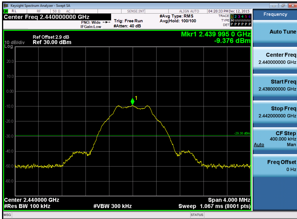
(Plot 4.6.1 B1: Channel 19: 2440MHz @ GFSK)
