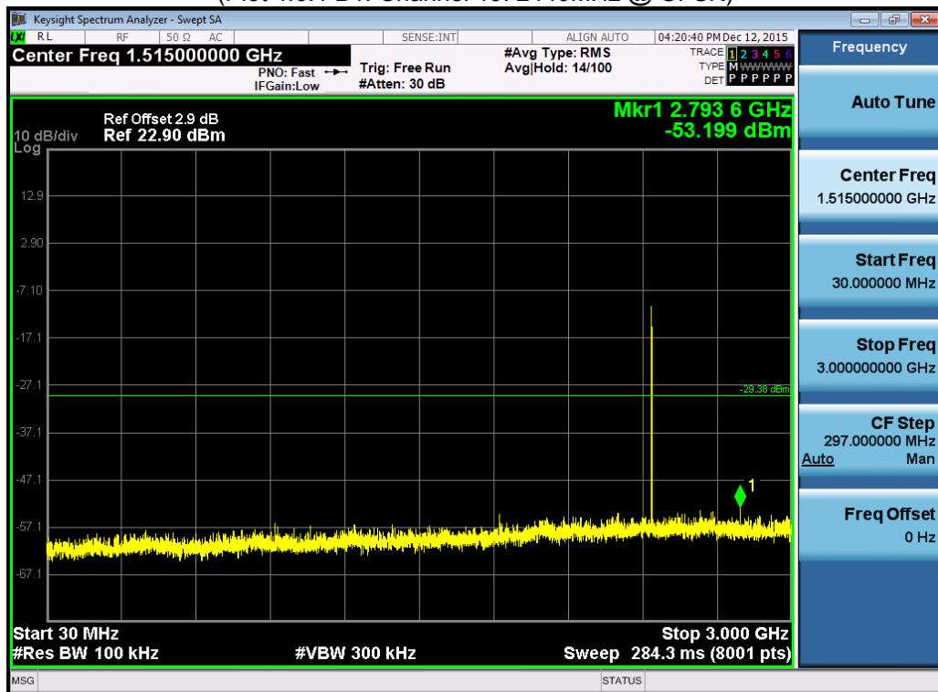
(Plot 4.6.1 B2: Channel 19: 2440MHz @ GFSK)
