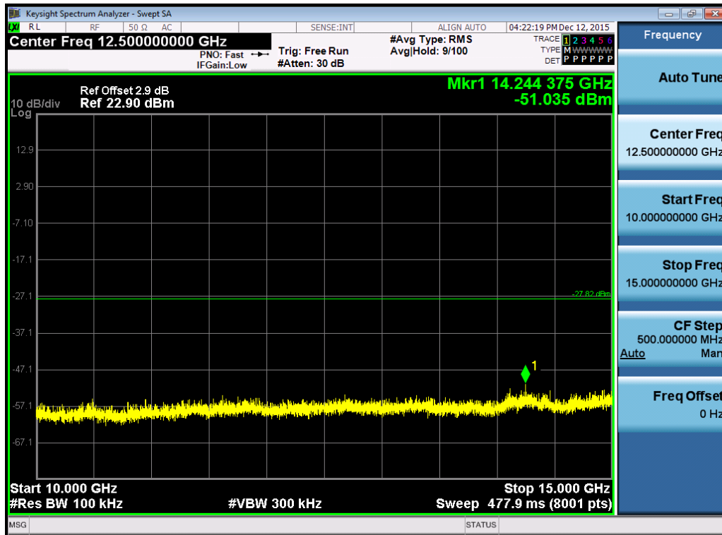
(Plot 4.6.1 C5: Channel 39: 2480MHz @ GFSK)
