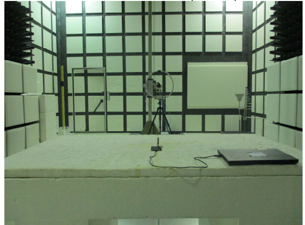
Radiated_MFIM0004 + Helical_Setup
