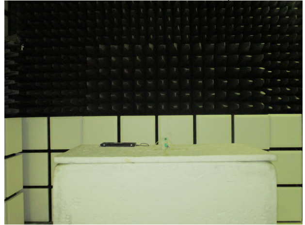
Radiated_MFIM0003 + Helical_Setup
