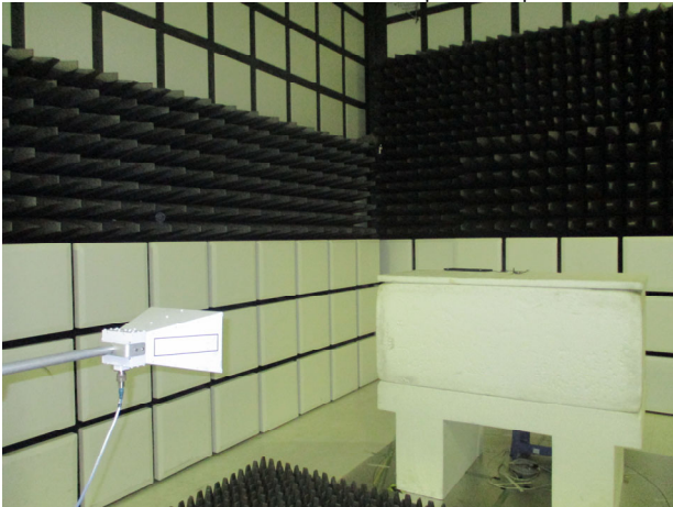
Radiated_MFIM0003 + Monopole_Setup
