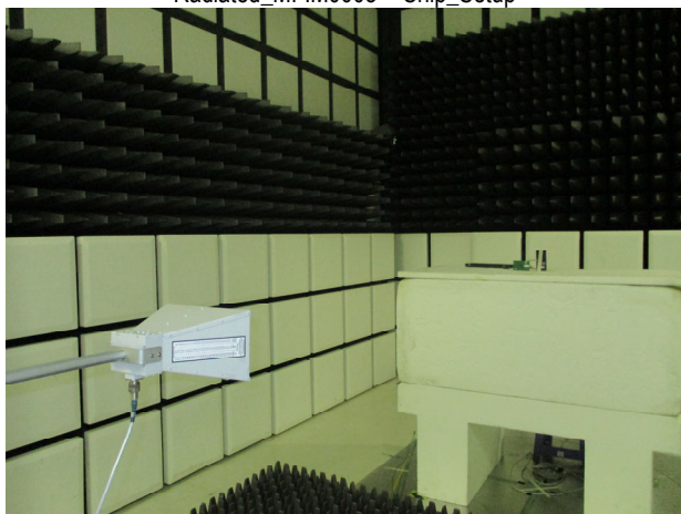
Radiated_MFIM0003 + Chip_Setup
