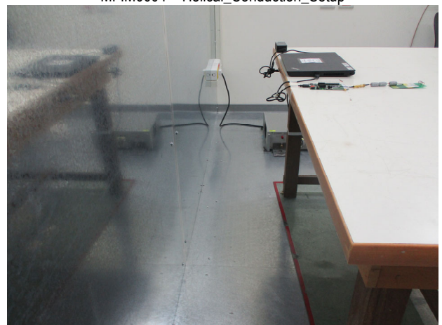
MFIM0004 + Helical_Conduction_Setup
