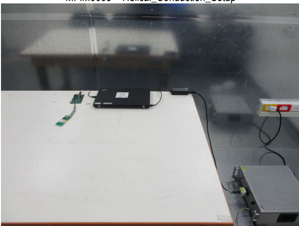
MFIM0003 + Helical_Conduction_Setup
