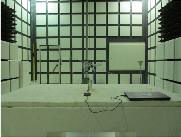
Radiated_MFIM0004 + Helical_Setup
