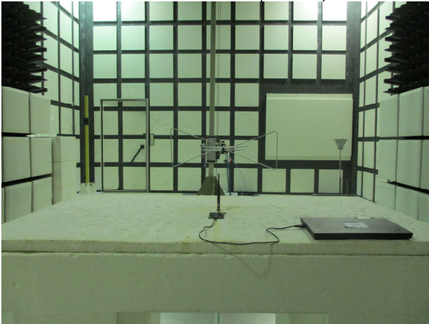
Radiated_MFIM0003 + Dipole_Setup
