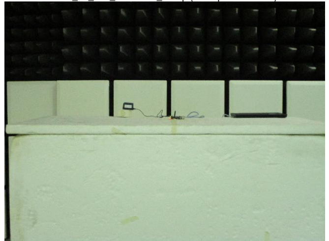
FCC_15_247_Radiated_Setup (Monopole Antenna)
