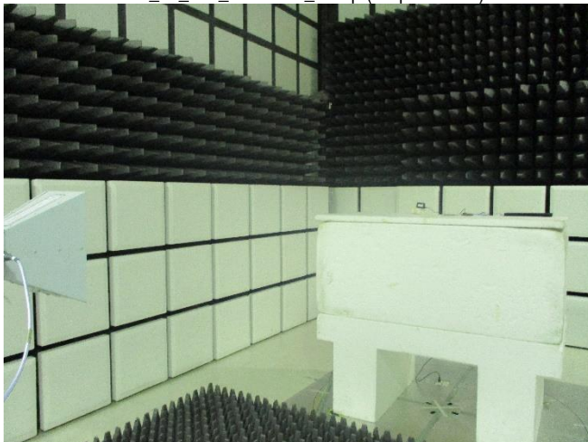
FCC_15_247_Radiated_Setup (Chip Antenna)
