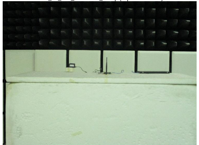
FCC_15_247_Radiated_Setup (Dipole Antenna)
