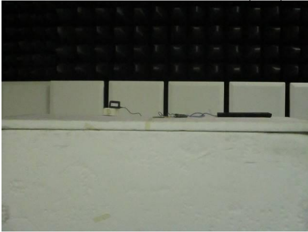
FCC_15_247_902~928MHz_OFDM_Radiated_Chip_Setup
