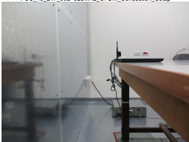
FCC_15_247_902~928MHz_OFDM_Conduction_Setup
