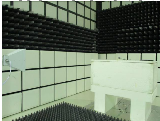
FCC_15_247_902~928MHz_OFDM_Radiated_Monopole_Setup
