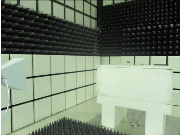
FCC_15_247_902~928MHz_OFDM_Radiated_Chip_Setup
