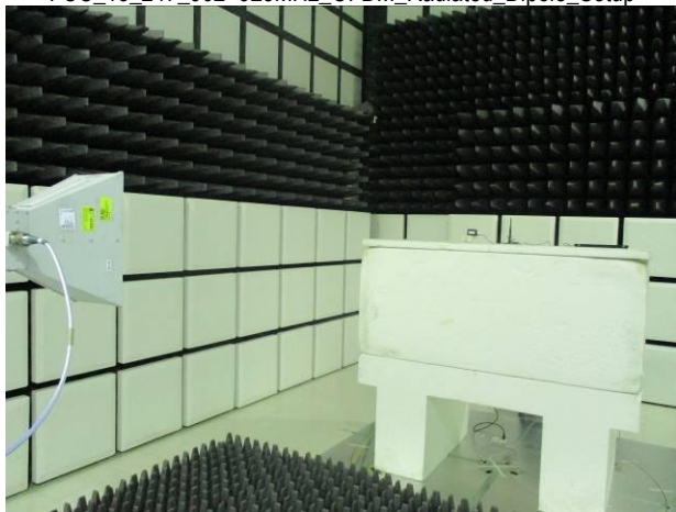
FCC_15_247_902~928MHz_OFDM_Radiated_Dipole_Setup
