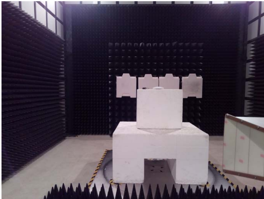
Radiated Emissions (Above 1 GHz, Powered by POE)
