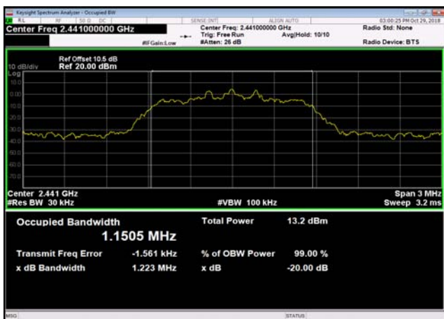
99% Bandwidth: pi/4DQPSK,2441MHz,2DH5
