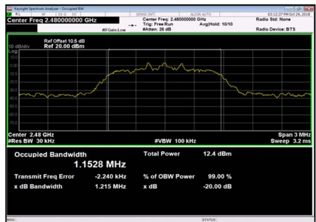
99% Bandwidth: pi/4DQPSK,2480MHz,2DH5
