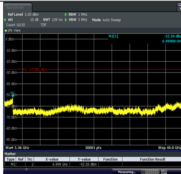
11N40SISO-Ant1-5190-5360~40000-PASS
