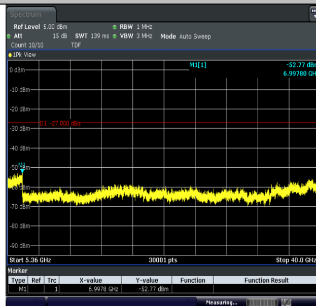
11N20SISO-Ant1-5180-5360~40000-PASS
