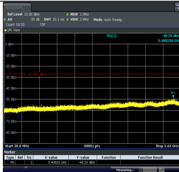
11N40SISO-Ant1-5755-30~5650-PASS
