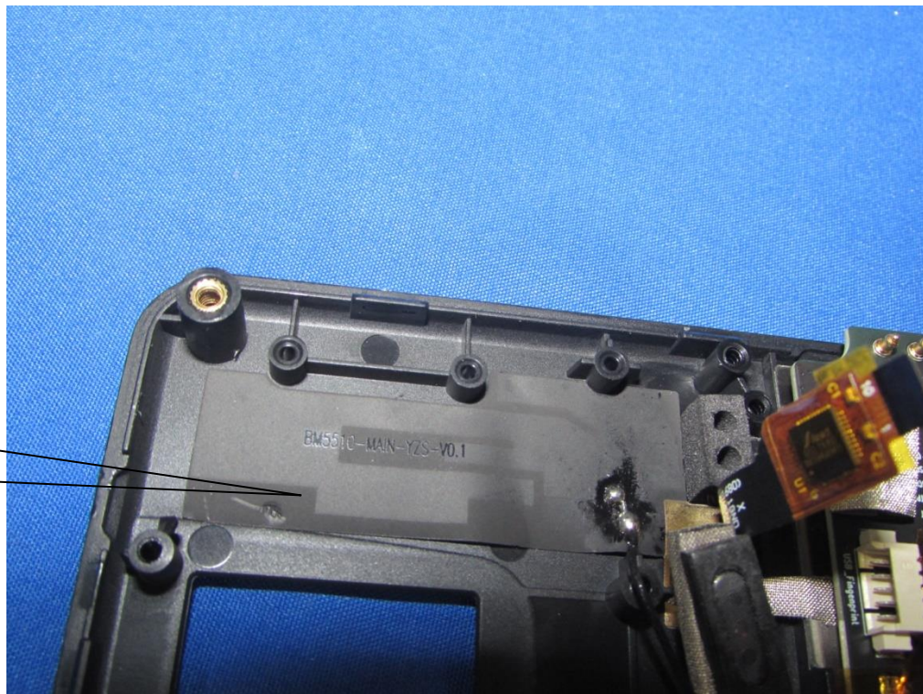
LTE/WCDMA /GSM Main Antenna
