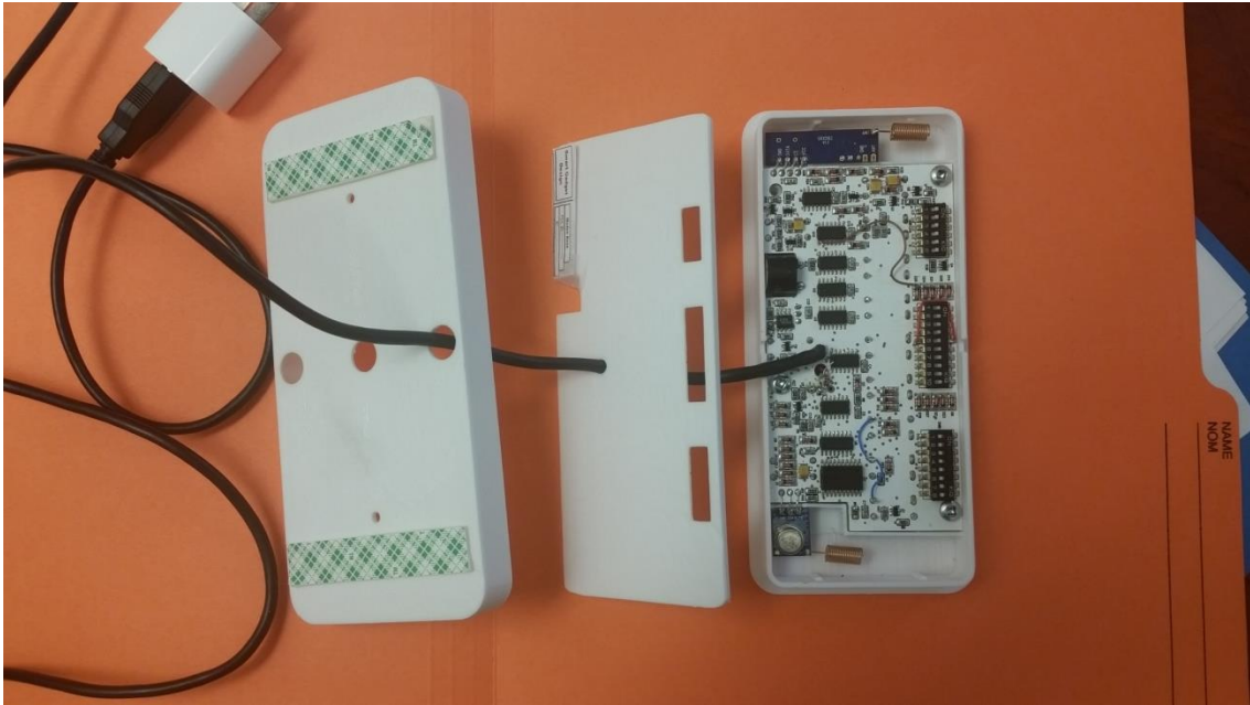
PCB location
