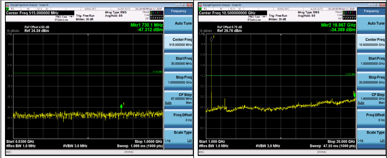
Band4-1.4MHz-64QAM-19957-1RB#0-Range1:30~1000MHz
