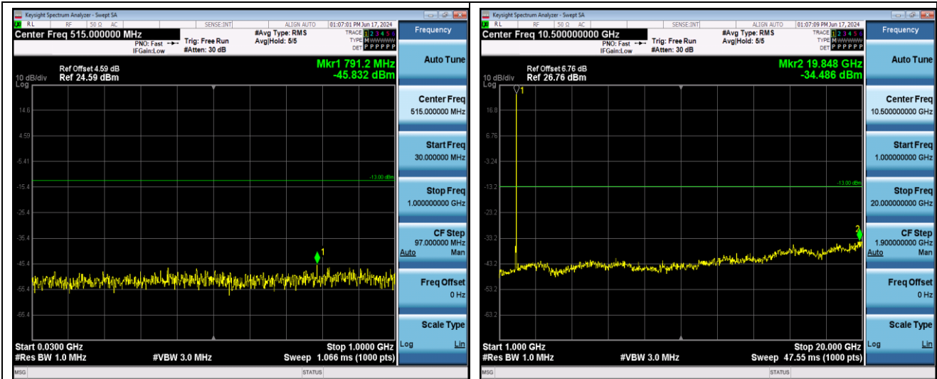
Band4-1.4MHz-QPSK-19957-1RB#0-Range1:30~1000MHz
