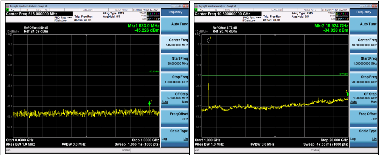
Band2-20MHz-16QAM-18900-1RB#0-Range1:30~1000MHz
