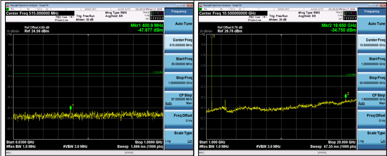
Band4-1.4MHz-QPSK-20175-1RB#0-Range1:30~1000MHz
