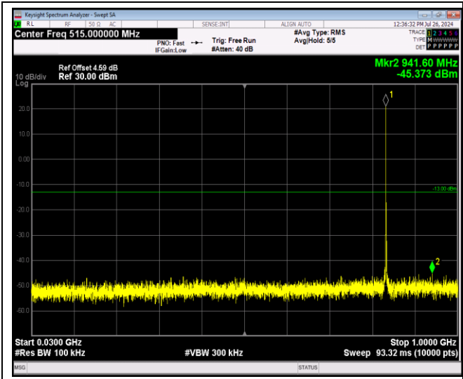
Band5-1.4MHz-QPSK-20643-1RB#0-Range1:30~1000MHz
