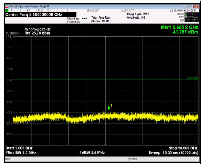
Band5-1.4MHz-QPSK-20643-1RB#0-Range2:1000~10000MHz
