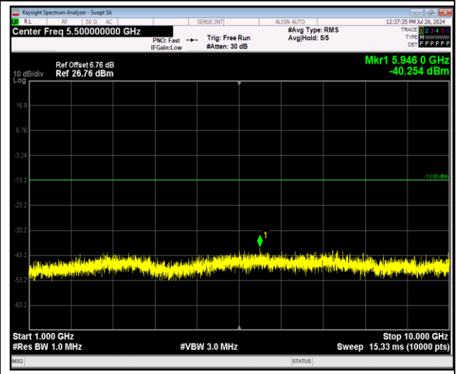
Band5-1.4MHz-16QAM-20407-1RB#0-Range2:1000~10000MHz
