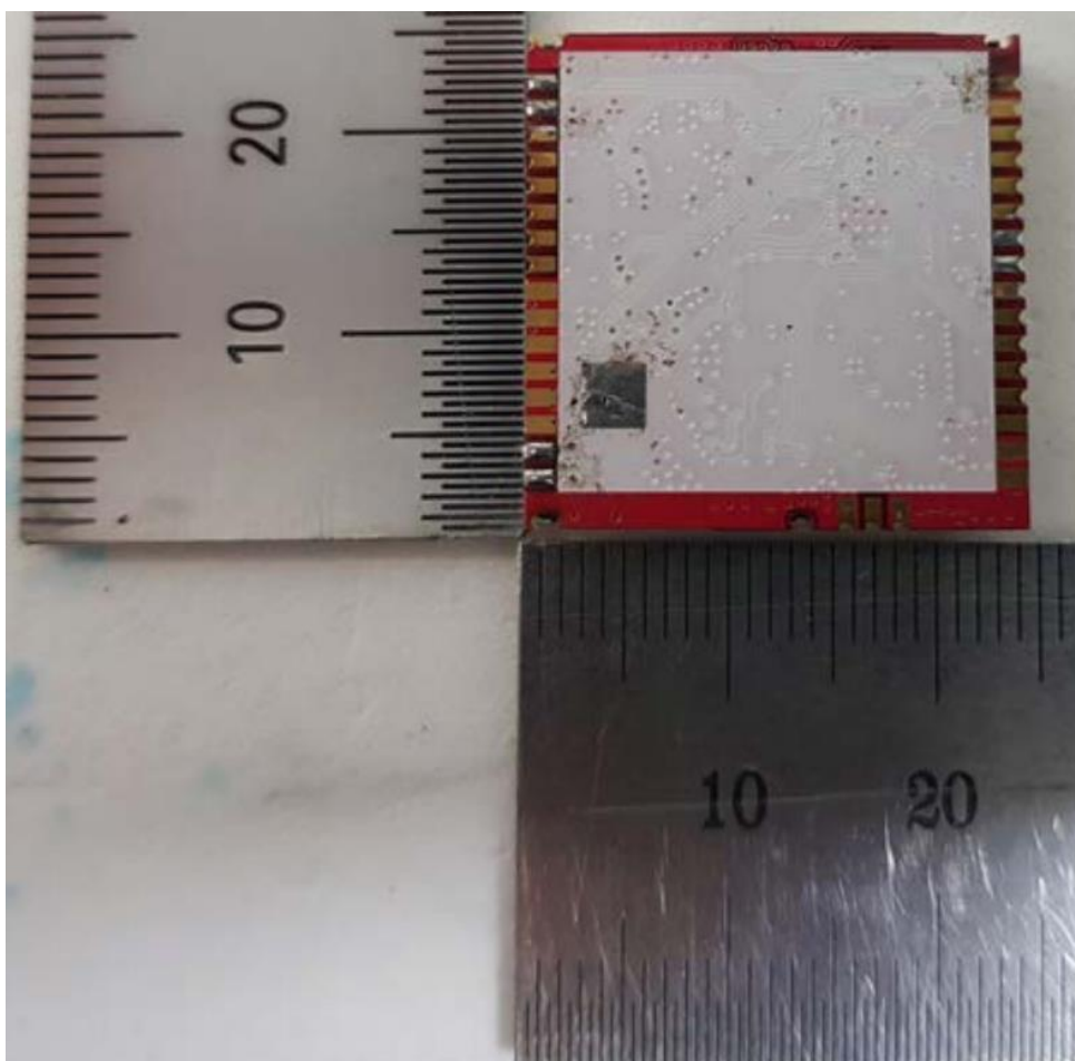
Figure 2 Bottom side
