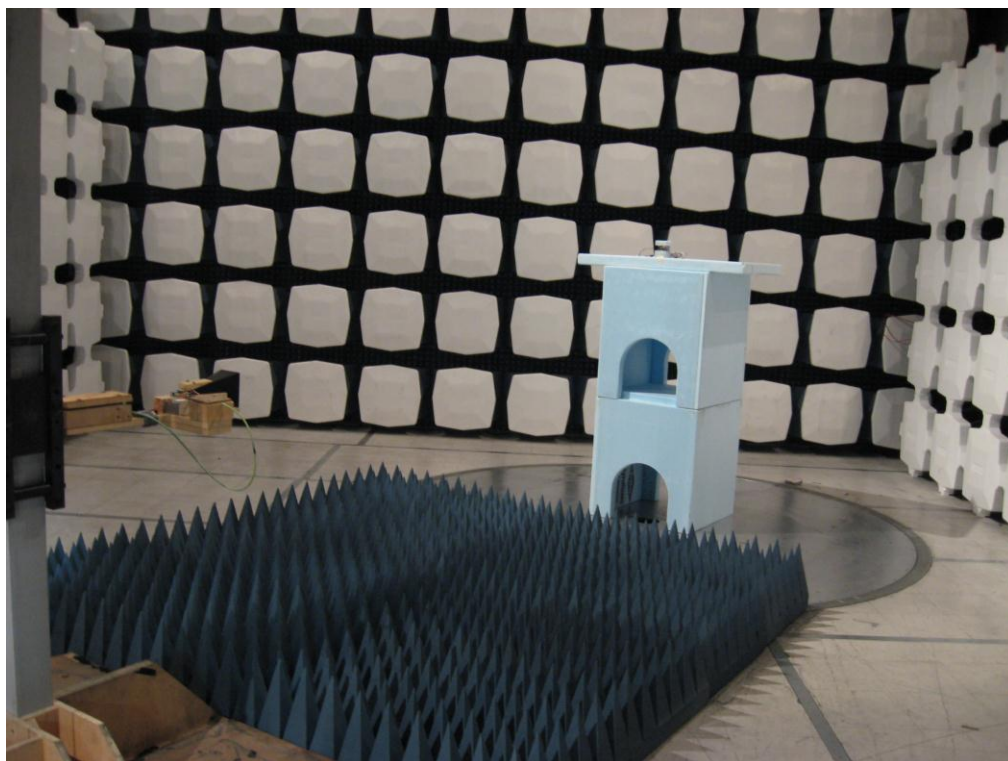
Figure 4: Emissions above 18 GHz
