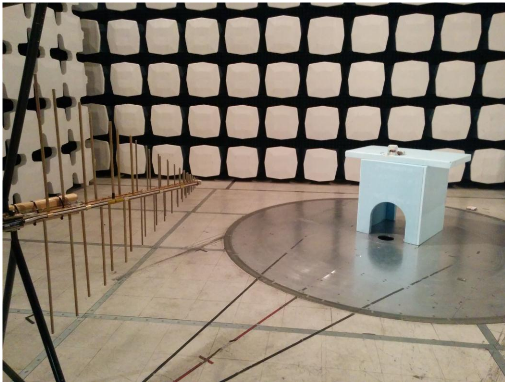
Figure 2: Emissions below 1 GHz
