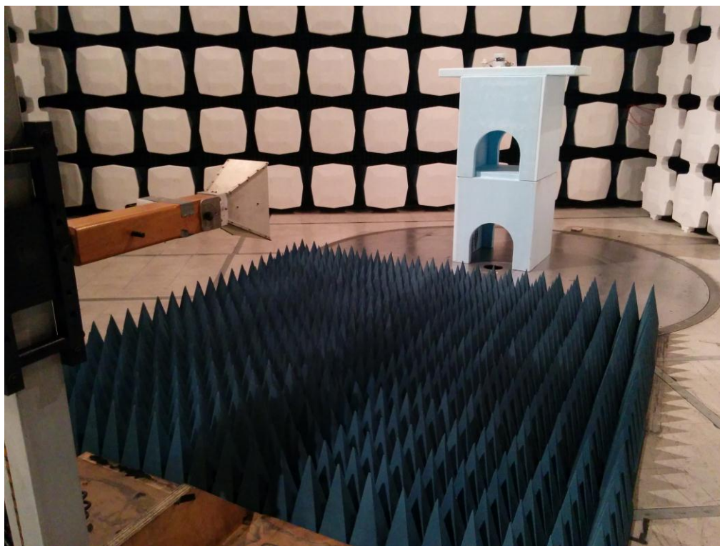
Figure 3: Emissions above 1 GHz
