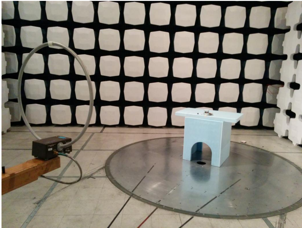
Figure 1: Emissions below 30 MHz
