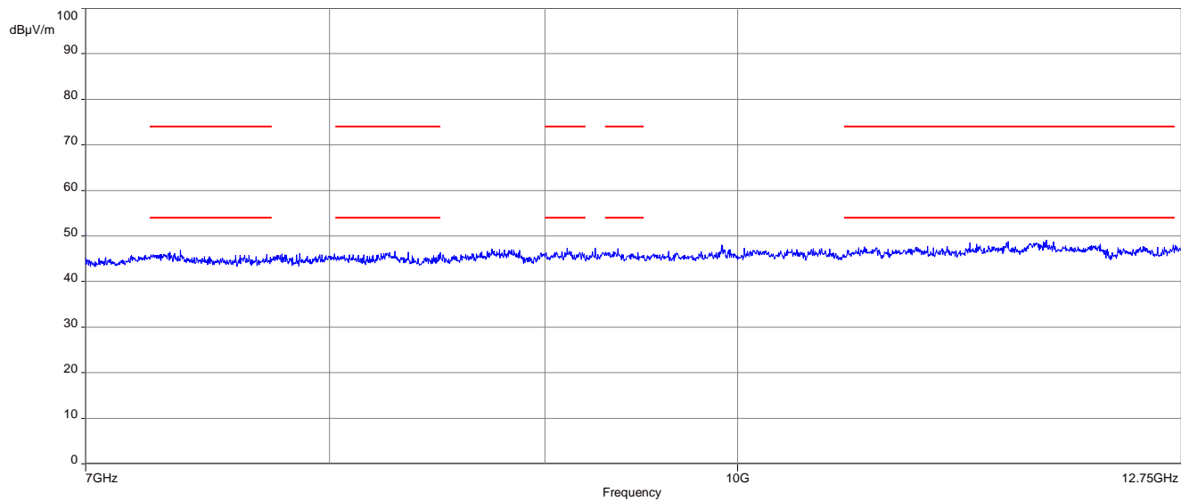
Plot 2: 7 GHz to 12.75 GHz, vertical & horizontal polarization
