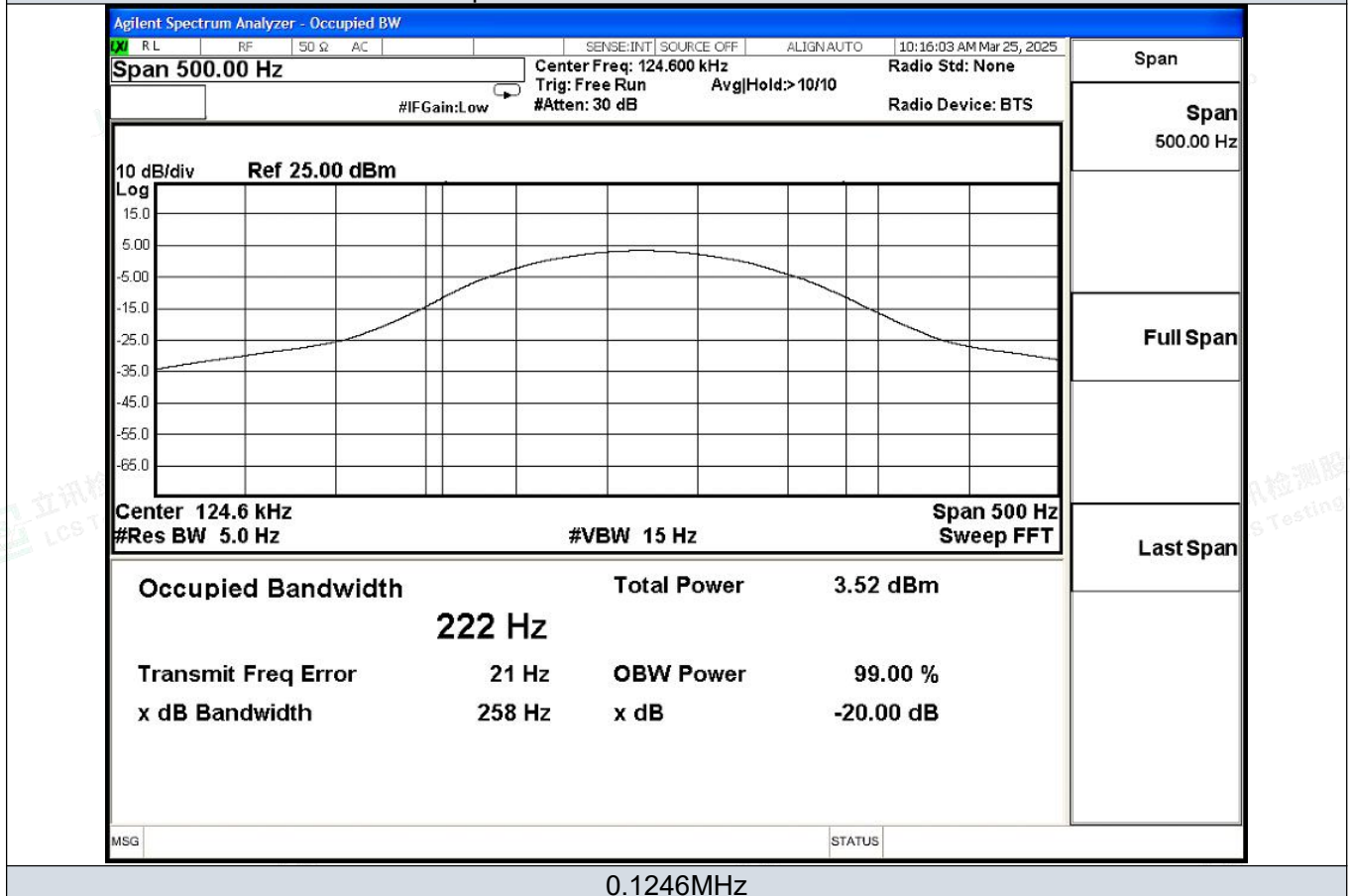
Test plot of 20 dB Bandwidth Measurement
