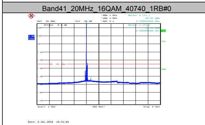
Band41_20MHz_16QAM_40740_1RB#0
