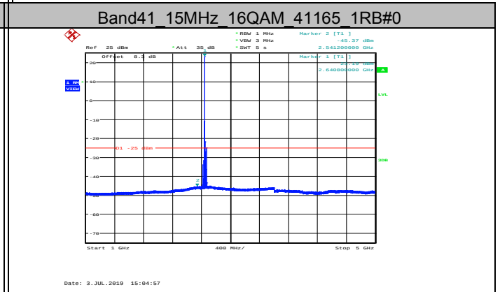
Band41_15MHz_16QAM_41165_1RB#0
