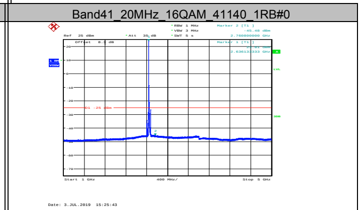
Band41_20MHz_16QAM_41140_1RB#0
