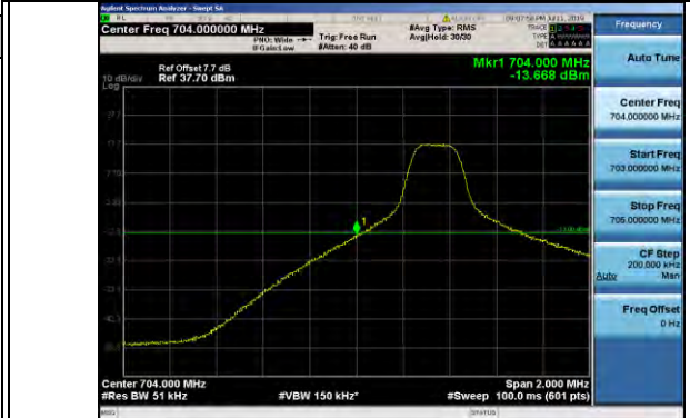
Band17_5MHz_QPSK_23755_25RB#0
