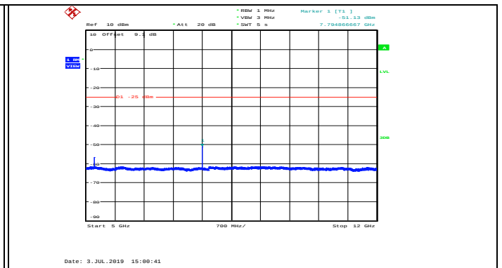
Band41_15MHz_16QAM_40740_1RB#0
