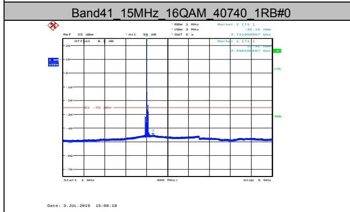
Band41_15MHz_16QAM_40740_1RB#0
