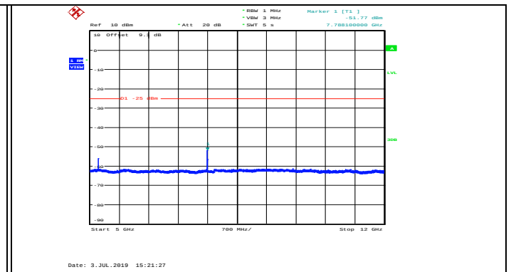
Band41_20MHz_16QAM_40740_1RB#0
