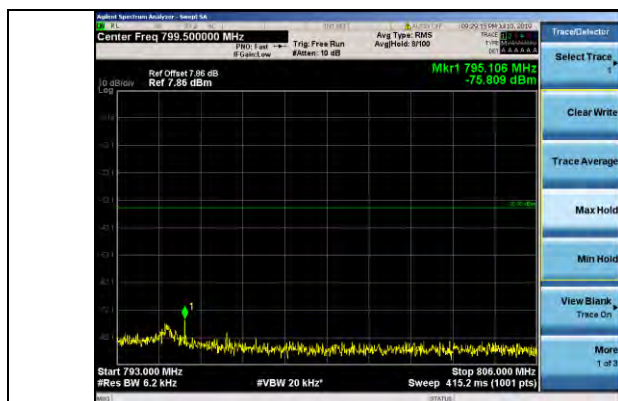
Band13 5MHz 16QAM 23230 1RB#0
