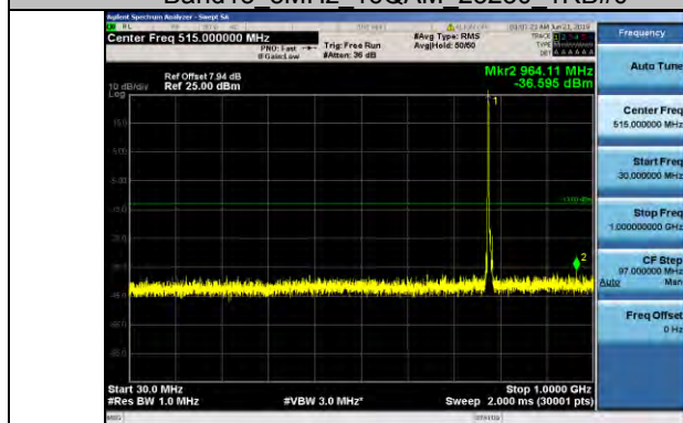
Band13 5MHz 16QAM 23230 1RB#0
