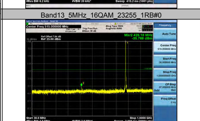
Band13 5MHz 16QAM 23255 1RB#0
